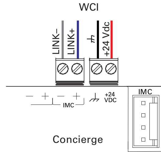
Figure 3. WCI Connection
