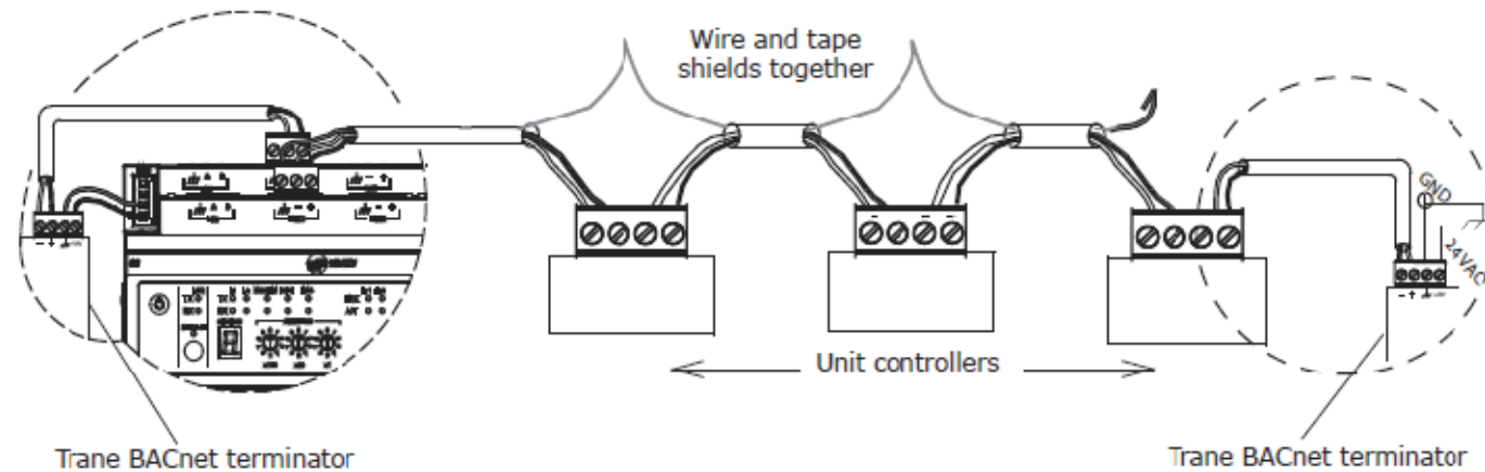
Figure 4. Daisy-chain configuration for BACnet wiring
