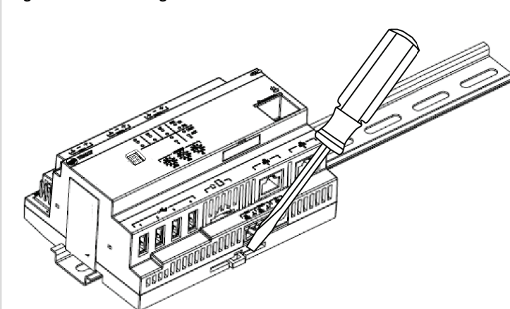
6 Figure 2. Removing the SC+ Controller
