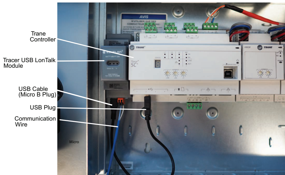
Figure 1. Tracer USB LonTalk module installed with a Trane Controller
