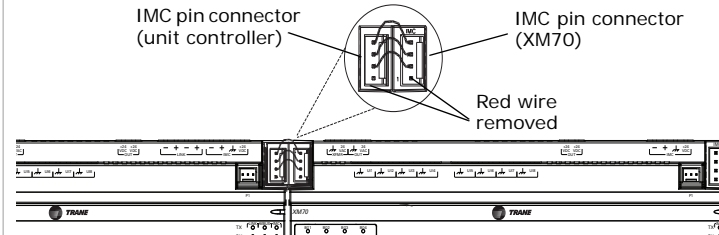
Figure 4. IMC connections from an XM70 to a UC400/UC600/XM70
