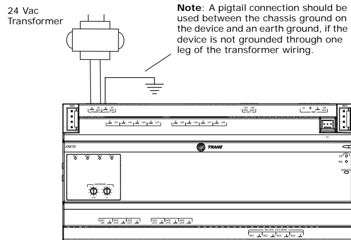
Figure 3. Wiring AC power to the Controller
