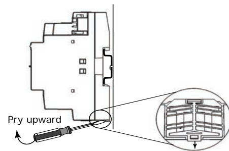
Figure 2. Removing the expansion module
