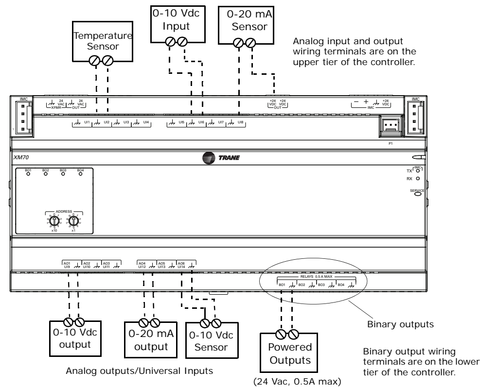
Figure 4. XM70 input and output wiring examples
