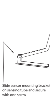
Figure 3. Sensor Mounting Bracket
