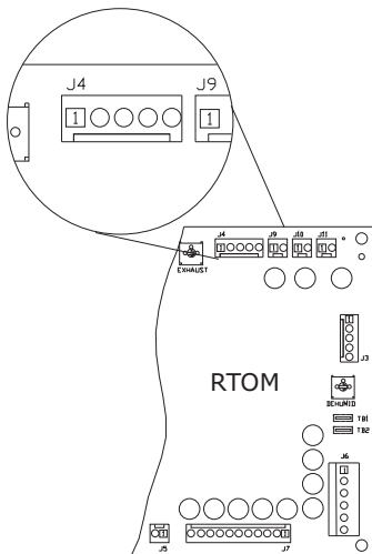
Figure 5. Options Board
