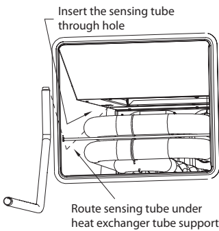
Figure 2. Insert the Sensing Tube
