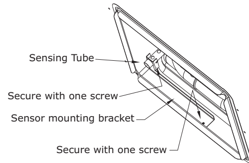
Figure 4. Mounting Bracket
