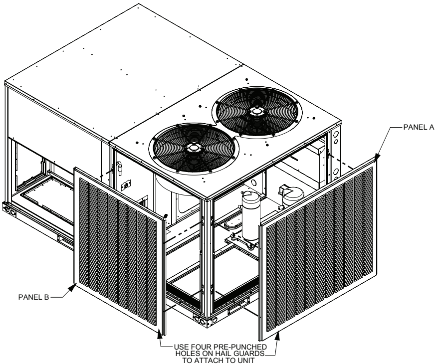
Figure 1. Hail guard installation
