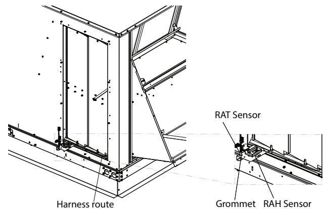
Figure 6. Routing harness through the cutout in horizontal damper
