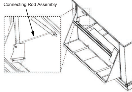
Figure 2. Attach rod to damper
