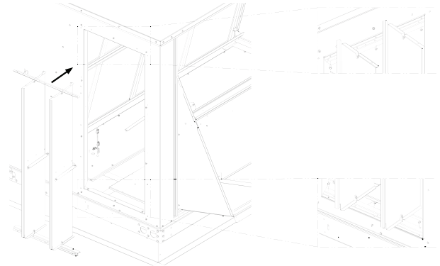
Figure 3. Attach return air damper assembly to return opening
