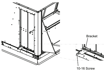
Figure 5. Assembling bracket to horizontal damper
