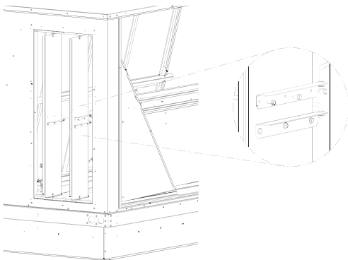
Figure 4. Attach connecting rods to return air damper
