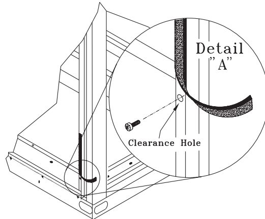
Figure 14. Remove gasket material
