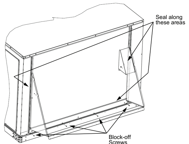
Figure 15. Block-off installation
