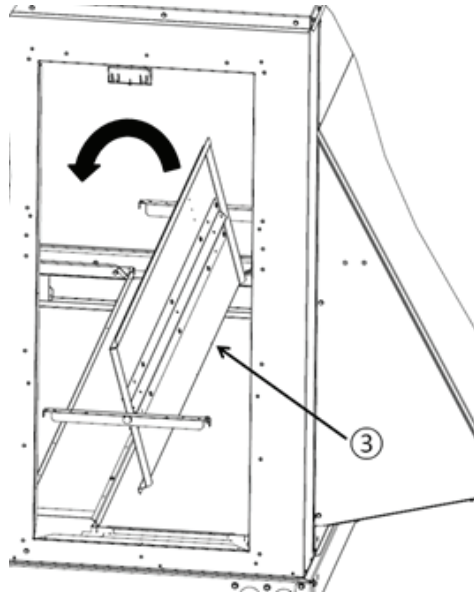
Figure 19. Switch return air assembly from Trane to Carrier
