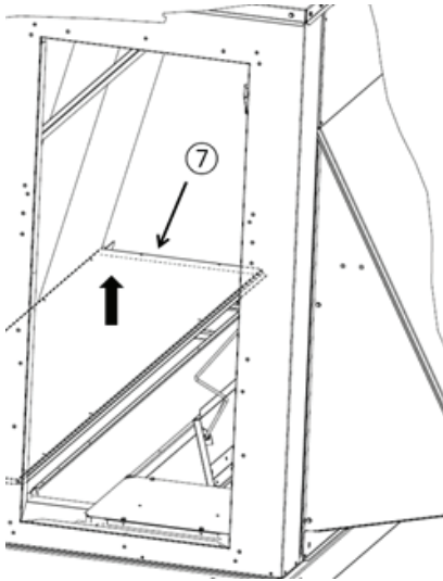
Figure 16. Remove duct cover
