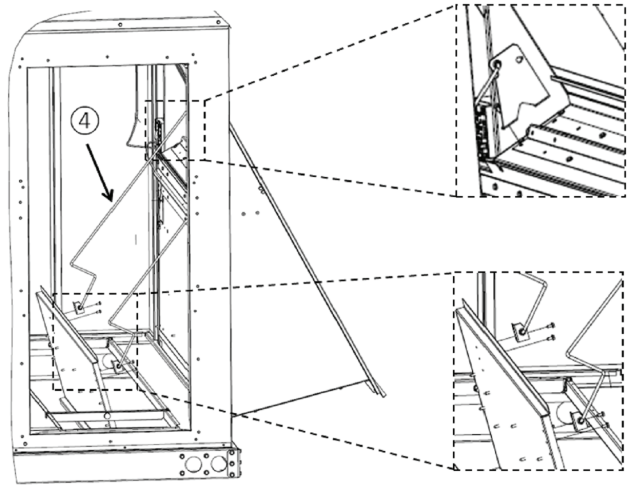
Figure 18. Remove connecting rods
