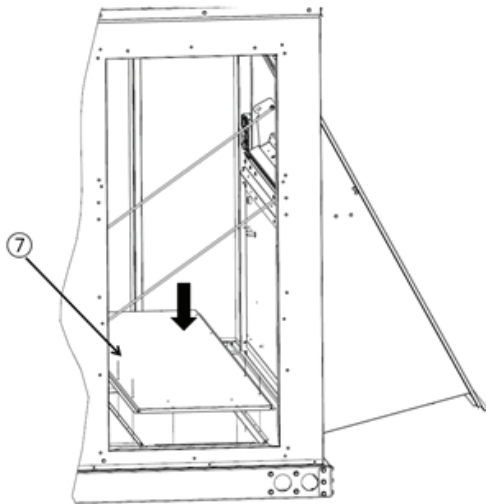
Figure 21. Attach return duct cover
