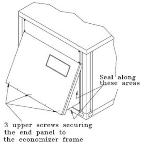
Figure 12. Attach end panel
