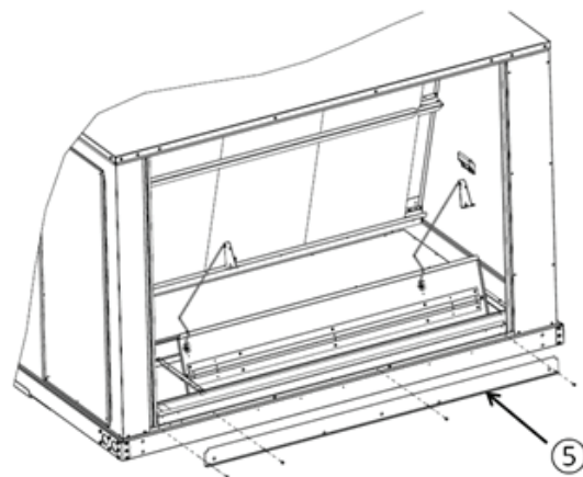
Figure 8. Install block-off
