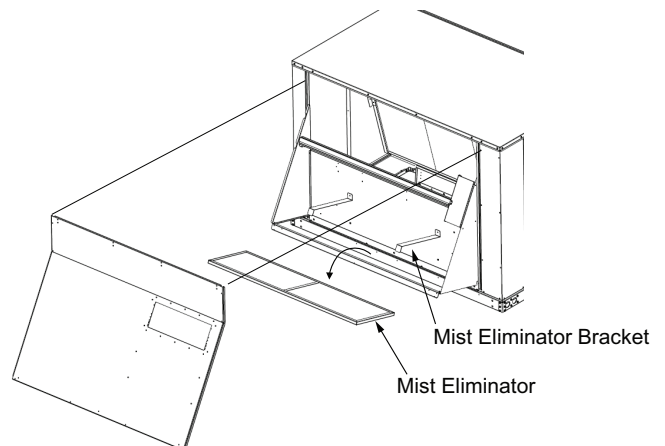
Figure 23. Mist eliminator removal
