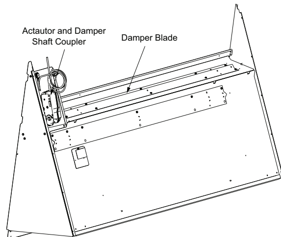
Figure 2. Economizer damper blade
