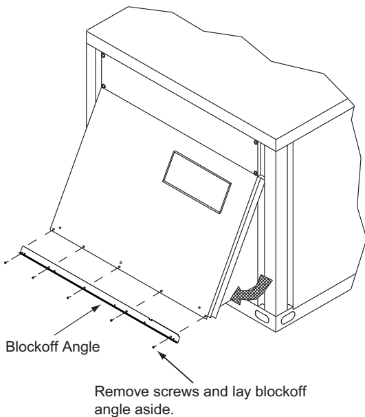
Figure 13. Pull economizer assembly outward
