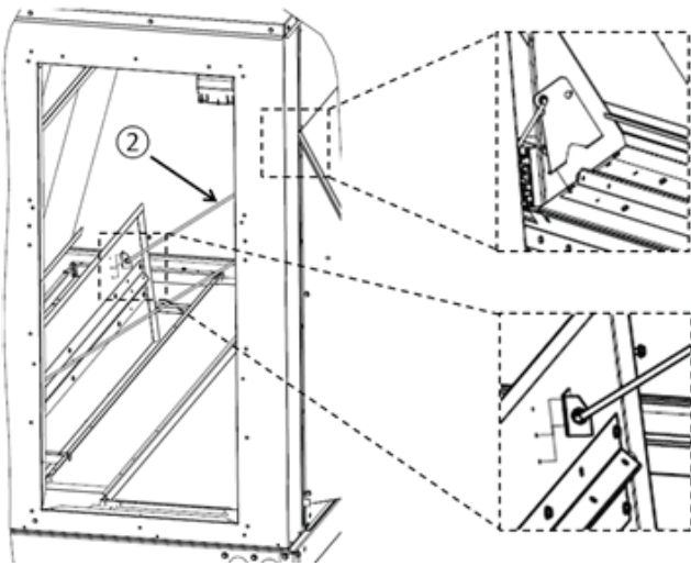
Figure 20. Attach connecting rods
