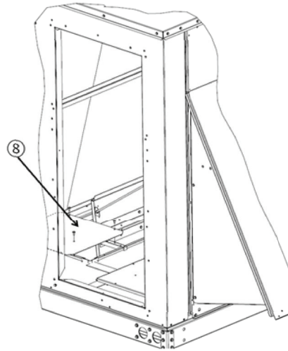
Figure 22. Attach block-off plate
