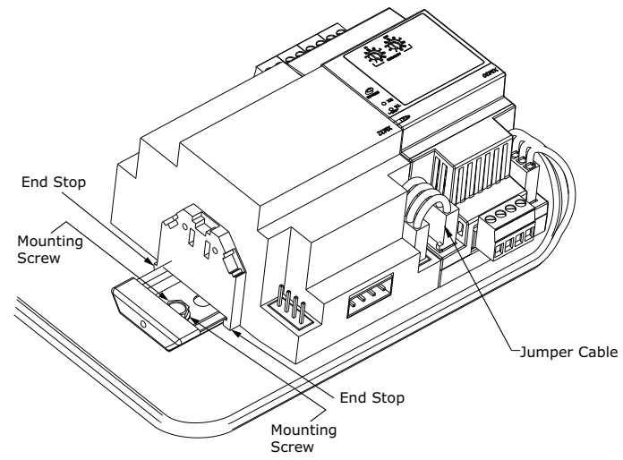
Figure 3. Jumper cables
