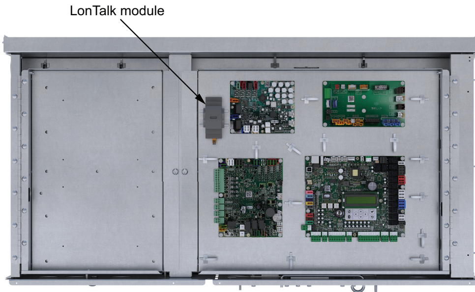
Figure 3. Precedent - LonTalk module location A cabinet
