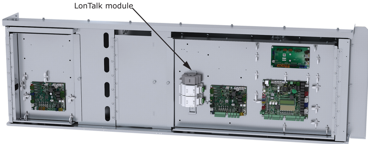
Figure 2. Precedent™ - LonTalk module location (B, C and D Cabinets)
