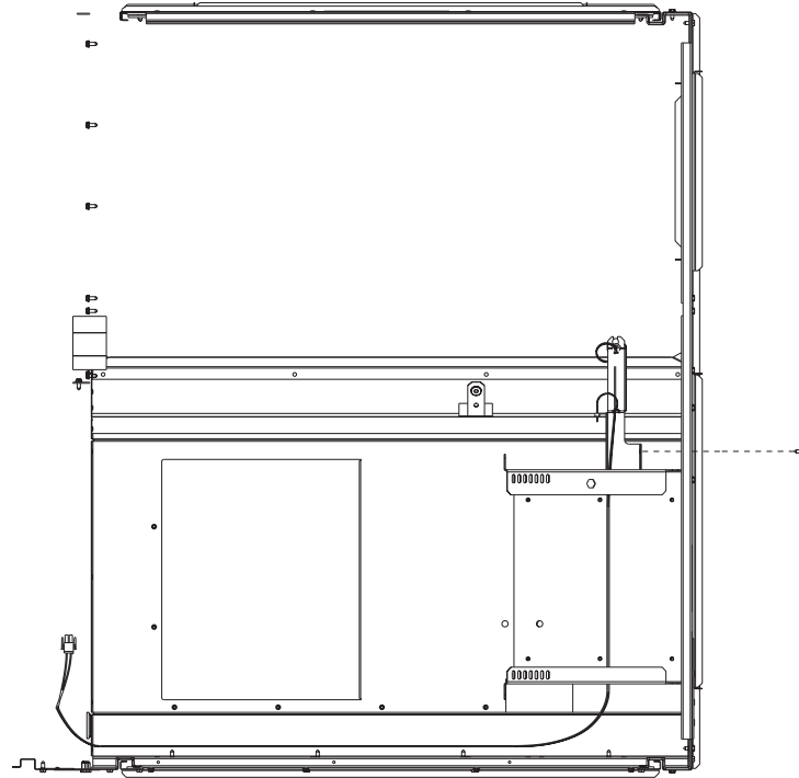
Figure 5. Install drain pan switch
