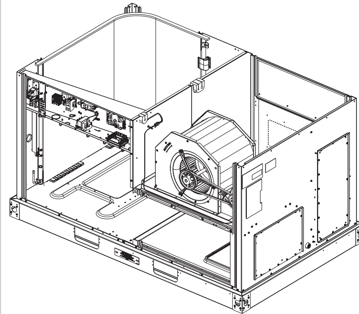
Figure 8. Route drain pan overflow switch wiring
