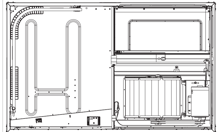
Figure 9. Route drain pan overflow switch wiring - top view
