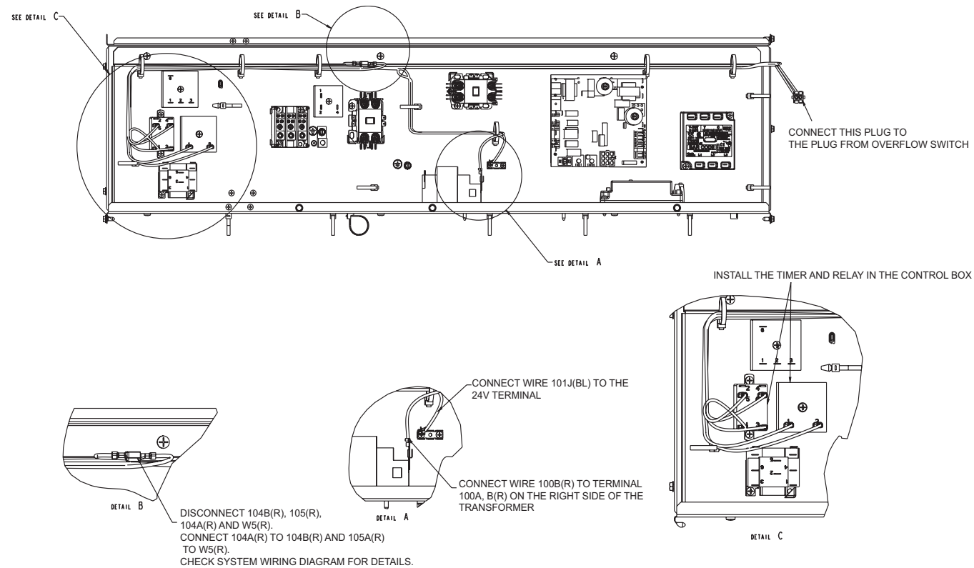
Figure 7. Install relay and timer
