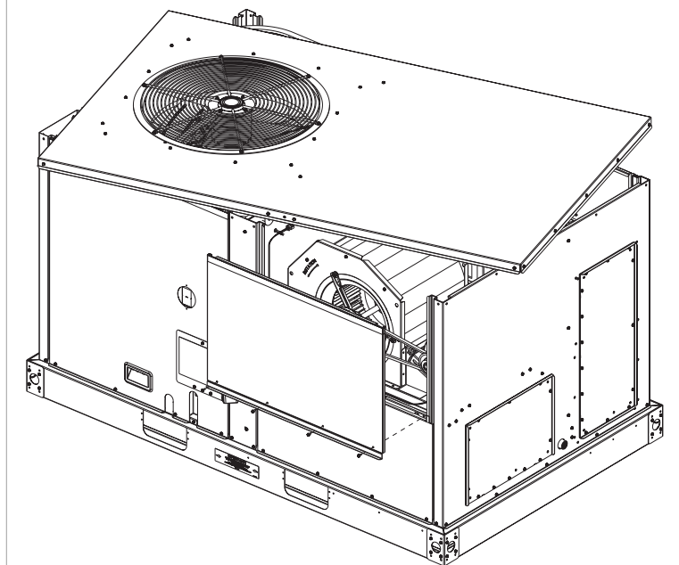
Figure 3. Remove indoor section access panel
