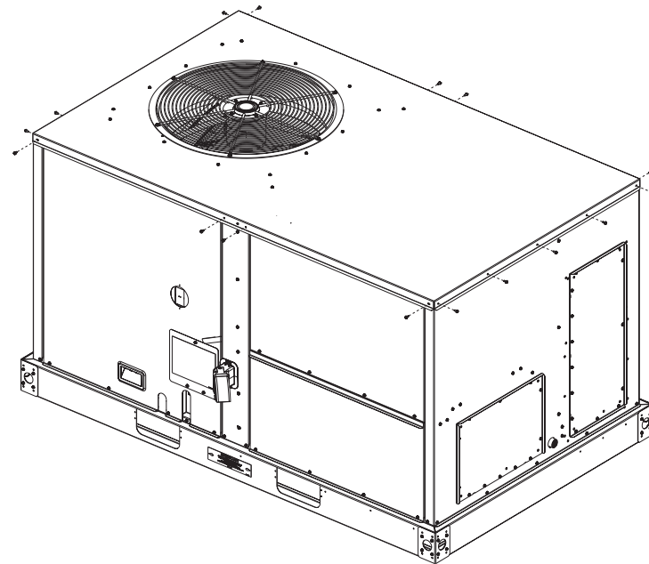
Figure 1. Remove screws around top panel assembly
