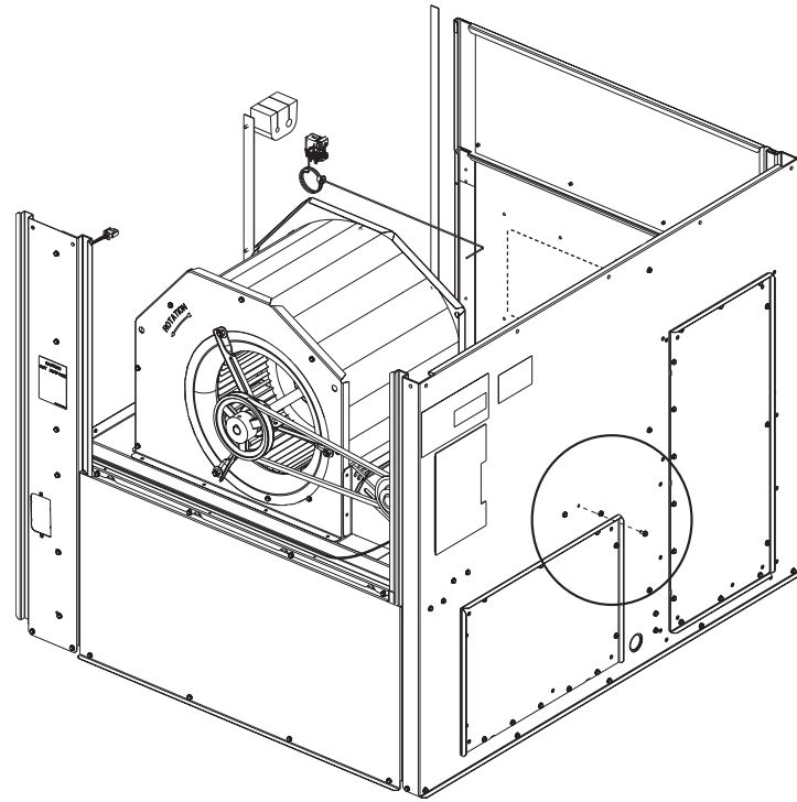
Figure 4. Remove screw from supply panel
