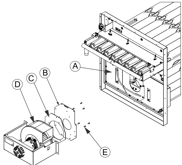
Figure 5. Inducer, gasket, and orifice plate assembly – D cabinet
