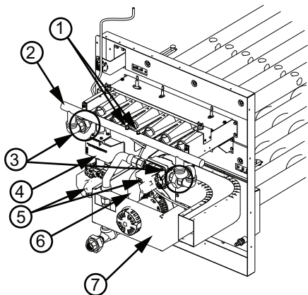
Figure 2. Location of gas heat components and connections – D cabinet
