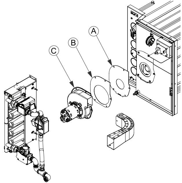
Figure 4. Inducer, gasket, and orifice plate assembly – B and C cabinet
