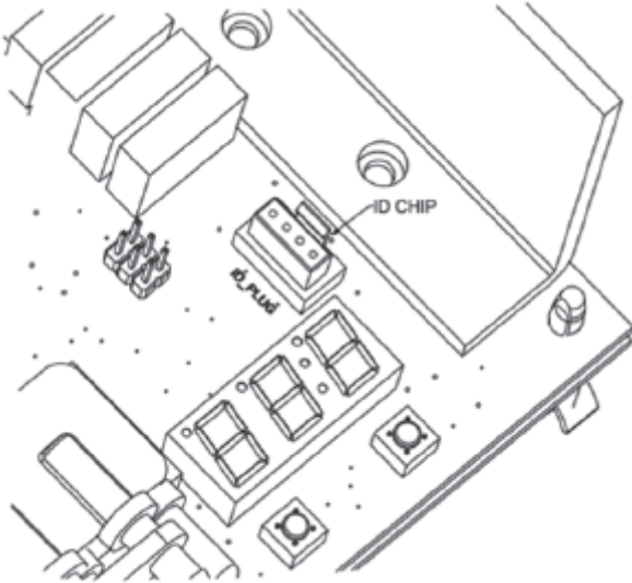
Figure 6. Control board with ID chip and ID plug
