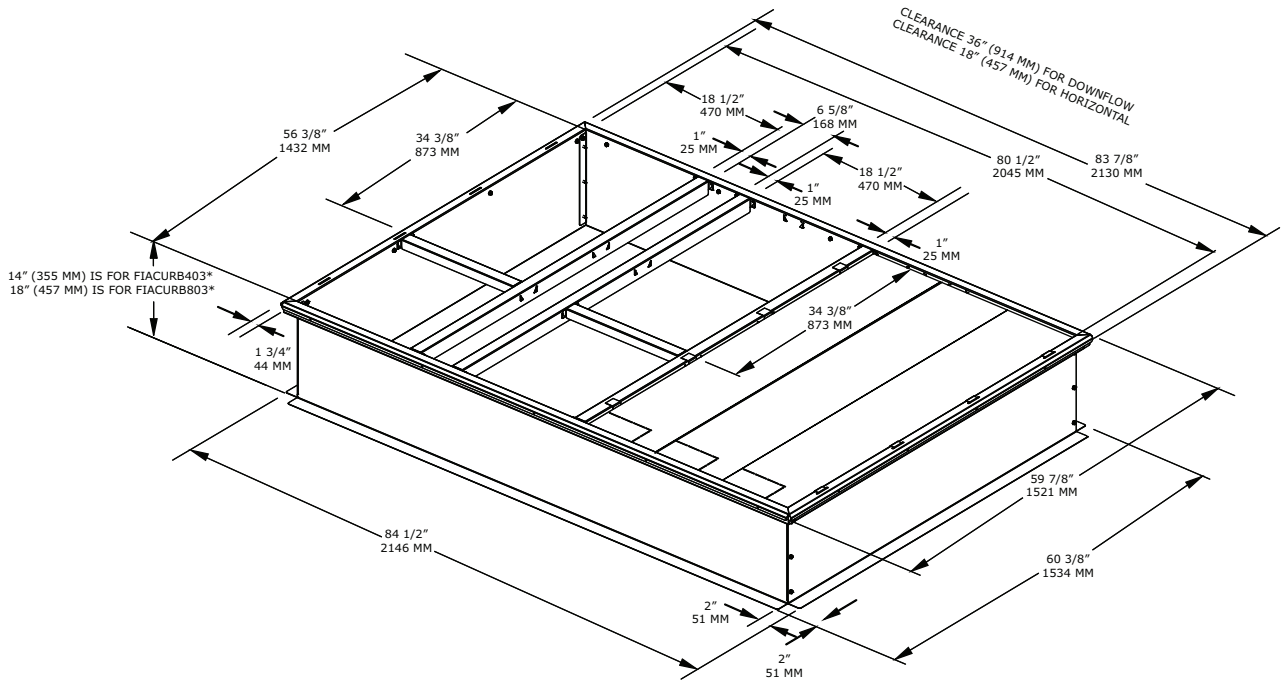
Figure 1. Curb dimensional data
