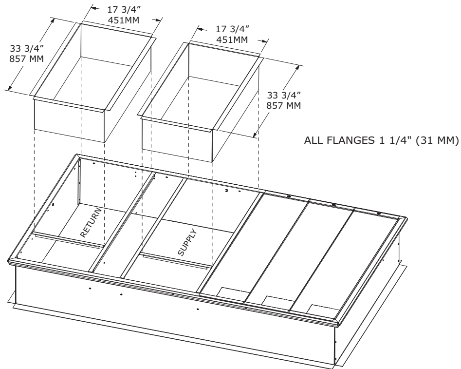
Figure 2. Curb dimensional data
