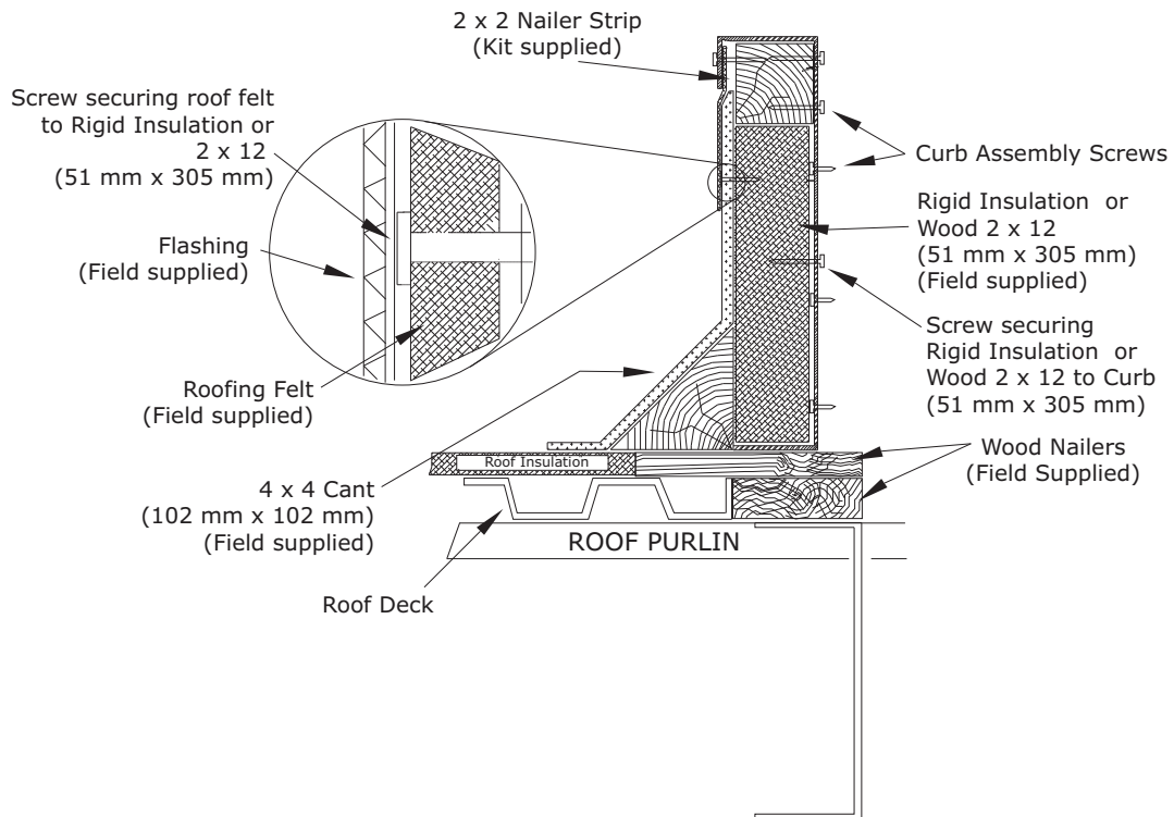
Figure 4. Existing roof construction
