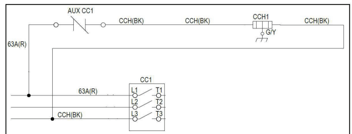
Figure 3. Crankcase heater wiring diagram
