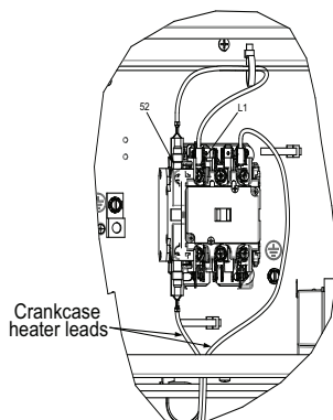
Figure 2. Harness connection between contactor and auxiliary
