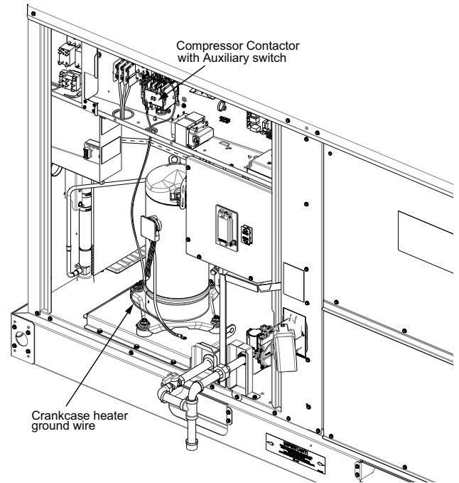
Figure 1. Place CCH band around the bottom of the compressor
