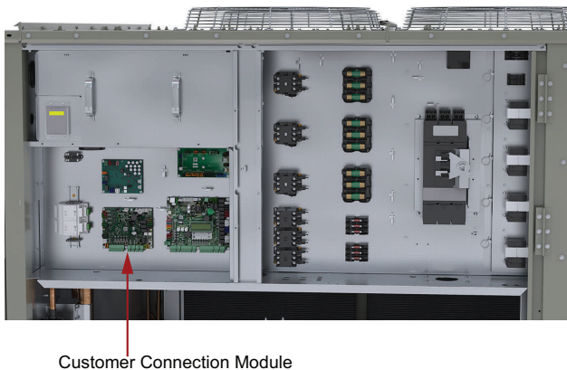
Figure 3. Voyager™ 3 - customer connection module
