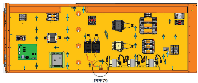
Figure 6. Outdoor motor power harness
