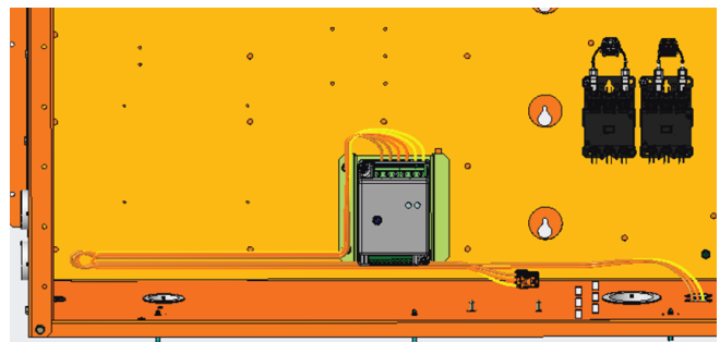
Figure 6. Outdoor motor power harness
