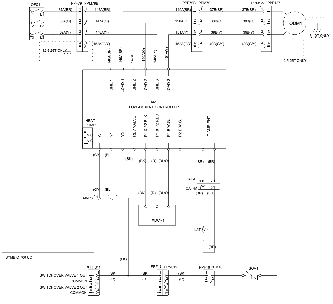
Figure 9. Low ambient controller
