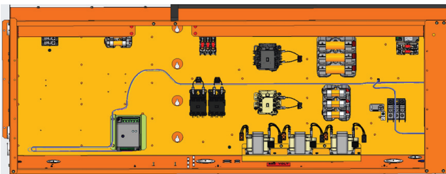
Figure 7. Control power harness
