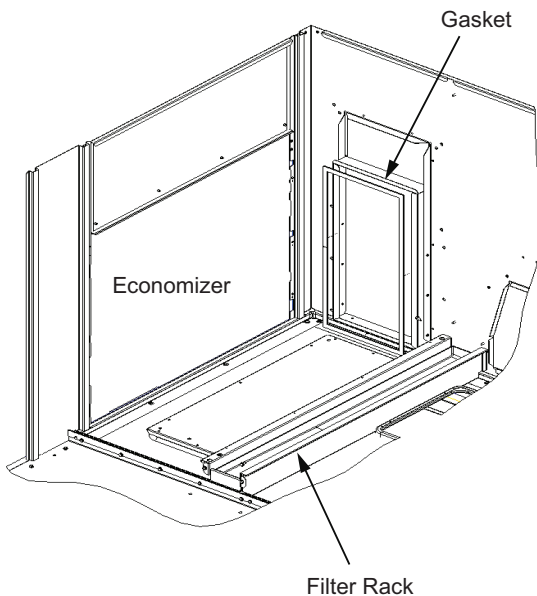
Figure 19. Apply gasket
