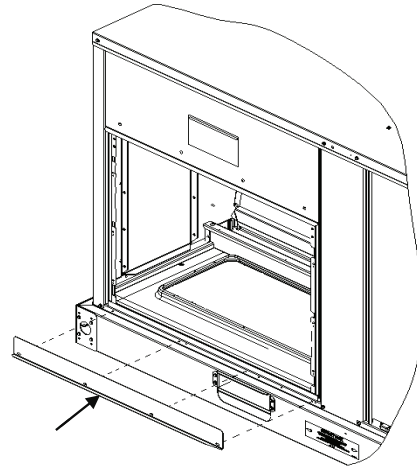
Figure 9. Install block-off
