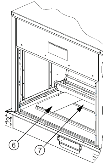
Figure 6. Install duct block-off plate - horizontal
