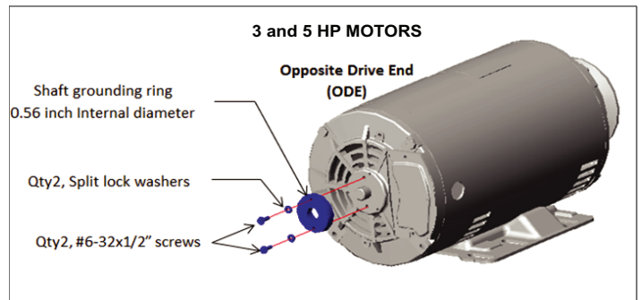
Figure 1. Shaft grounding ring installation on 3 and 5 HP motors
