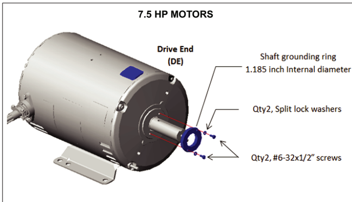
Figure 2. Shaft grounding ring installation on 7.5 HP motors
