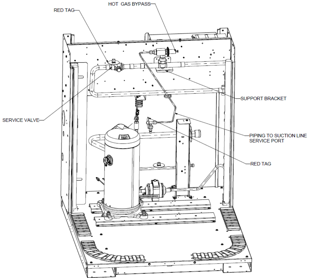
Figure 9. Condensing unit - typical HGBP accessory layout (single circuit system shown, dual circuit systems will only go to circuit A)
