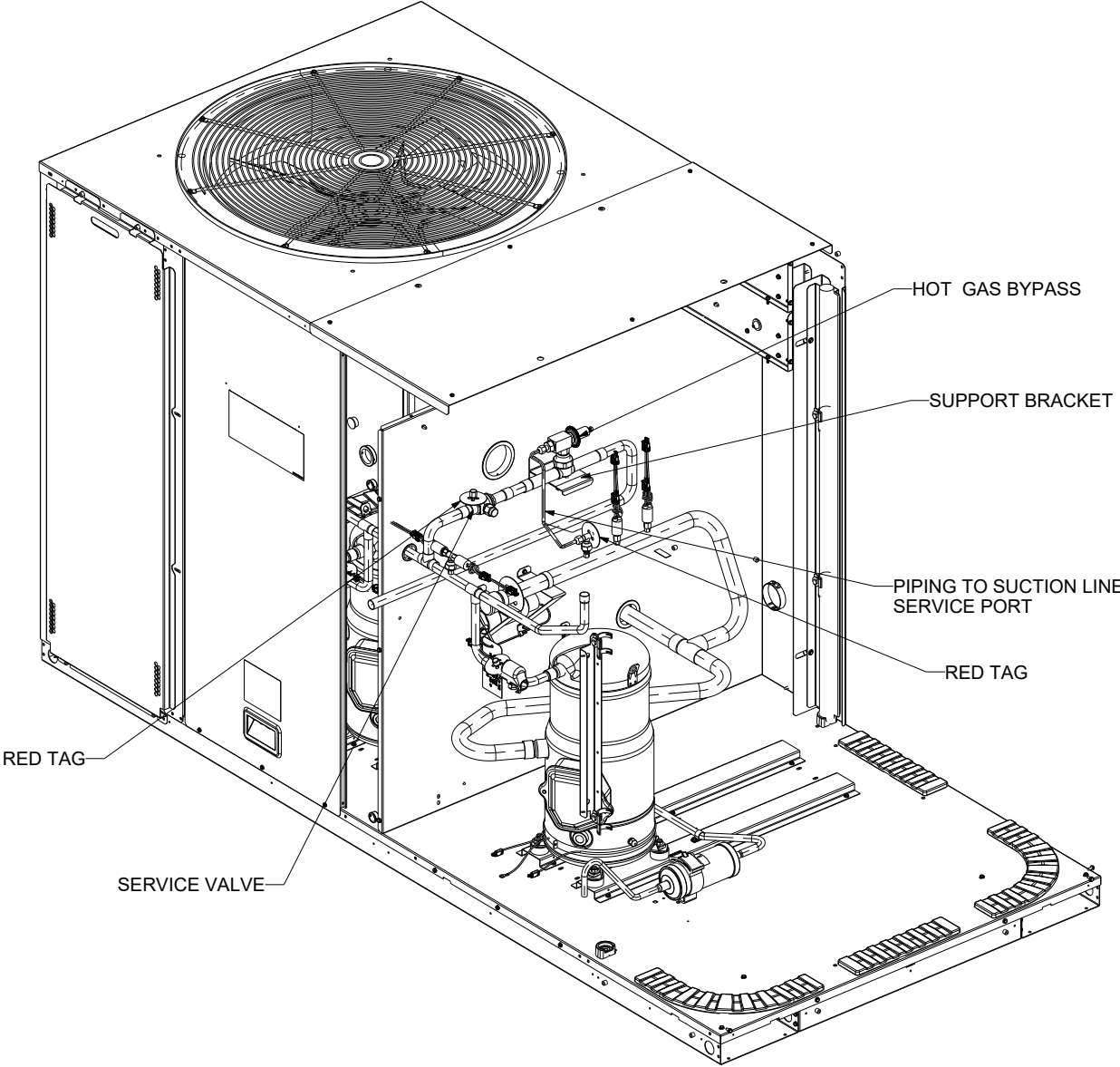
Figure 10. Condensing unit - typical HGBP accessory layout (manifolded system shown, dual circuit systems will only go to circuit A)
