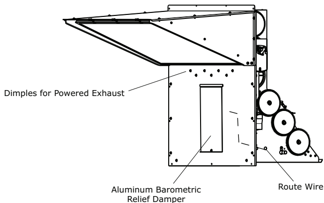
Figure 6. Low leak install
