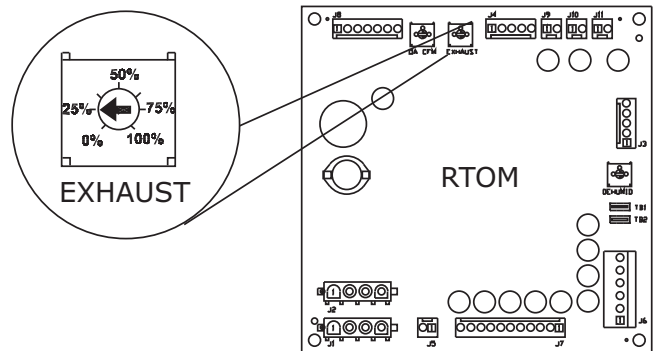
Figure 10. Power exhaust potentiometer
