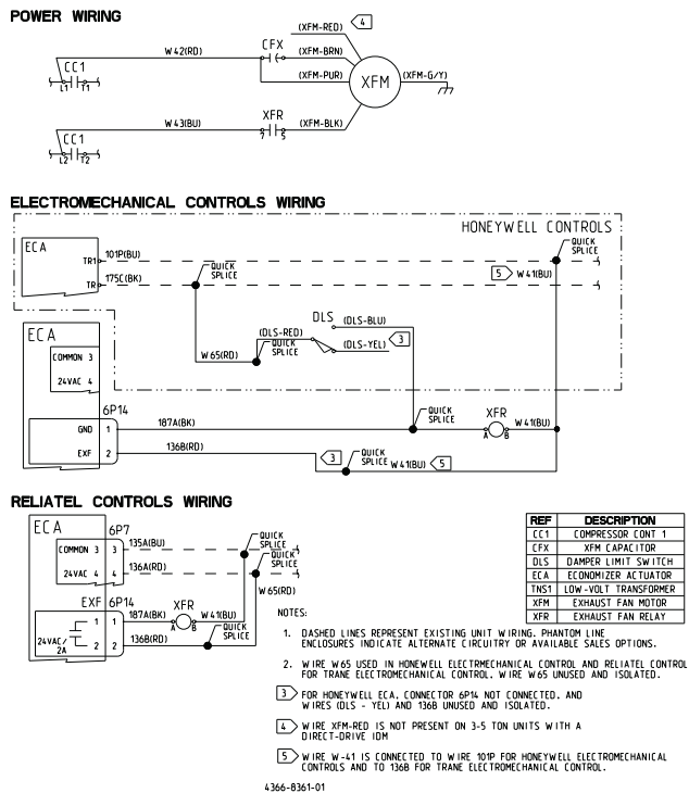
Figure 7. Wiring
