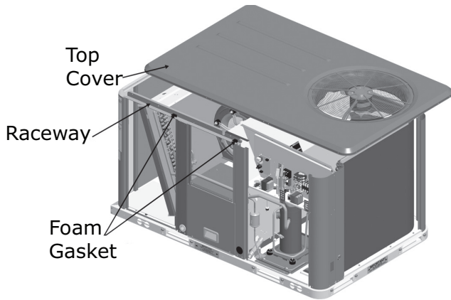
Figure 5. Raceway top view
