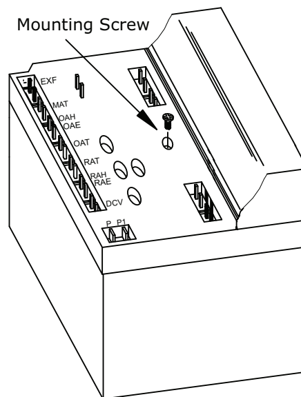
Figure 8. Logic module
