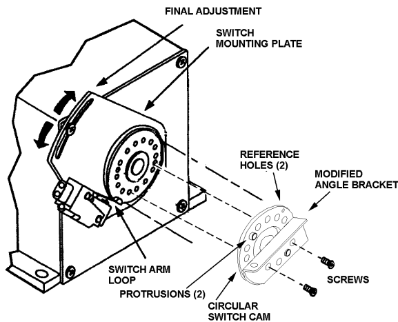
Figure 9. Switch kit installation
