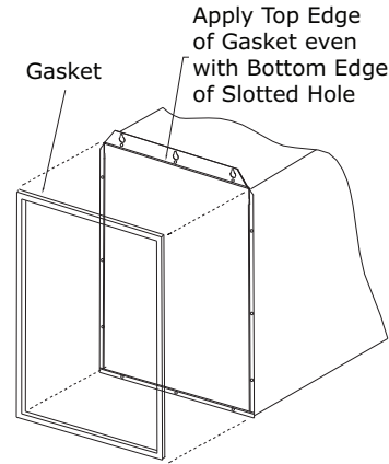
Figure 3. Gasket to power exhaust assembly
