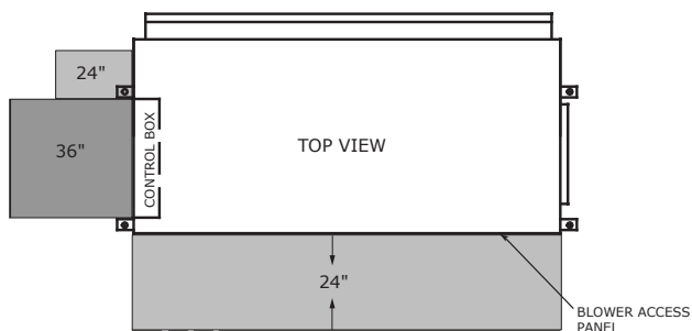
Figure 2. Clearance - GEH 6 to 15 tons
