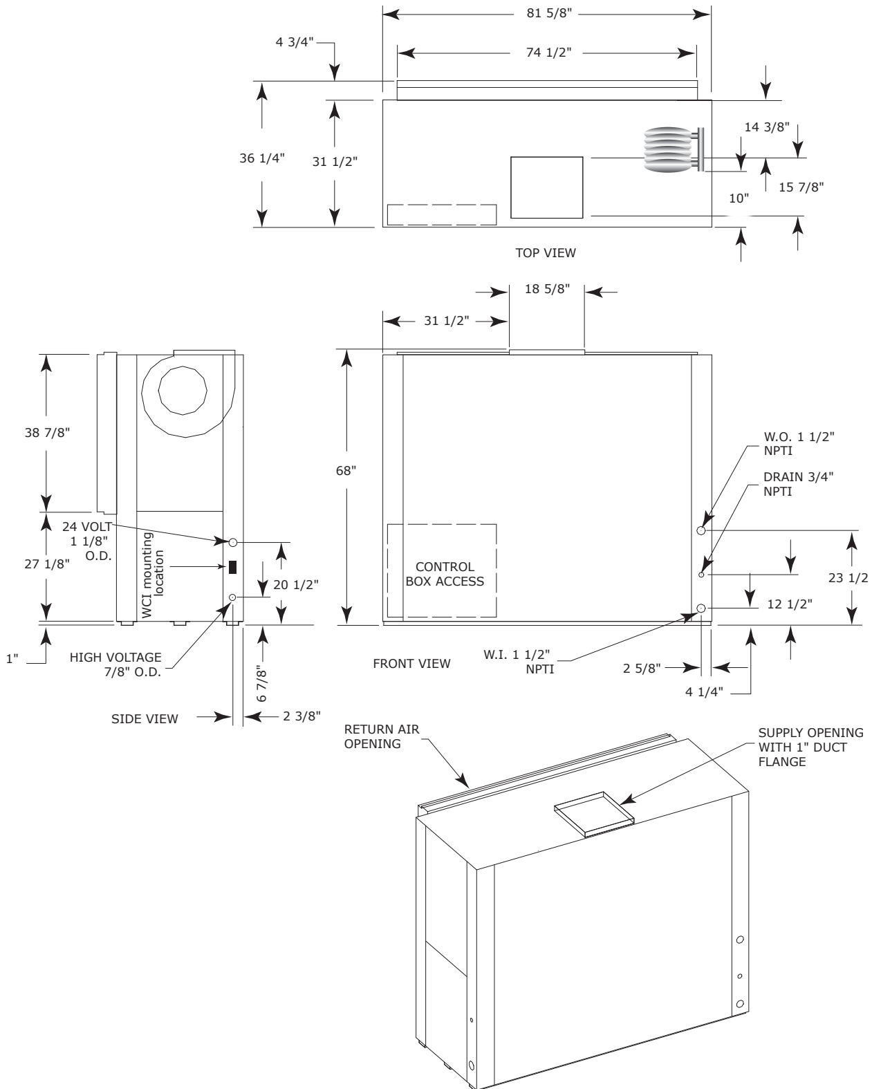
Figure 28. Back return/top supply: GEVK 12.5 to 15 tons (60 Hz); GEVK 10 and 12.5 tons (50 Hz)
