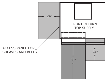
Figure 4. Clearance - GEV 6 to 10 tons
