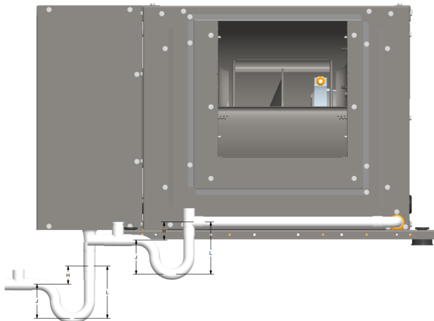
Figure 70. Step 8
