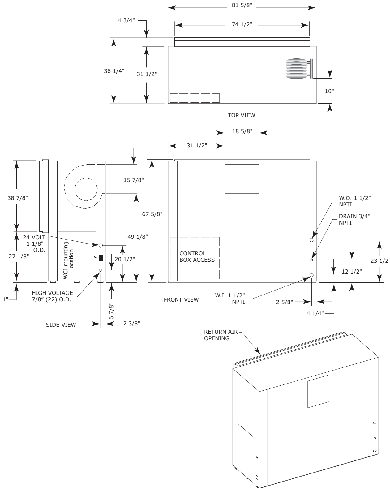
Figure 26. Back return/front supply GEVK 12.5 to 15 tons (60 Hz); GEVK 10 and 12.5 tons (50 Hz)
