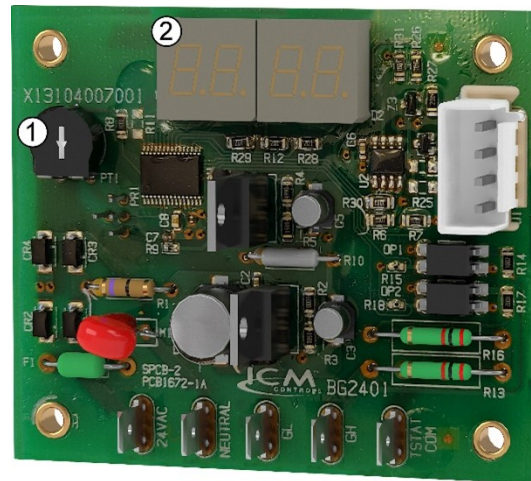
Figure 66. ECM control board
