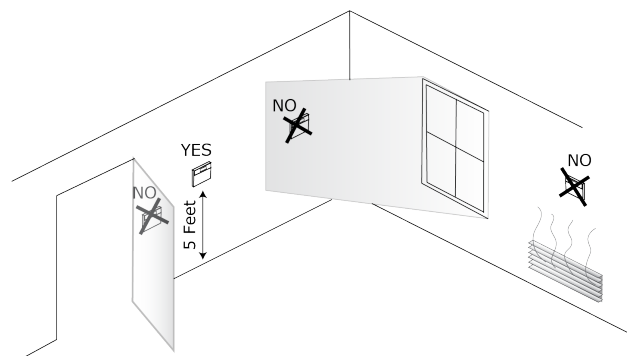
Figure 53. Thermostat/sensor location
