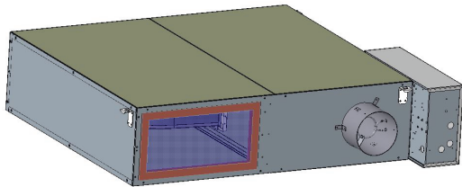
Figure 6. Low height parallel: LPCF
