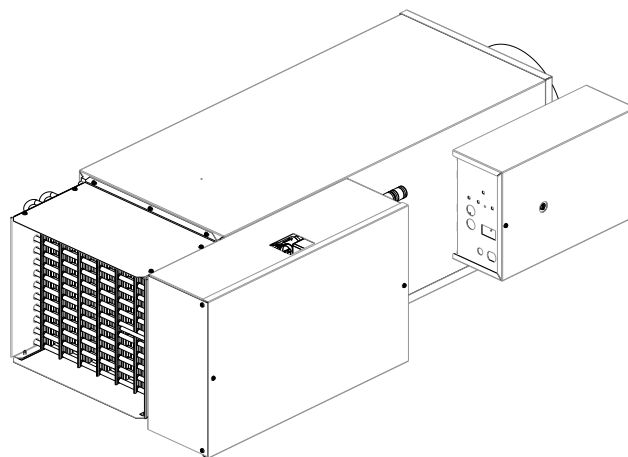
Figure 10. Typical hot water single duct unit with factory installed piping package
