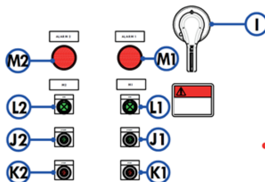
Figure 22. Cooling tower starter panel door layout
