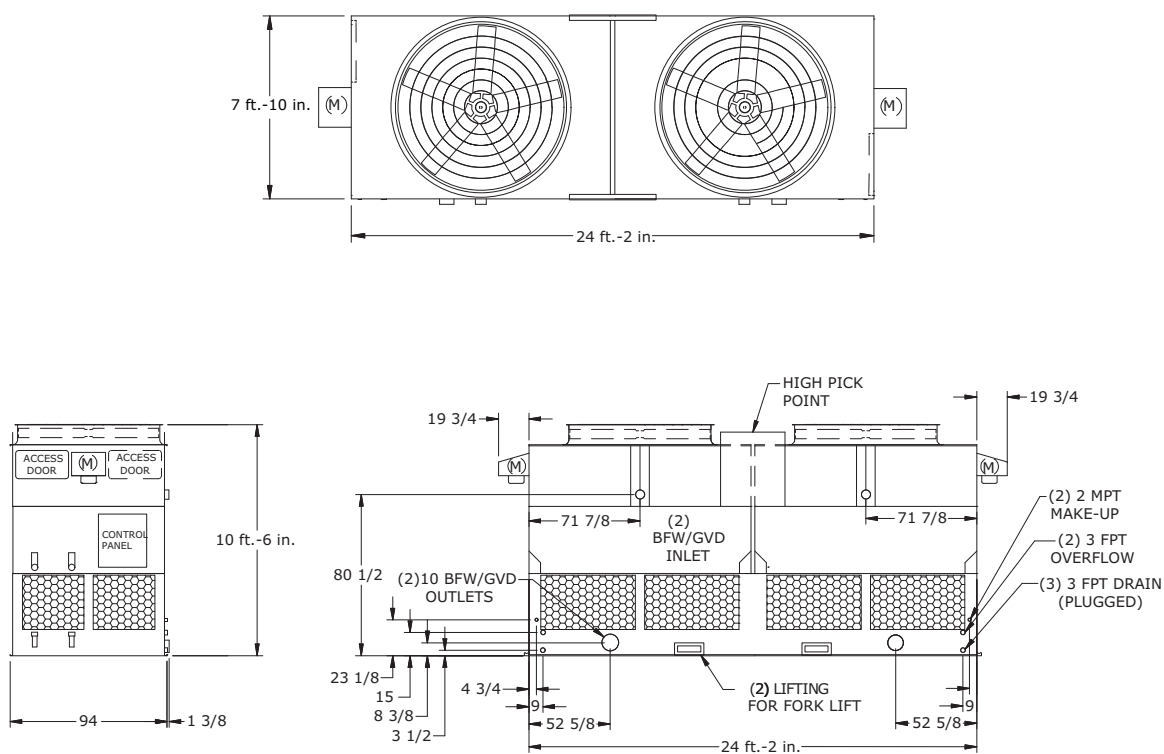
Figure 26. Unit drawing
