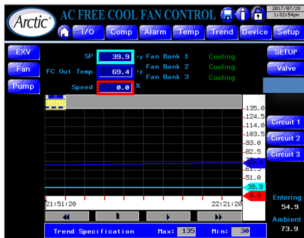
Figure 29. Free-cool fan control page
