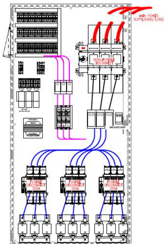
Figure 4. Power panel
