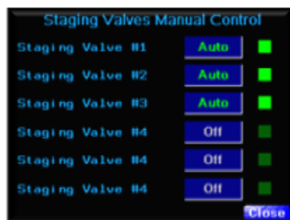
Figure 27. Staging valves control screen
