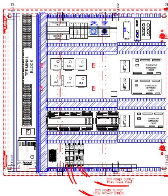
Figure 5. Control panel
