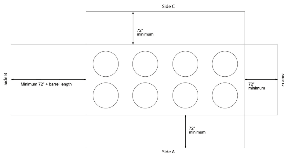
Figure 1. Recommended chiller clearances
