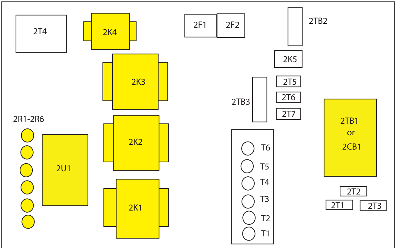
Figure 5. Remove the highlighted components (wye-delta starter) — RTHA-YD
