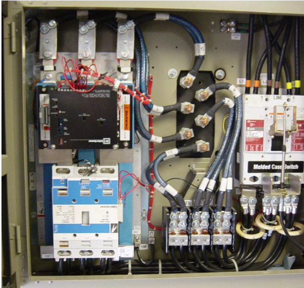
Figure 20. Location of Benshaw starter and additional components (highlighted)
