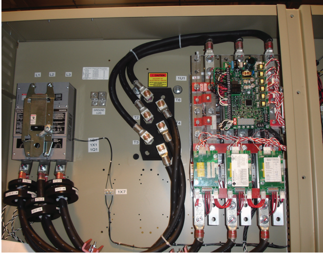
Figure 33. Benshaw starter installed — RTHD
