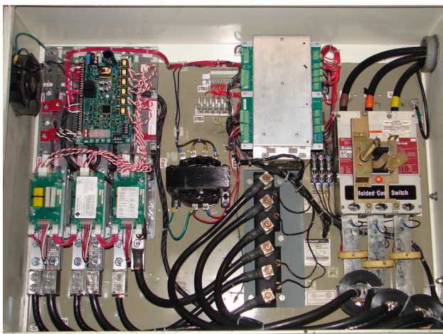
Figure 14. Benshaw starter installed — RTHB
