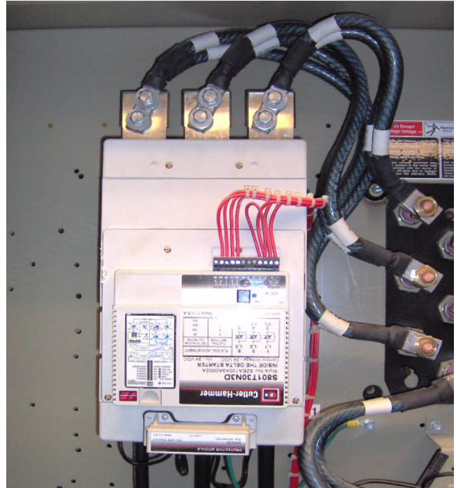
Figure 3. Cutler-Hammer EasySTART
