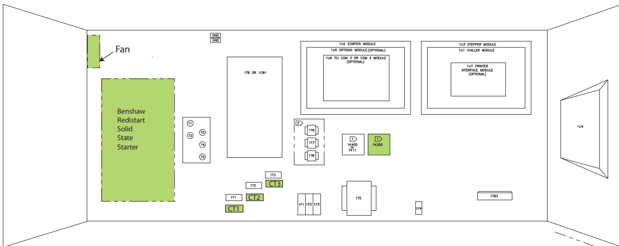
Figure 26. Location of benshaw starter and additional components (highlighted) — RTHC
