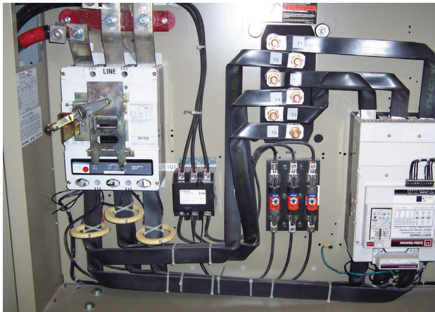
Figure 32. Location of benschaw starter — RTHD
