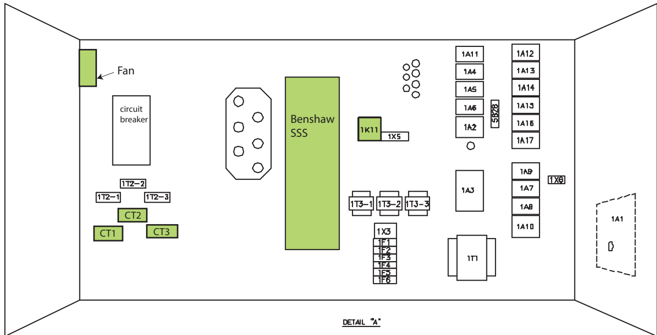
Figure 32. Location of benschaw starter — RTHD
