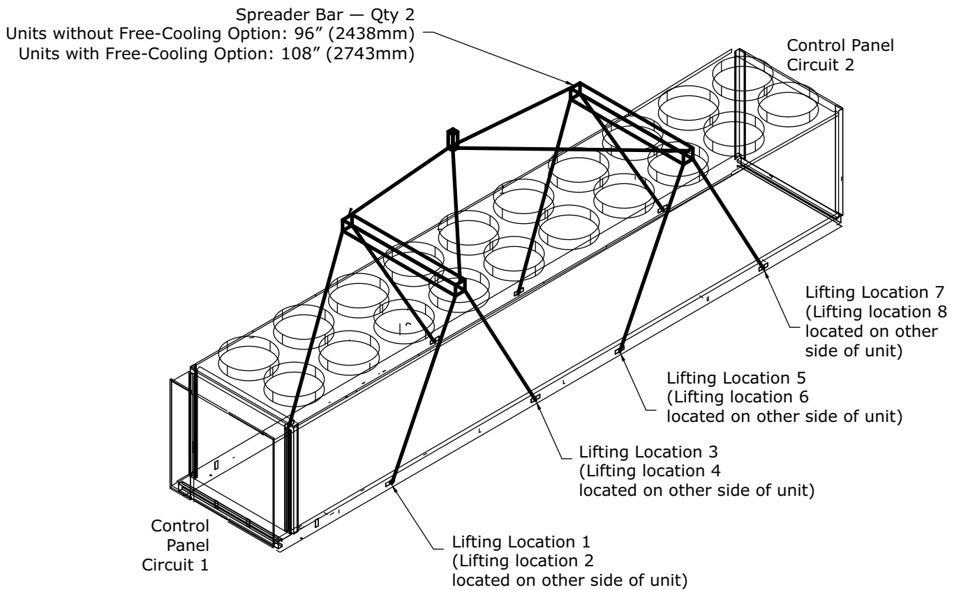
Figure 22. Lifting configuration — 8 point
