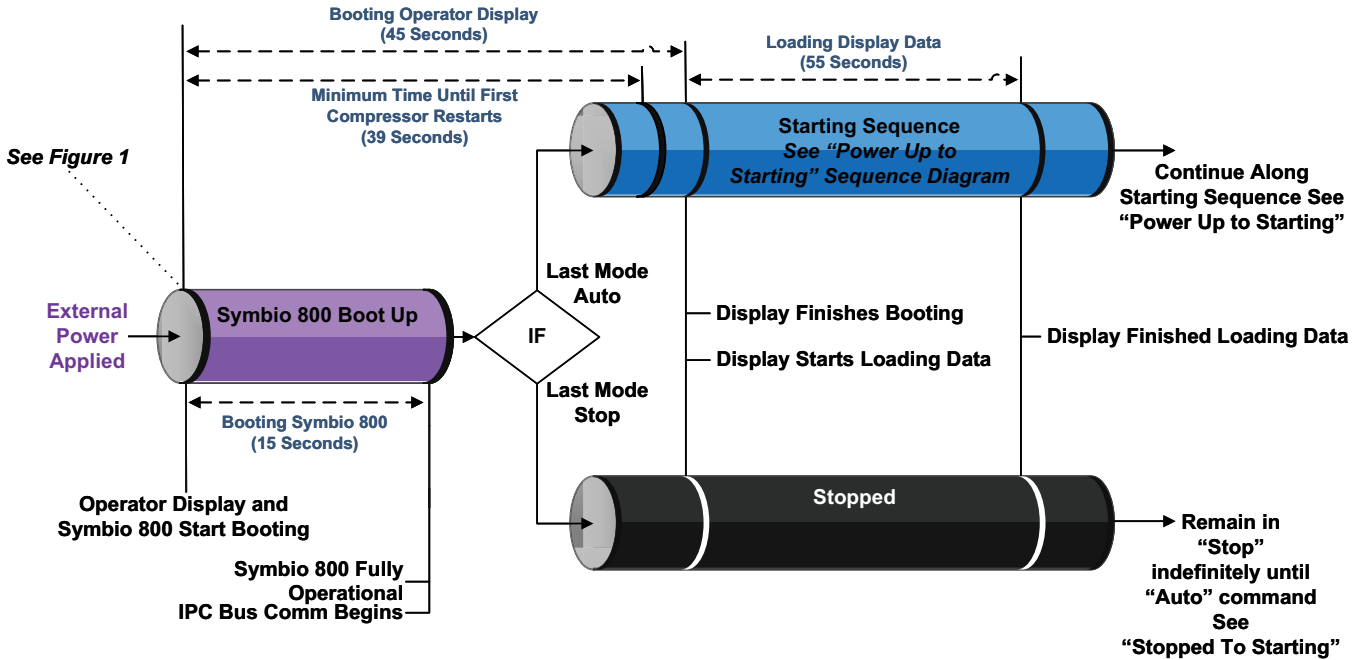
Figure 54. Sequence of operation: power up diagram
