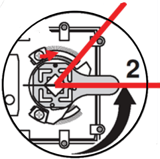
Figure 69. By-pass valve setting photo
