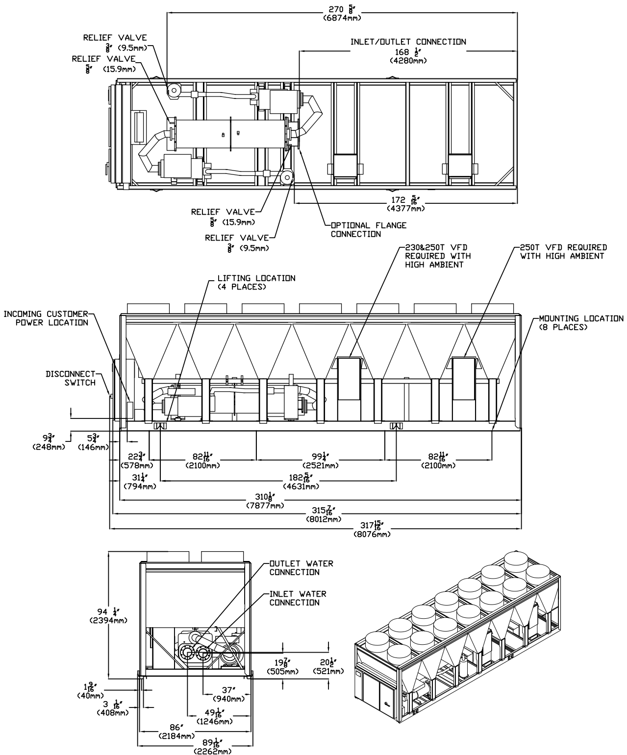
Figure 7. RTAF unit dimensions — 230, 250, 270 ton
