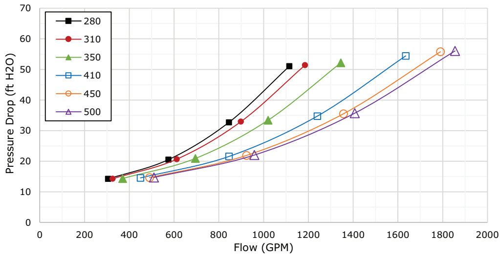
Figure 44. Evaporator water pressure drop, 35% propylene glycol, free-cooling off — 280 to 500 tons, 1-pass without turbulators
