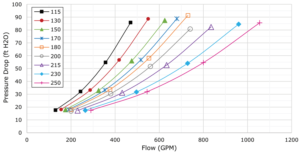
Figure 48. Evaporator water pressure drop, 35% propylene glycol, free-cooling off — 280 to 500 tons, 1-pass with turbulators
