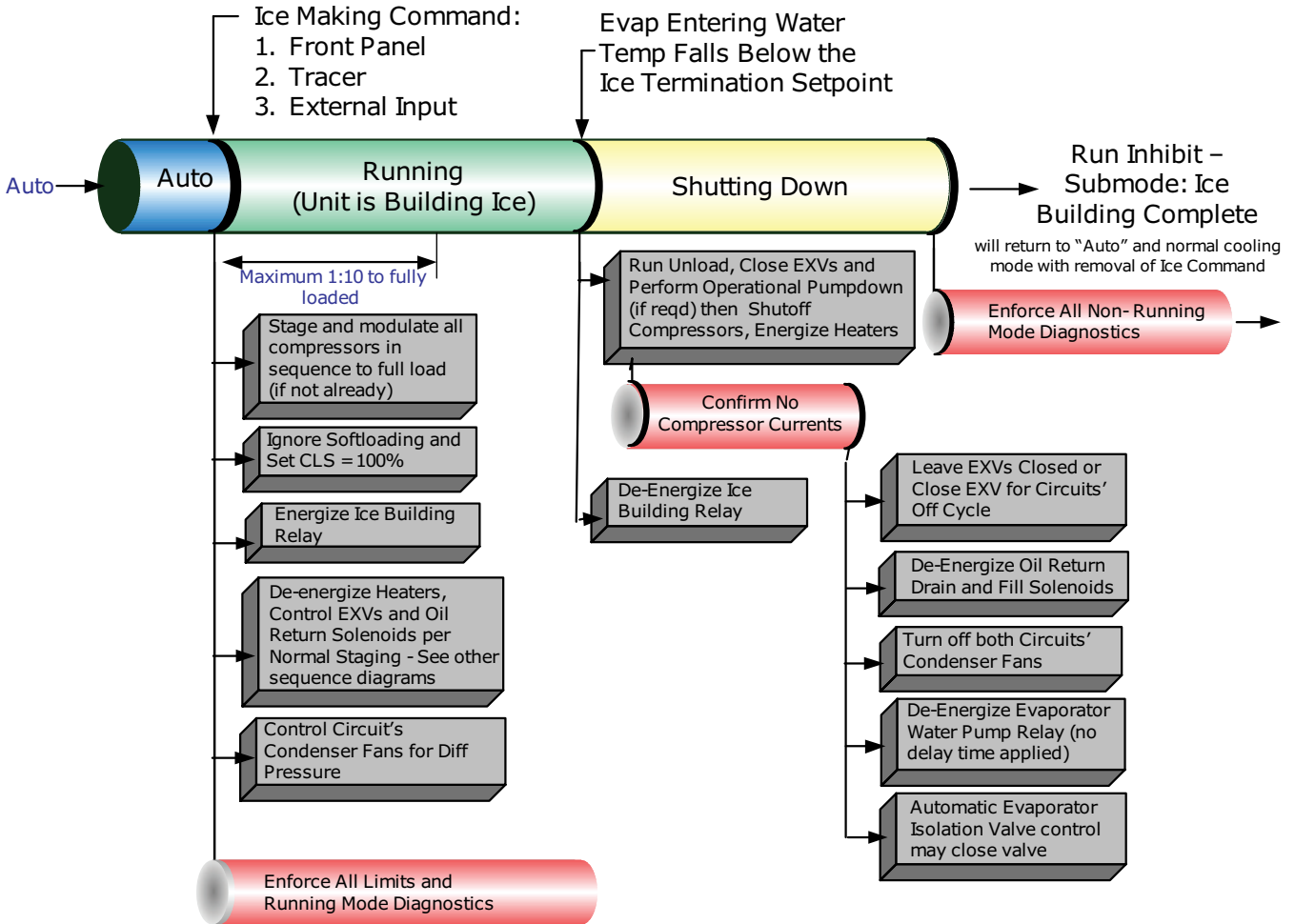
Figure 64. Sequence of events: ice making (auto to ice making to ice making complete)
