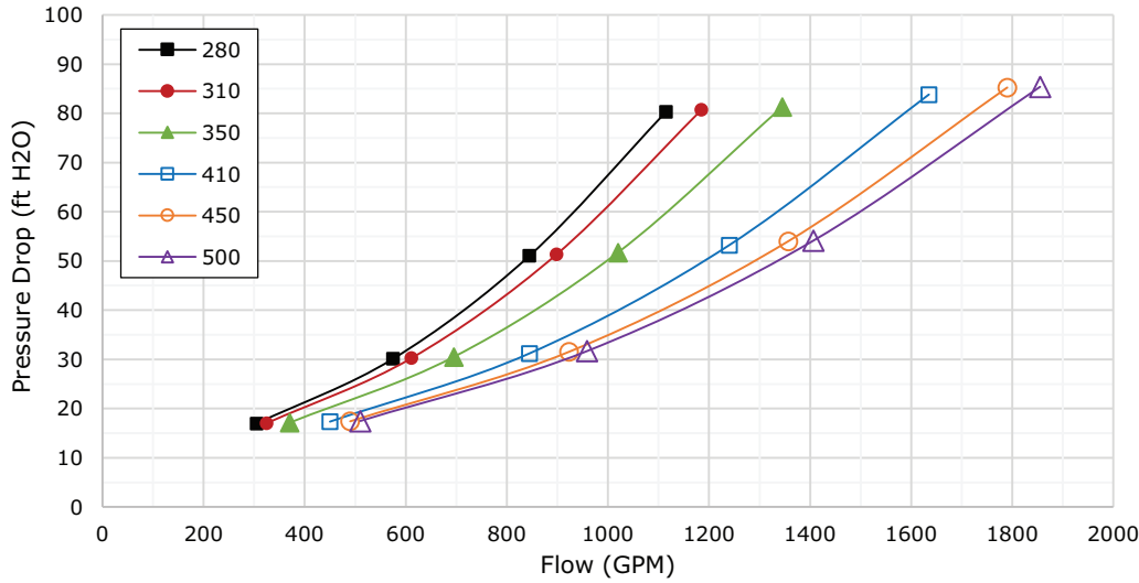
Figure 40. Evaporator water pressure drop, 35% ethylene glycol, free-cooling off — 280 to 500 tons, 1-pass with turbulators
