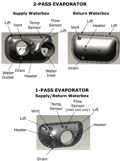
Figure 26. Waterbox configurations
