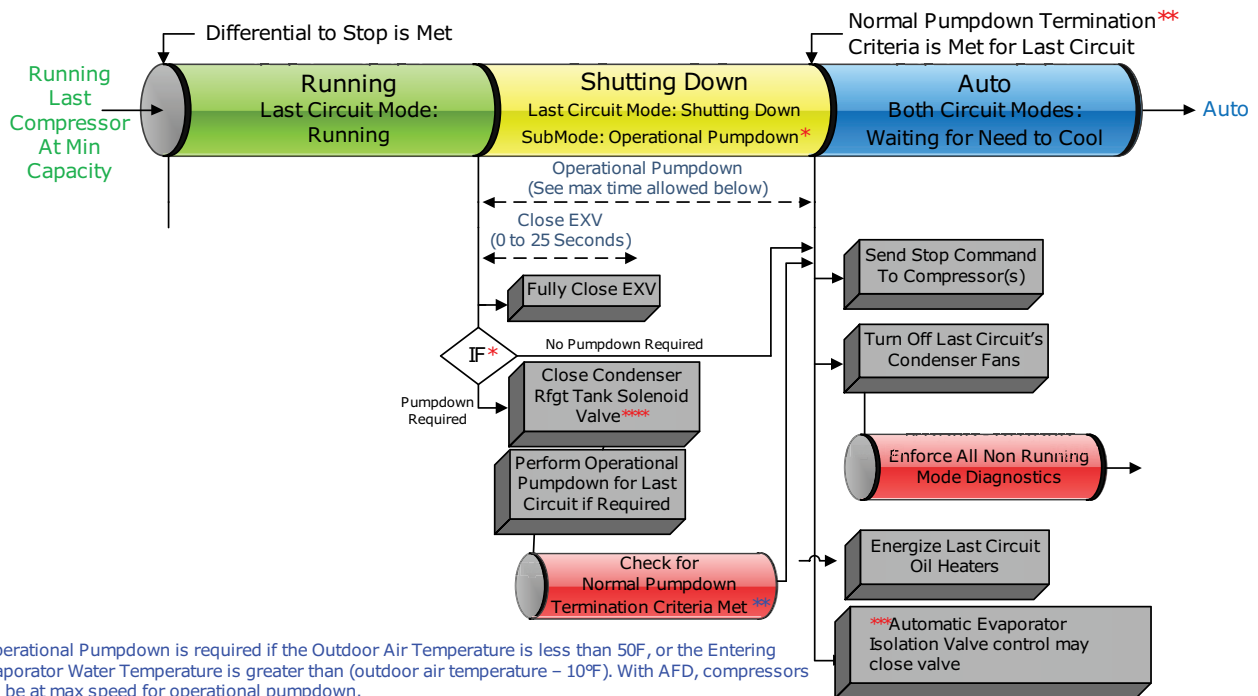
Figure 59. Sequence of events: satisfied setpoint
