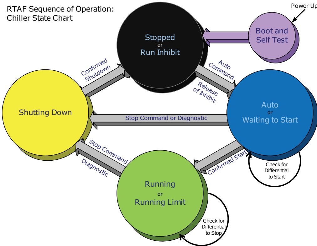
Figure 53. Software operation overview
