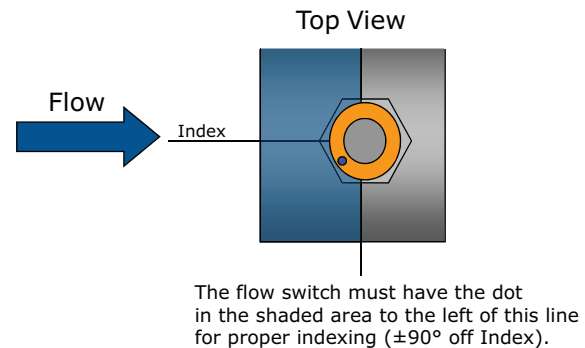
Figure 28. Proper flow switch indexing
