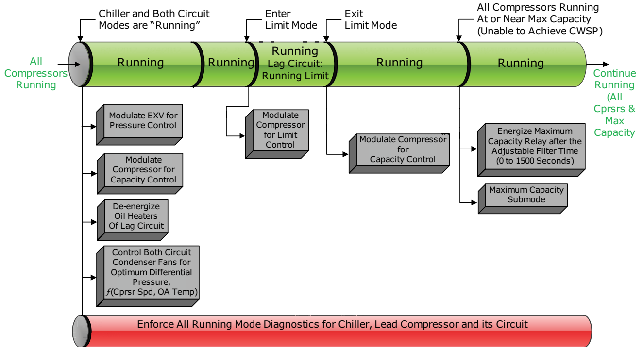
Figure 58. Sequence of operation: running (lag compressor/circuit start and run)
