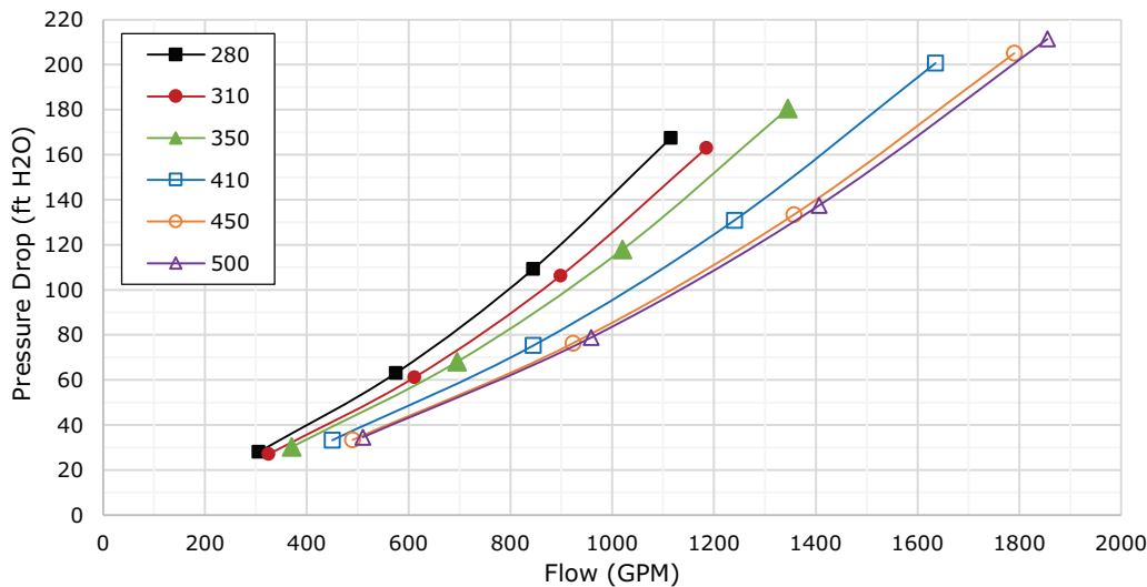
Figure 38. Evaporator water pressure drop, 35% ethylene glycol, free-cooling on — 280 to 500 tons, 1-pass with turbulators
