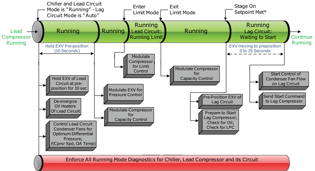
Figure 57. Sequence of operation: running (lead compressor/circuit start and run)
