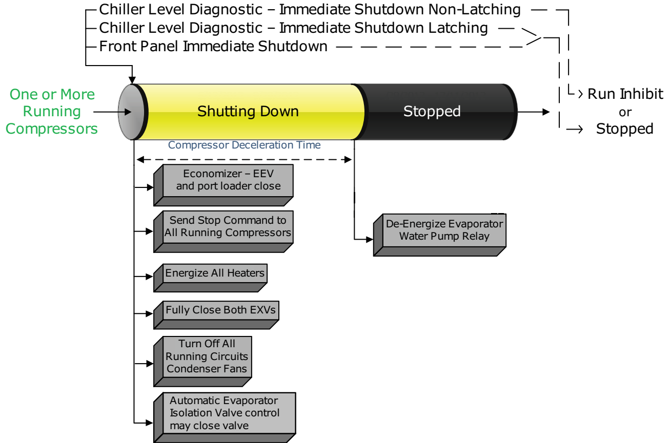
Figure 62. Sequence of events: immediate shutdown to stopped or run inhibit
