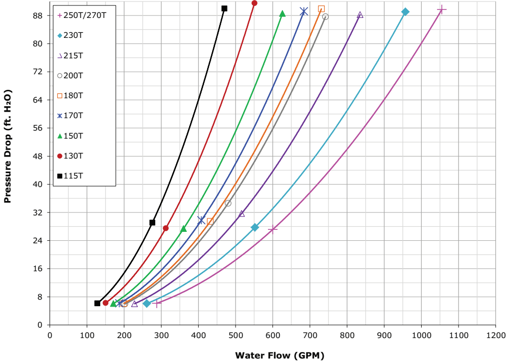
Figure 32. Evaporator water pressure drop — 280 to 520 tons, 1-pass with turbulators
