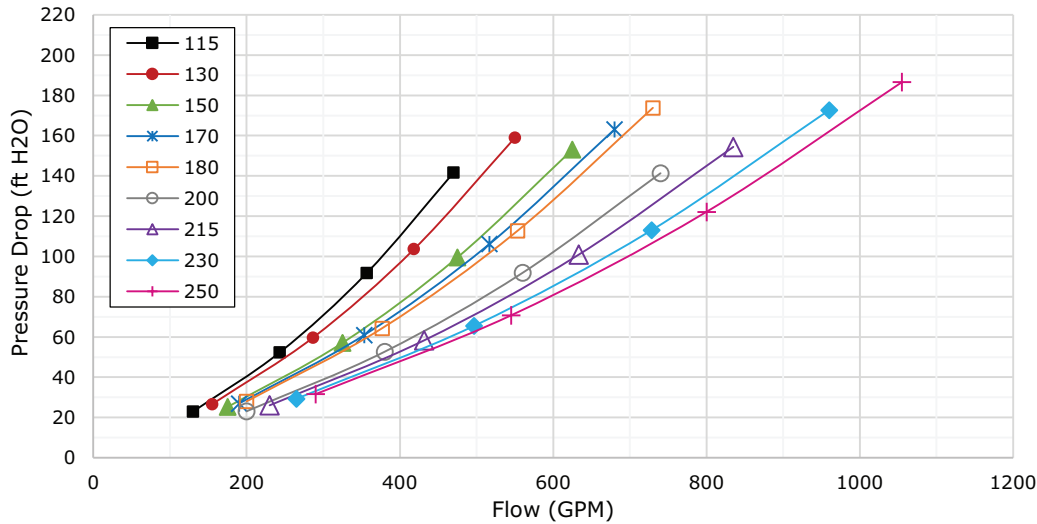
Figure 38. Evaporator water pressure drop, 35% ethylene glycol, free-cooling on — 280 to 500 tons, 1-pass with turbulators
