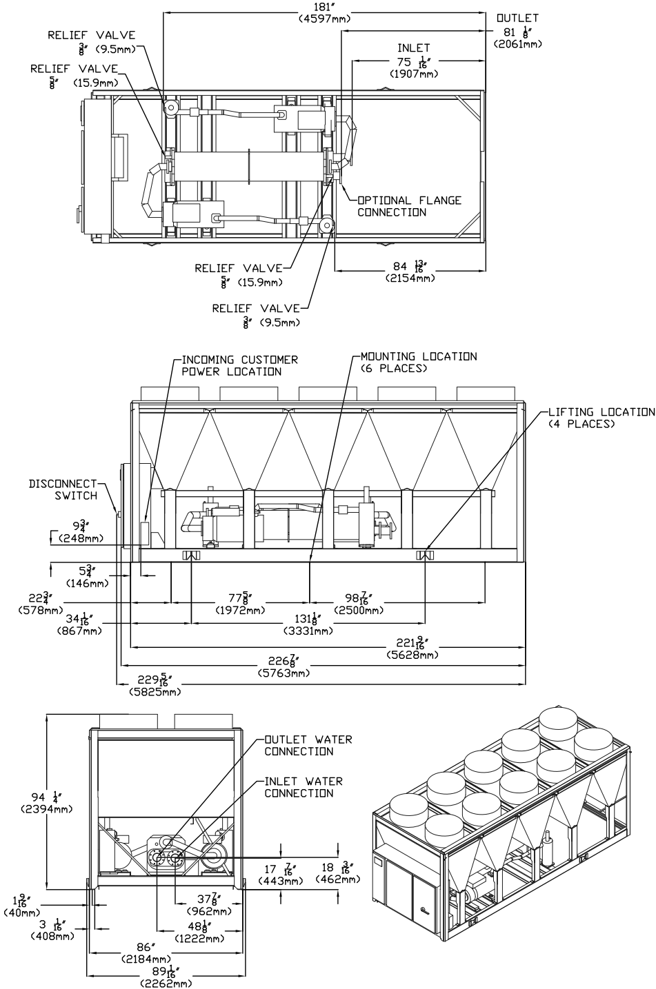
Figure 4. RTAF unit dimensions — 115, 130 ton
