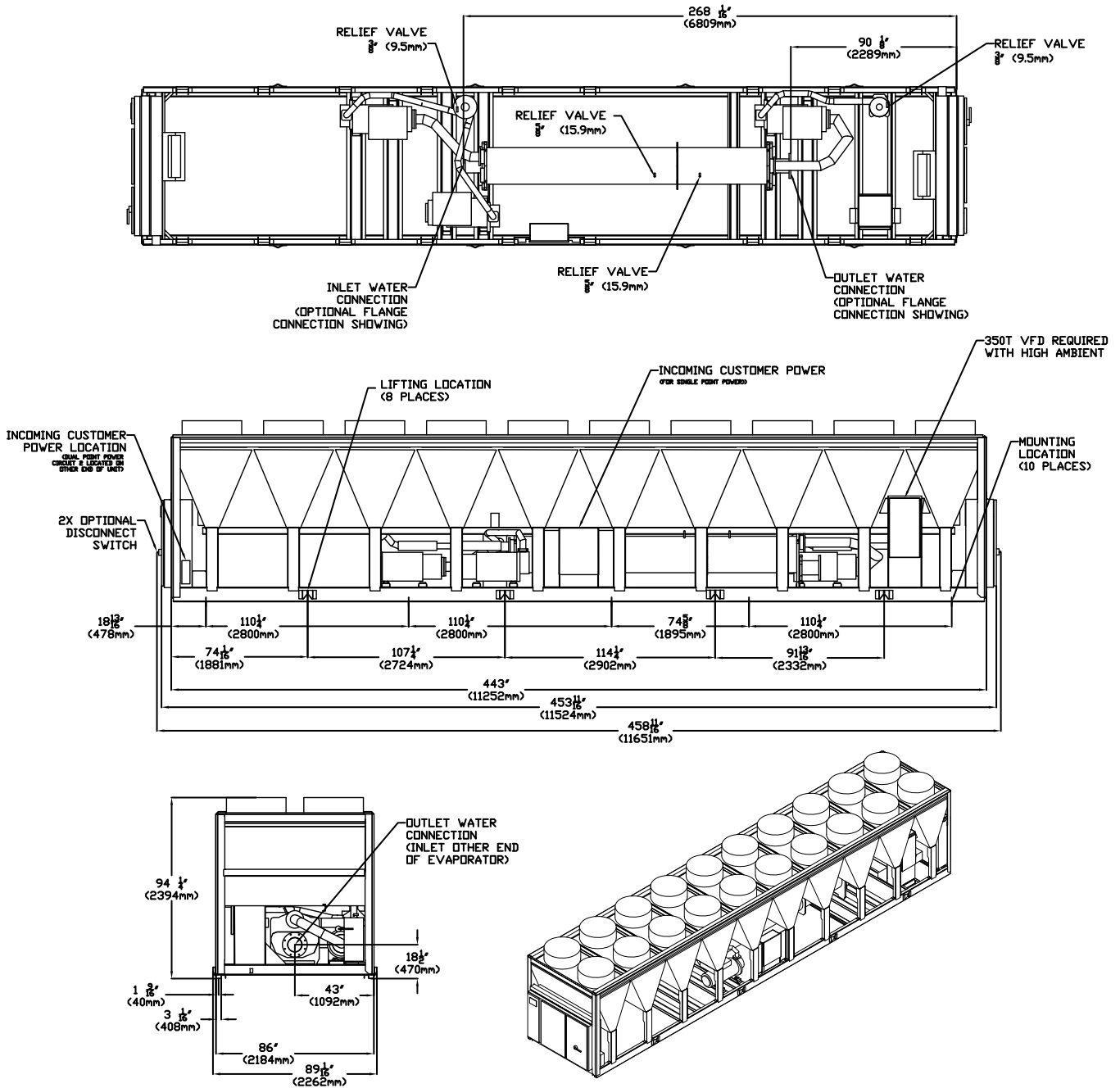
Figure 9. RTAF unit dimensions — 310, 350, 390 ton
