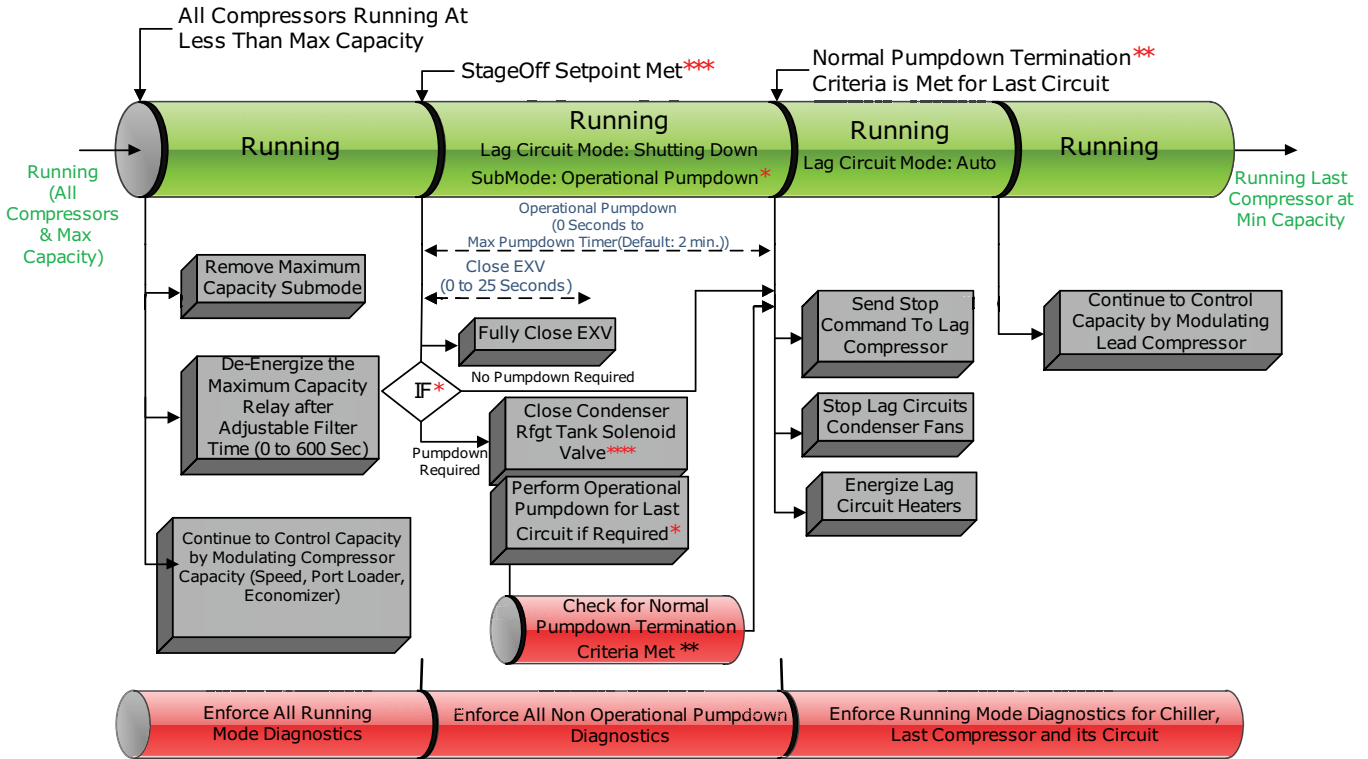
Figure 60. Sequence of events: unloading unstaging
