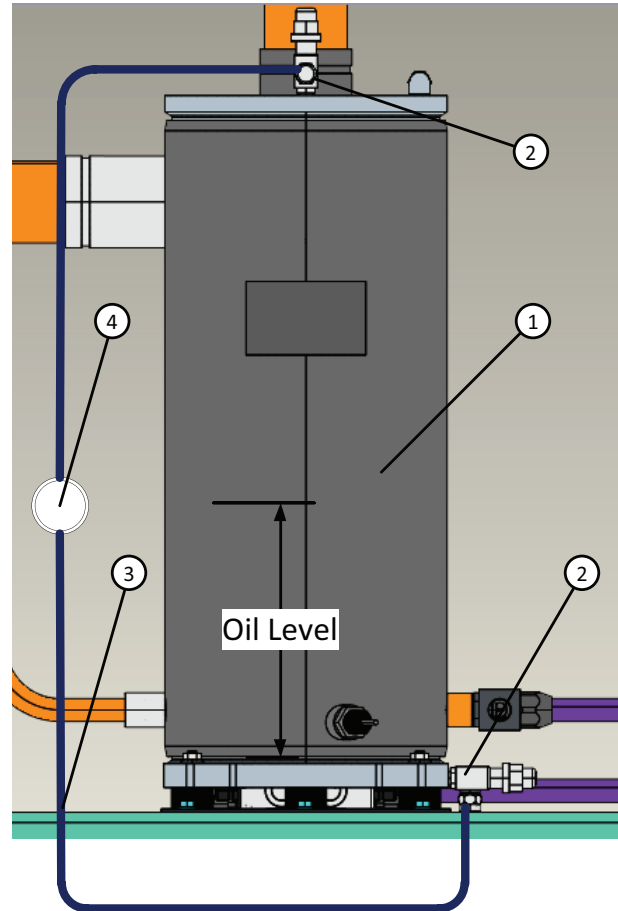
Figure 65. Oil sump level check
