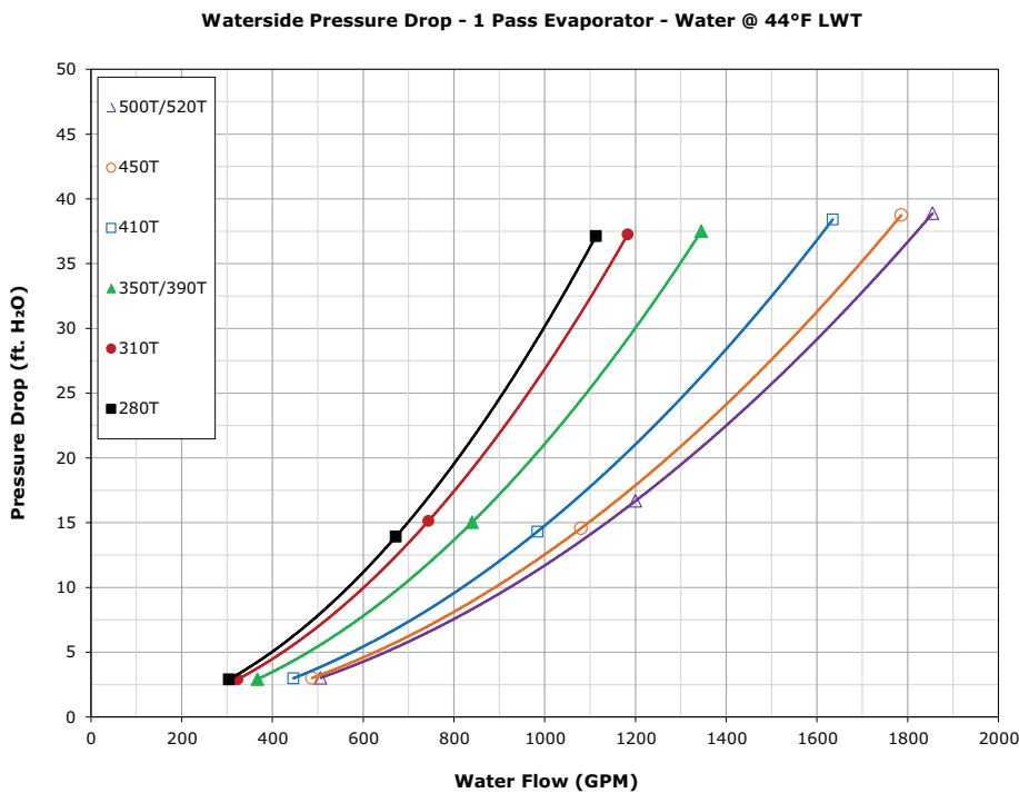
Figure 30. Evaporator water pressure drop — 280 to 520 tons, 1-pass without turbulators
