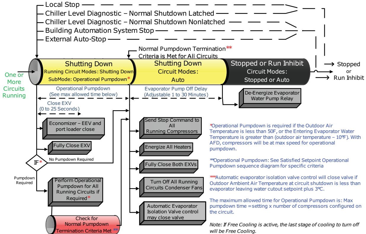
Figure 61. Sequence of events: normal shutdown to stopped or run inhibit
