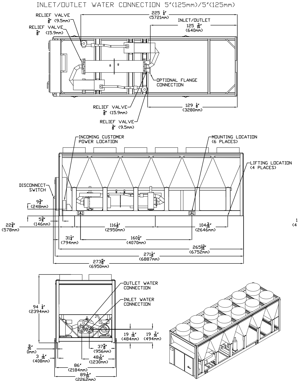
Figure 5. RTAF unit dimensions — 150, 170, 180 ton
