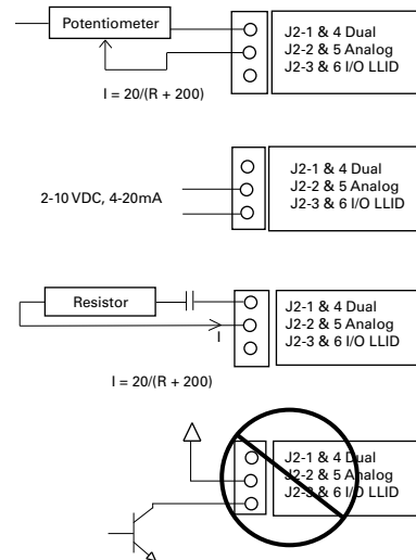
Figure 49. Wiring examples for EDLS and ECWS
