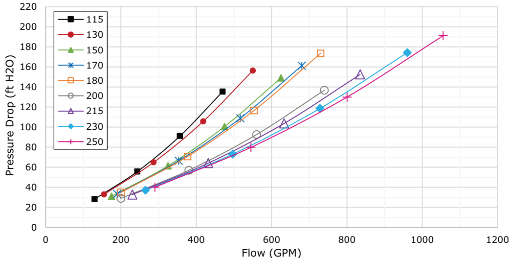
Figure 42. Evaporator water pressure drop, 35% propylene glycol, free-cooling on — 280 to 500 tons, 1-pass without turbulators
