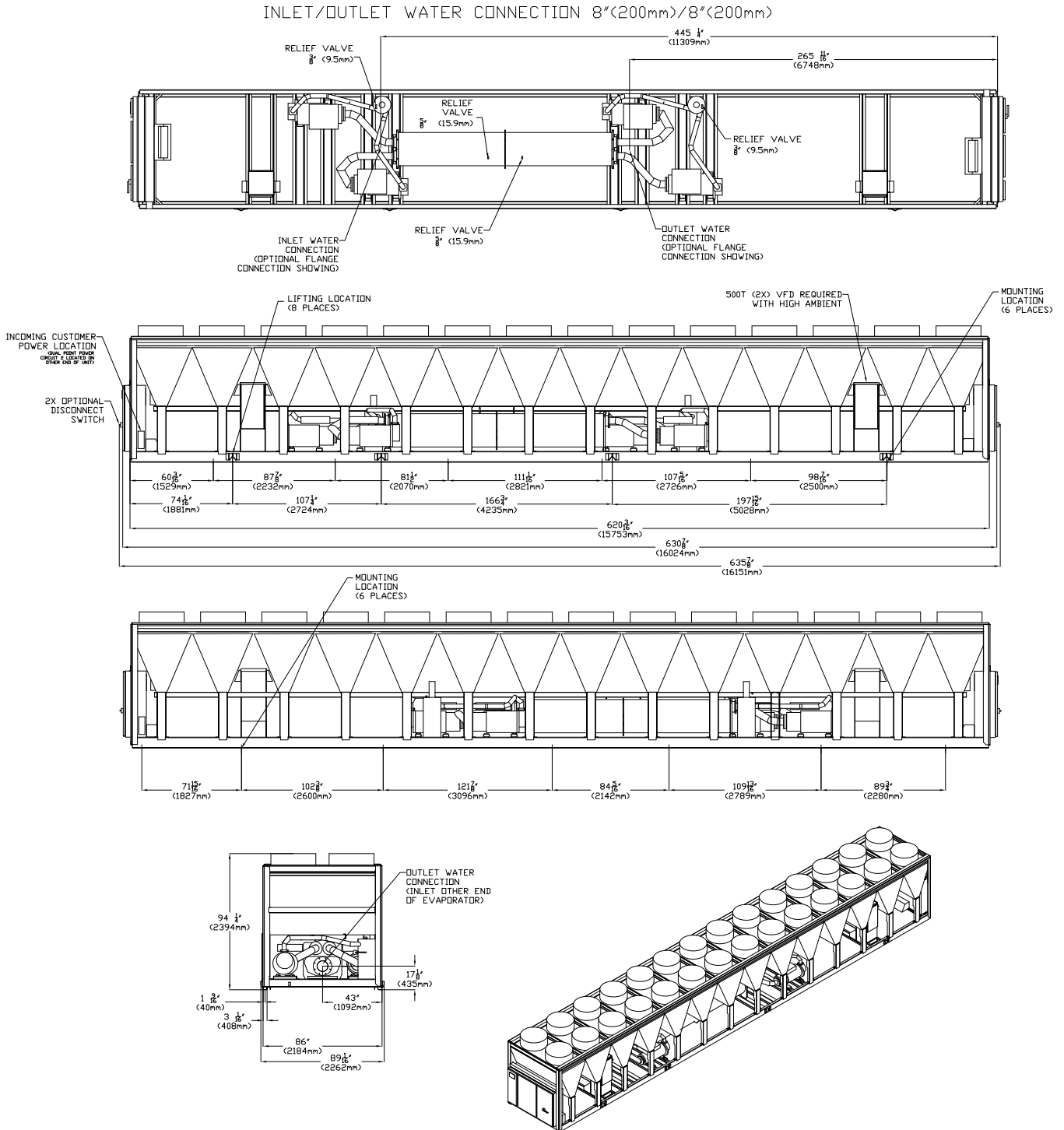
Figure 11. RTAF unit dimensions — 450, 500, 520 ton
