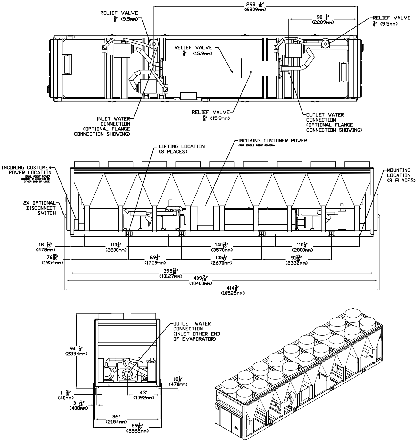
Figure 8. RTAF unit dimensions — 280 ton
