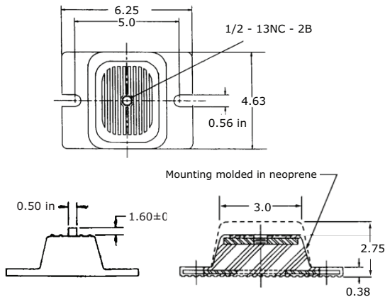
Figure 23. Elastomeric isolator
