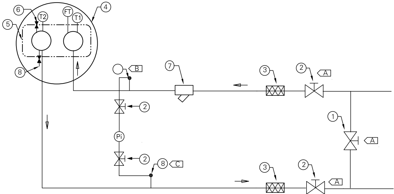
Figure 27. Evaporator water piping
