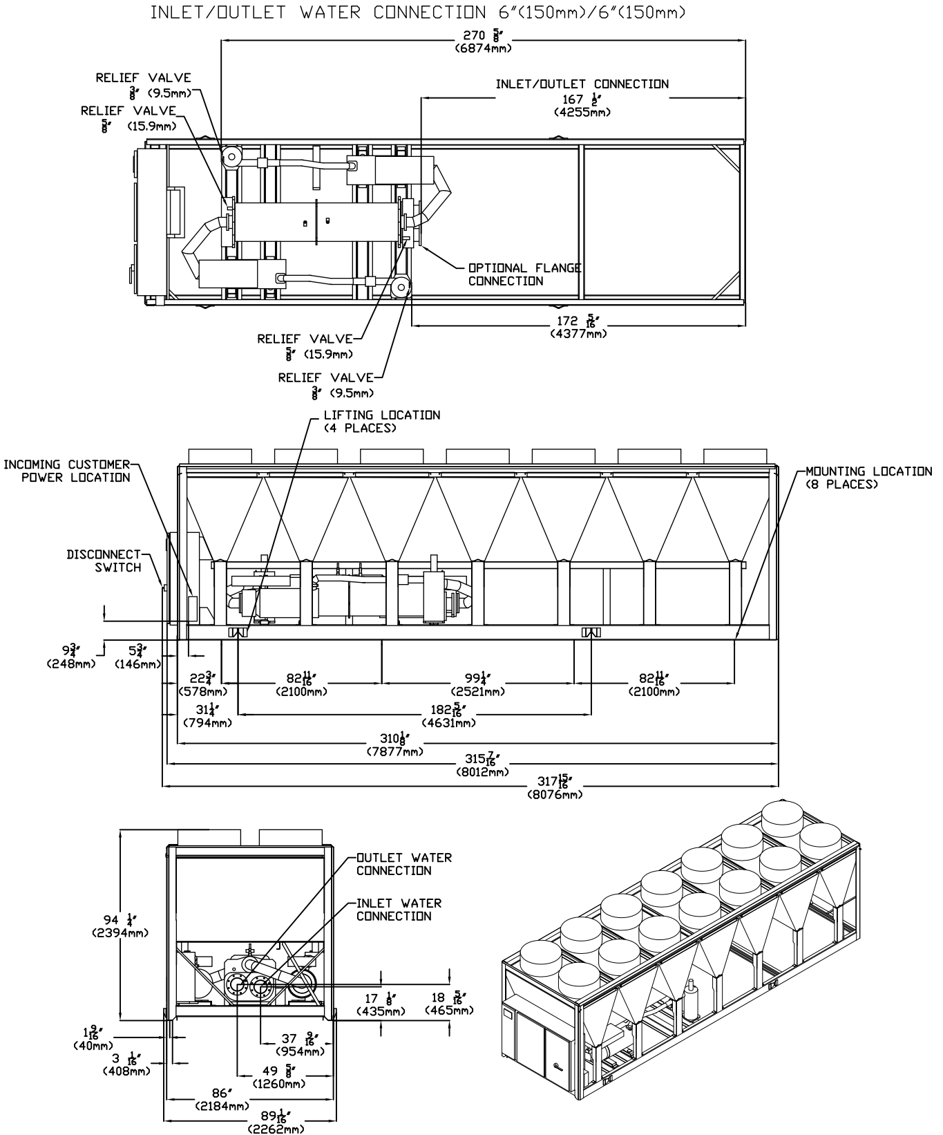
Figure 6. RTAF unit dimensions — 200, 215 ton
