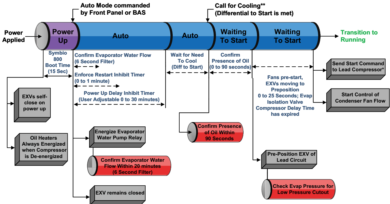
Figure 55. Sequence of events: power up to starting
