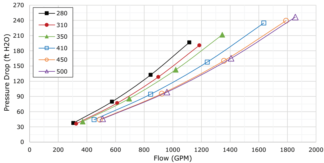
Figure 46. Evaporator water pressure drop, 35% propylene glycol, free-cooling on — 280 to 500 tons, 1-pass with turbulators
