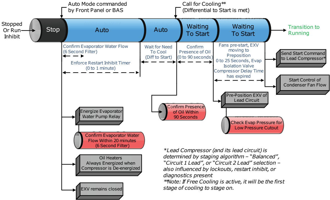
Figure 56. Sequence of events: stopped to starting
