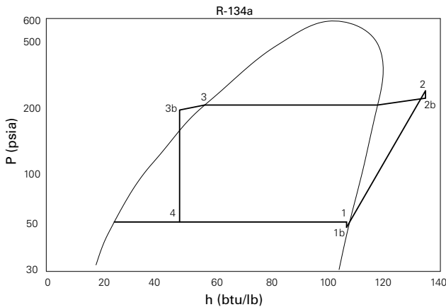
Figure 51. Pressure-enthalpy diagram
