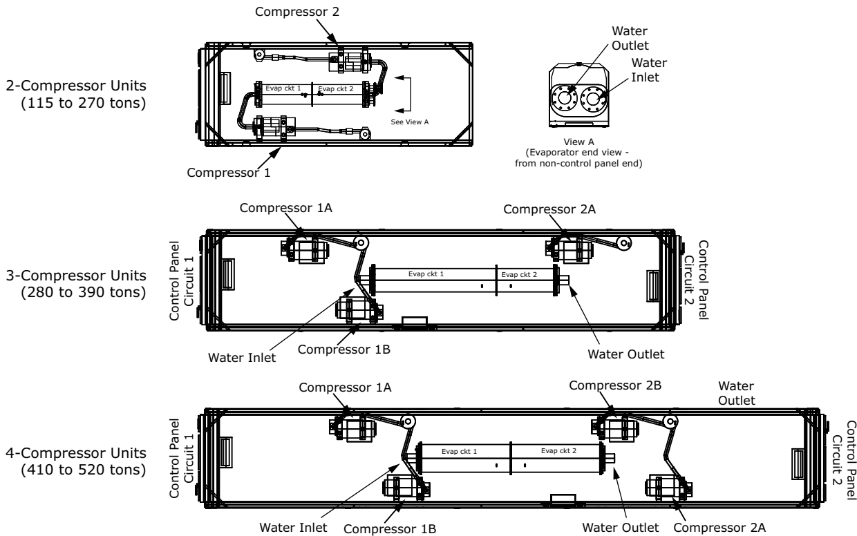
Figure 2. Evaporator piping and compressor locations
