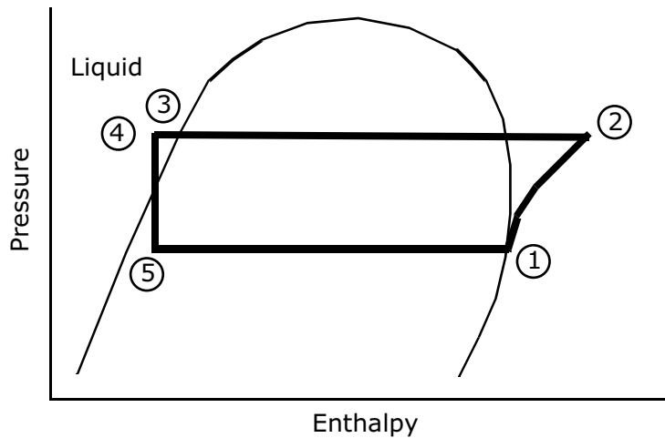
Figure 29. Pressure enthalpy curve
