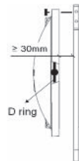
Figure 33. Waterbox removal - slide out, install safety hoist ring
