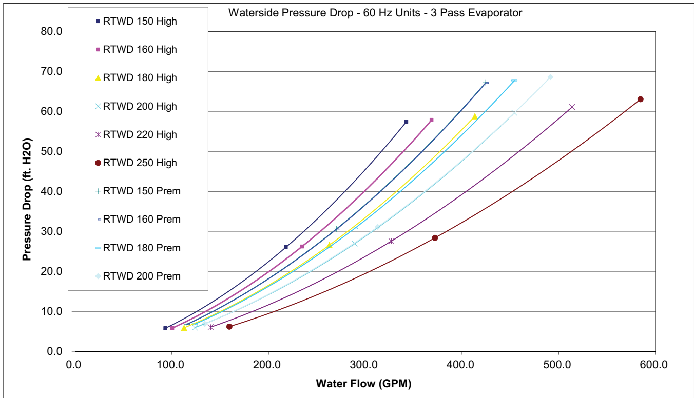
Figure 21. Evaporator pressure drop curves - 3 pass, 60 Hz - RTWD
