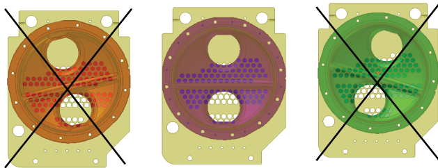
Figure 16. RTWD waterboxes
