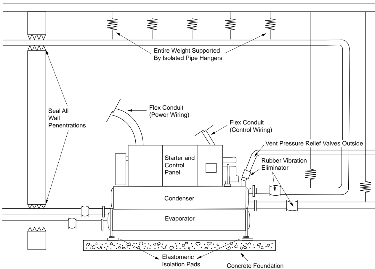
Figure 15. RTWD installation
