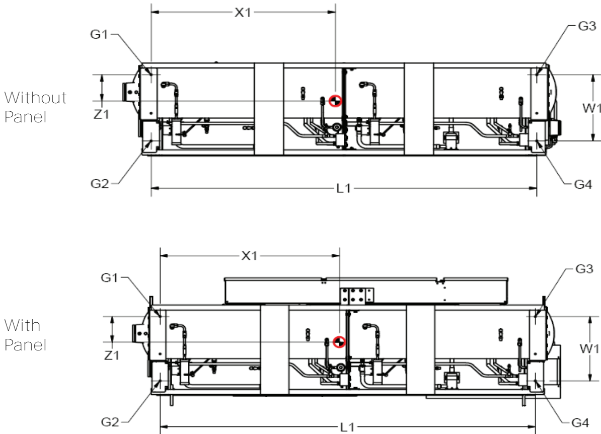
Figure 13. Mounting point locations and weights – RTWD Premium efficiency (all), RTWD High efficiency: 150 – 250T (60 Hz)
