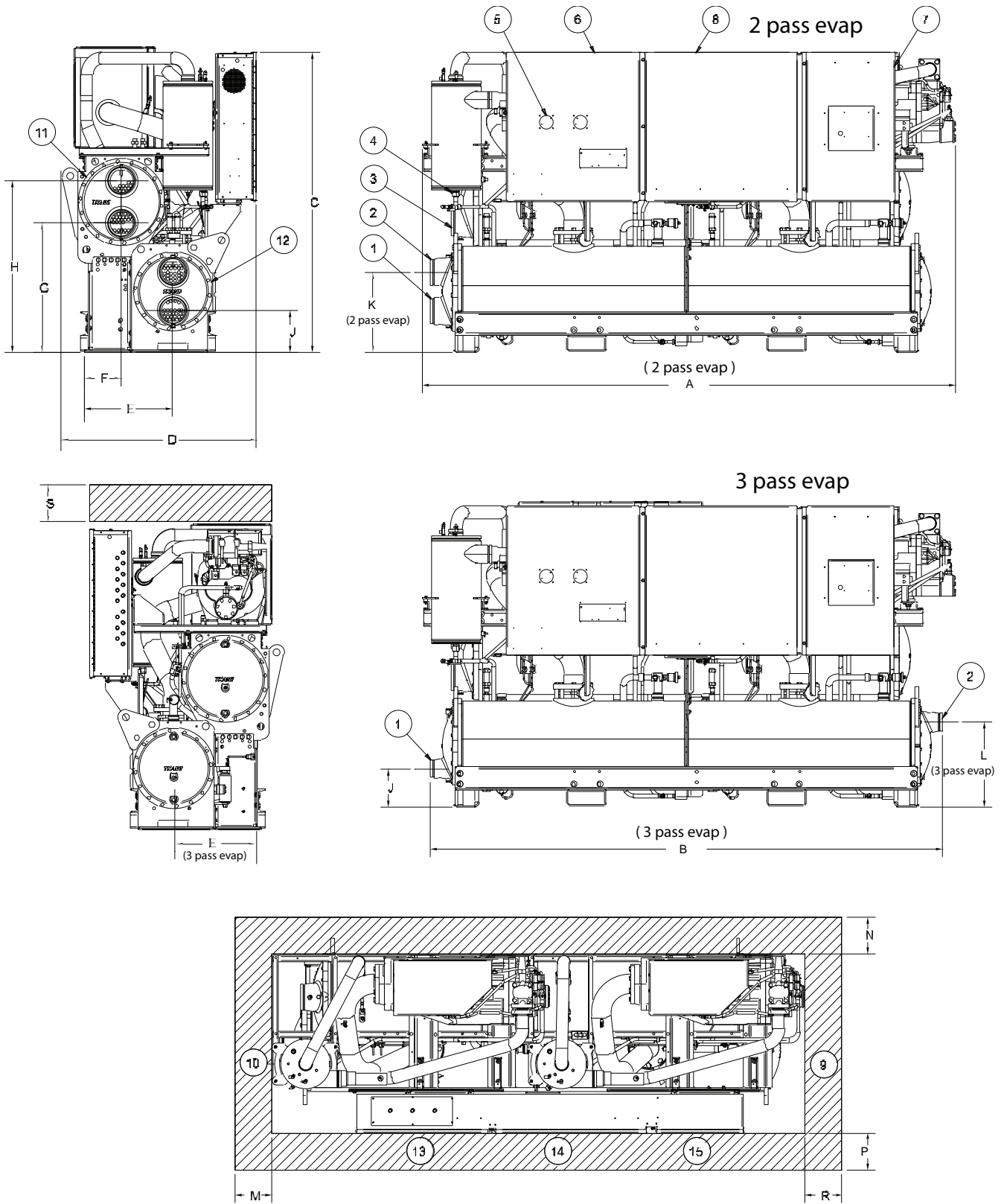
Figure 2. RTWD, 150 to 250 tons, 60 Hz
