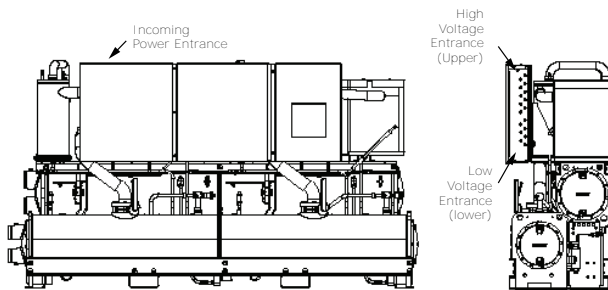
Figure 25. Power entrance
