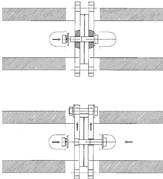
Figure 5. Recesses in the header insulation facilitate the assembly of connecting hardware
