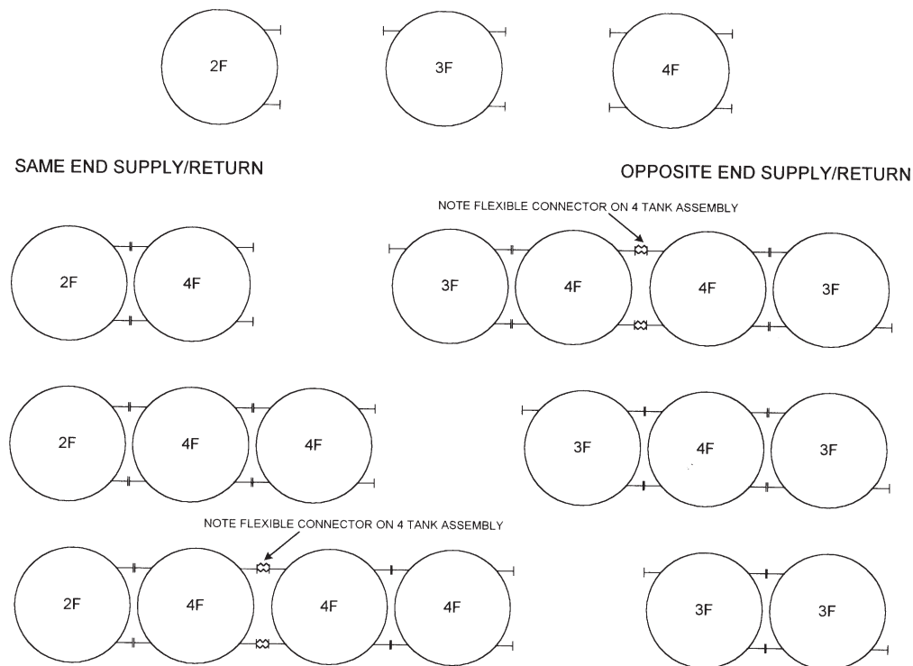
Figure 4. Assembly options for “C” model tanks
