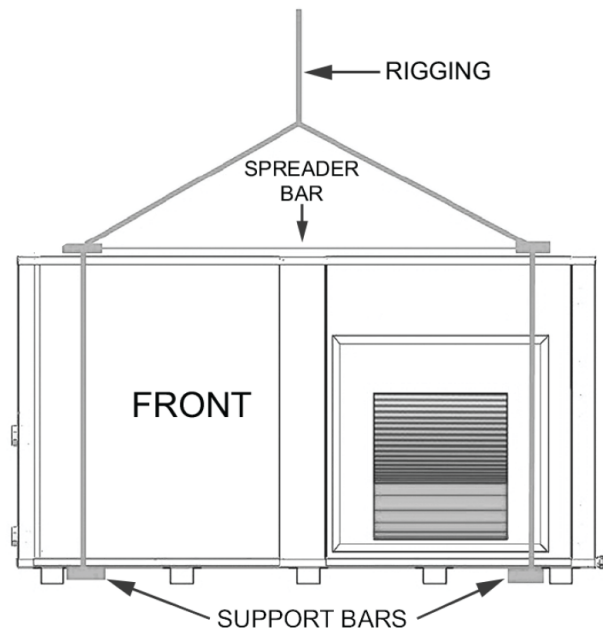
Figure 4. Rigging and hoisting unit
