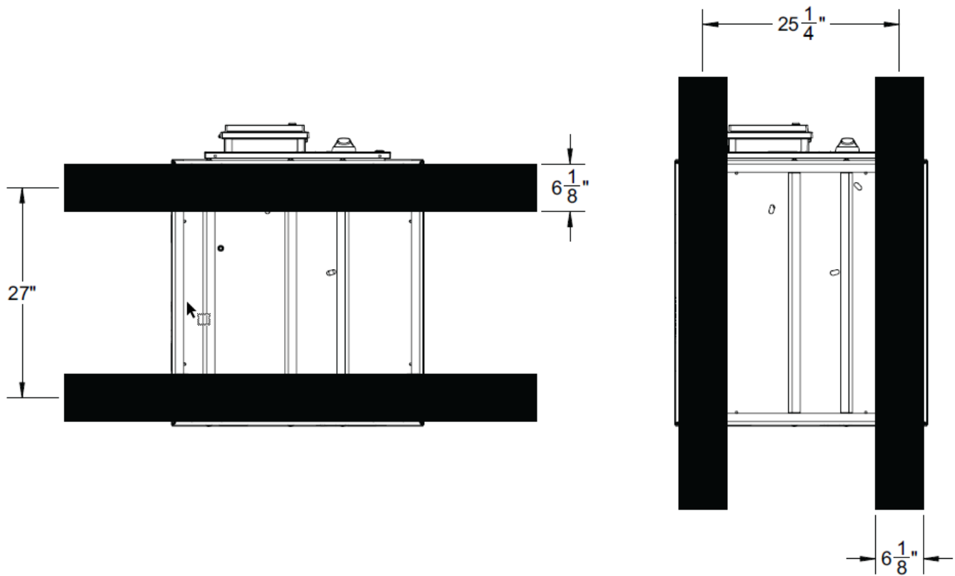
Figure 7. T270WM mounting rails position and widths
