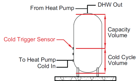
Figure 13. Single-pass tank sensor location
