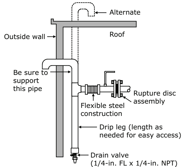
Figure 1. Rupture disc relief piping arrangement
