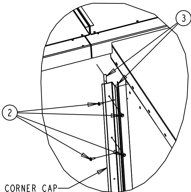
Figure 89. Pipe cabinet installation details
