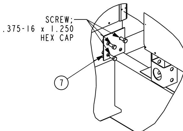
Figure 82. Pipe cabinet installation details
