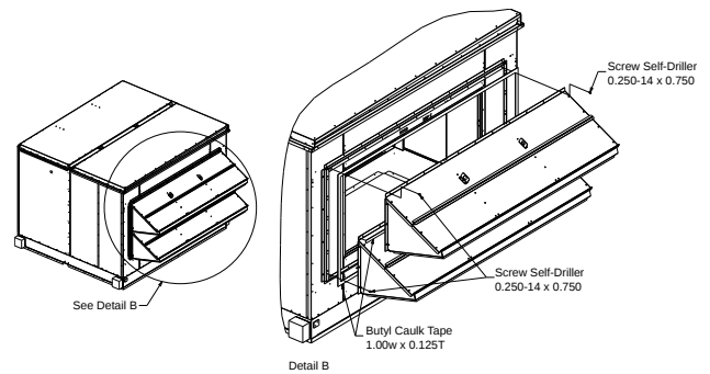
Figure 101. Standard inlet hood installation
