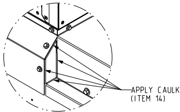
Figure 65. Internal width 27.5 to 96 in. (des seq M or later), non-hurricane units
