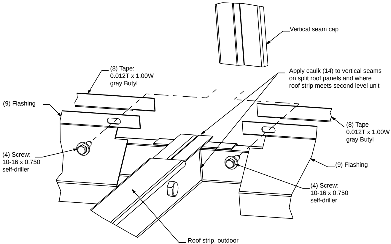
Figure 58. Flashing installation for perpendicular-to-airflow piece if second level of unit is shorter than first level
