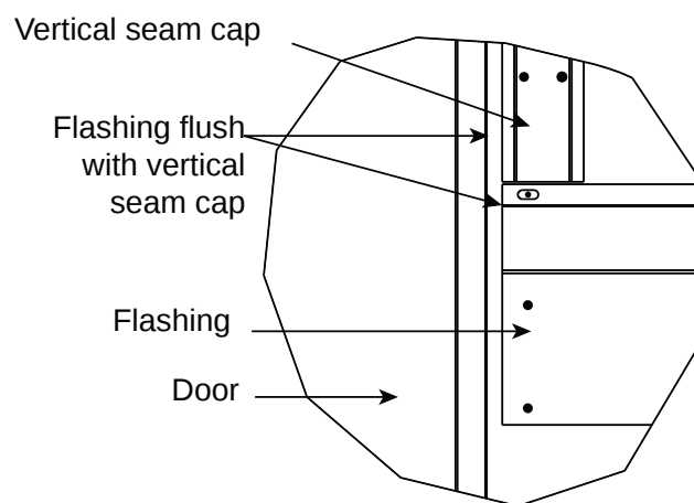
Figure 52. Side flashing installation with full height doors
