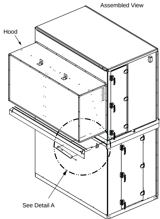
Figure 98. Stacked unit assembly – angle and guard installation
