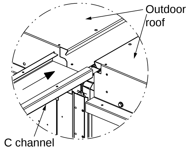
Figure 34. Slide c-channel
