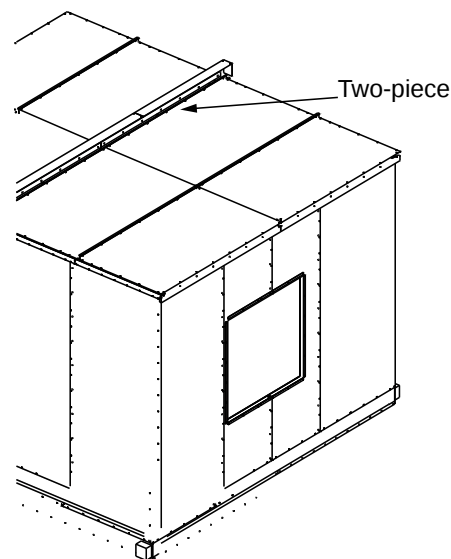
Figure 23. Double roof
