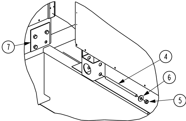
Figure 83. Pipe cabinet installation details
