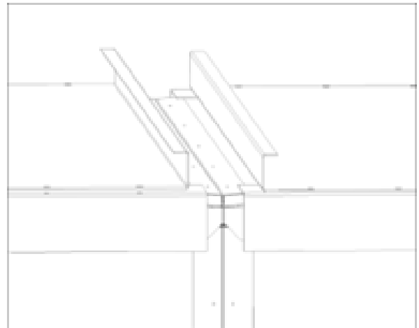
Figure 18. Corner detail
