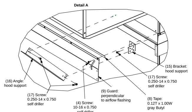
Figure 98. Stacked unit assembly – angle and guard installation
