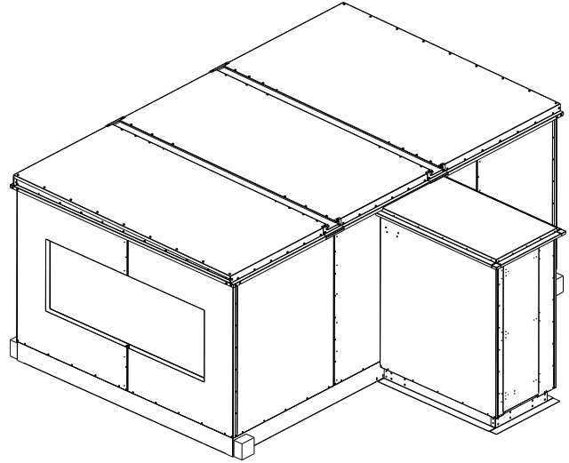
Figure 72. Pipe cabinet install before corner cap
