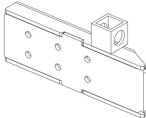
Figure 11. LH wedge block assembly
