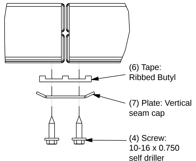
Figure 15. Seam cap installation – shipping split seams
