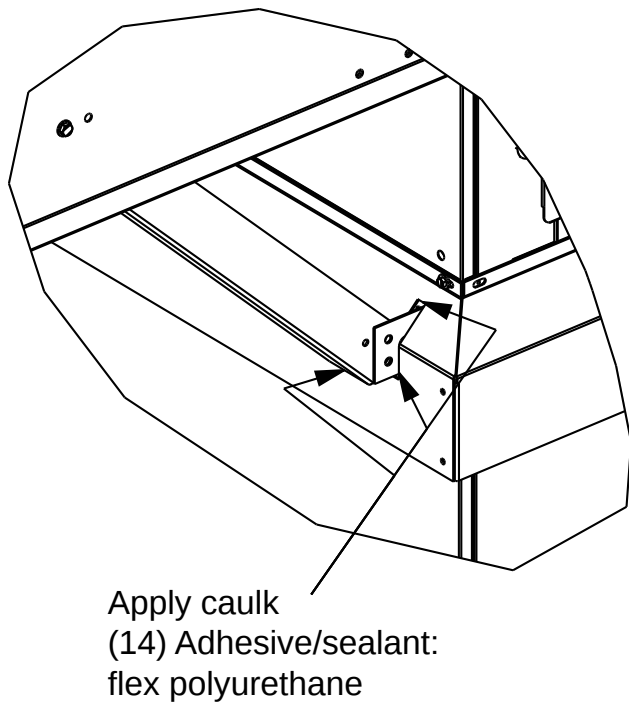
Figure 99. Stacked unit assembly - apply caulk
