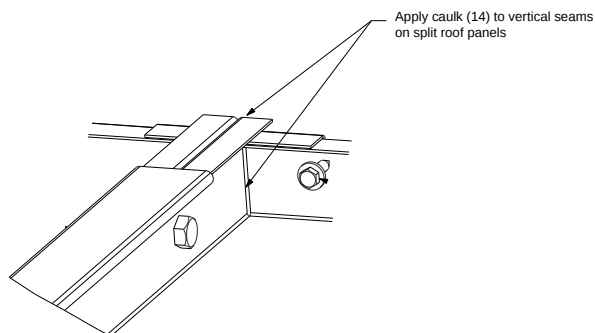
Figure 27. Vertical gap caulk
