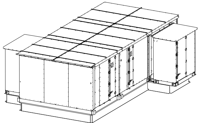
Figure 77. Pipe cabinet installation, unit sizes 3 to 35 (des seq L or earlier) and 40 to 120
