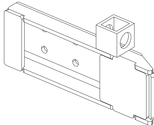
Figure 12. RH wedge block assembly
