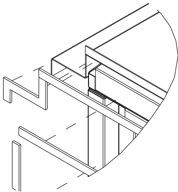
Figure 75. Pipe cabinet installation, unit sizes 3 to 35 (des seq M or later)
