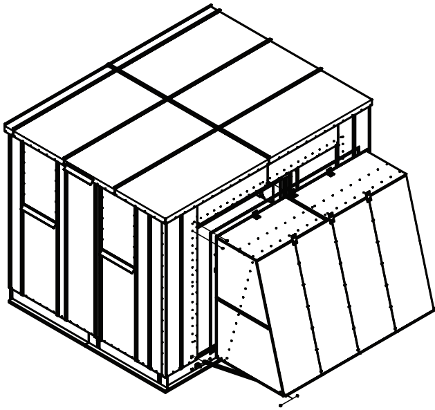
Figure 96. Inlet hurricane and exhaust hood installation
