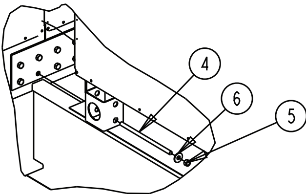
Figure 88. Pipe cabinet installation details
