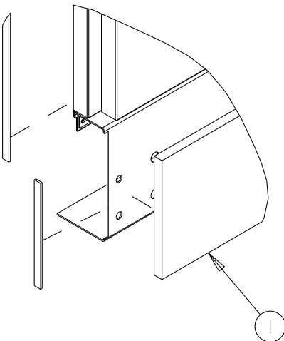
Figure 75. Pipe cabinet installation, unit sizes 3 to 35 (des seq M or later)
