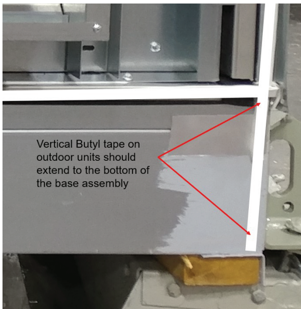
Figure 6. Install butyl tape on outdoor bases
