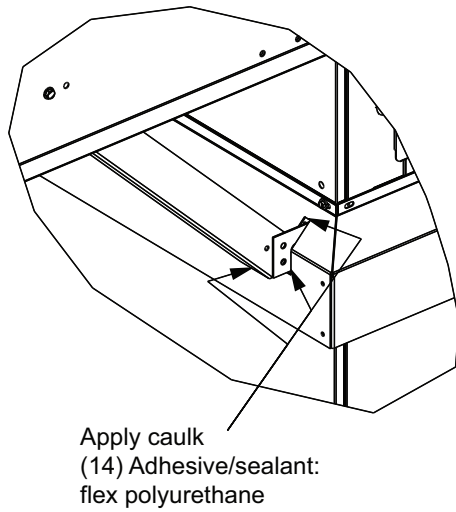
Figure 99. Stacked unit assembly - apply caulk
