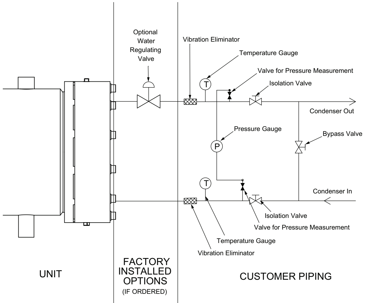
Figure 4. Condenser piping schematic
