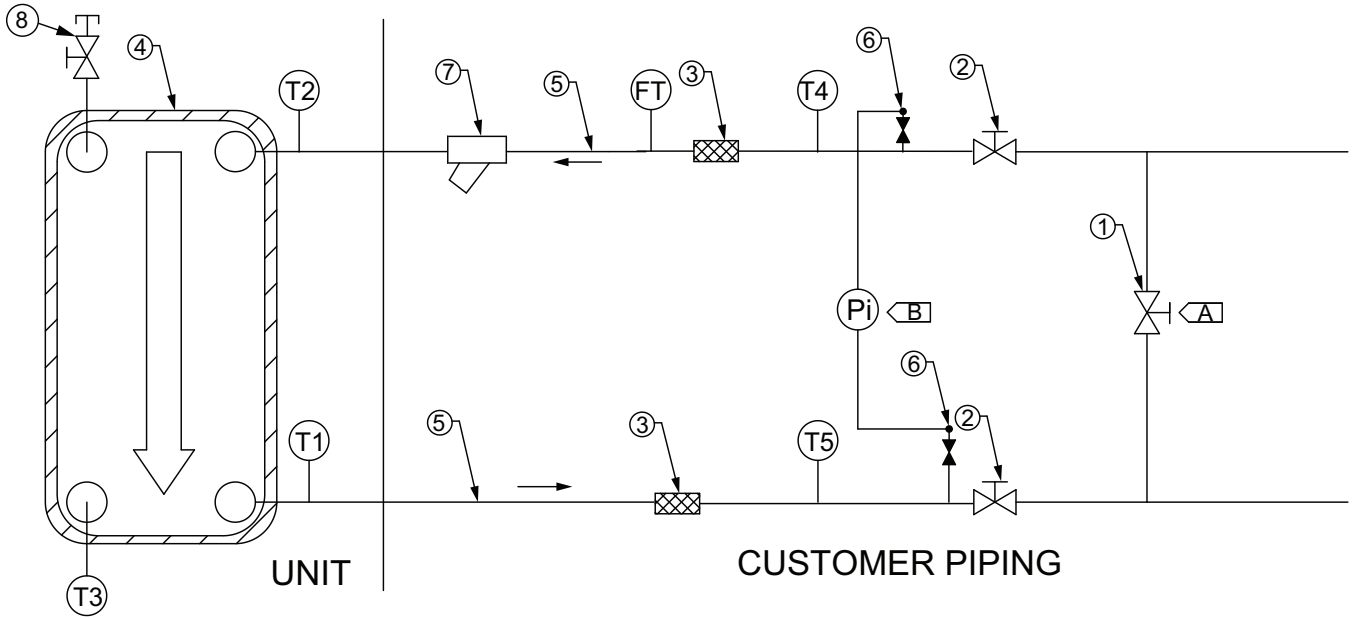
Figure 3. Chilled water piping schematic
