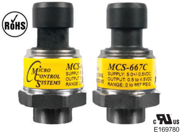
Part # MCS-667C-xx*
