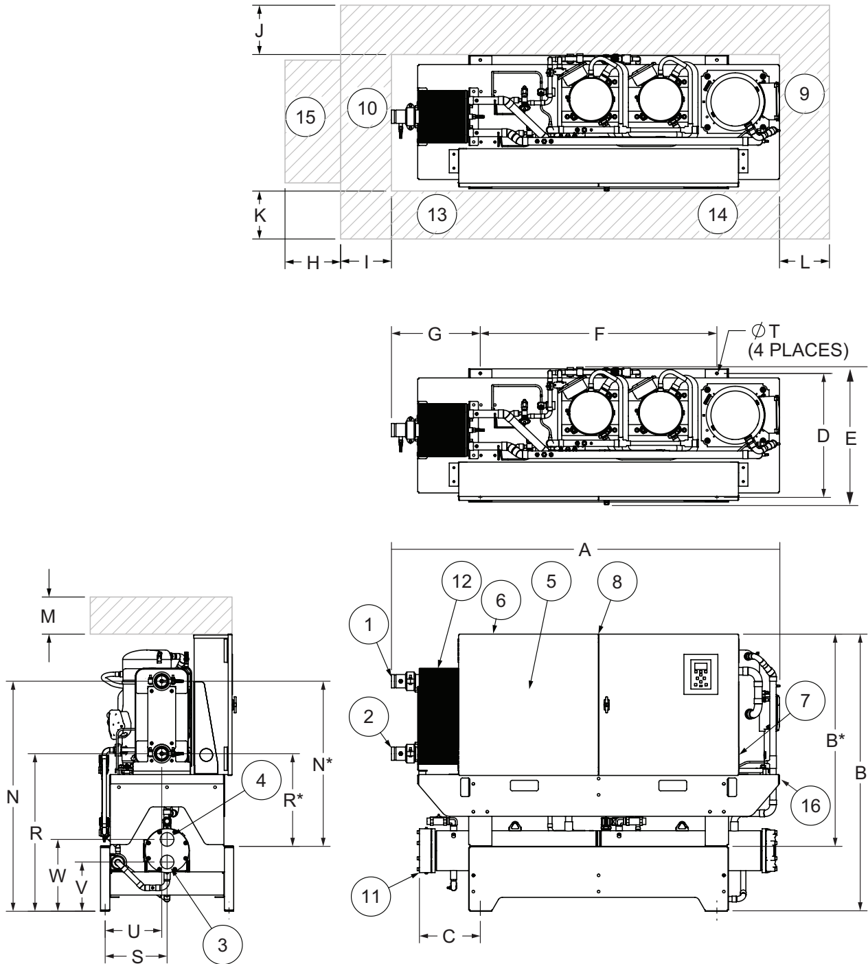
Figure 2. CGWR/CCAR 40 to 75 ton mechanical drawing
