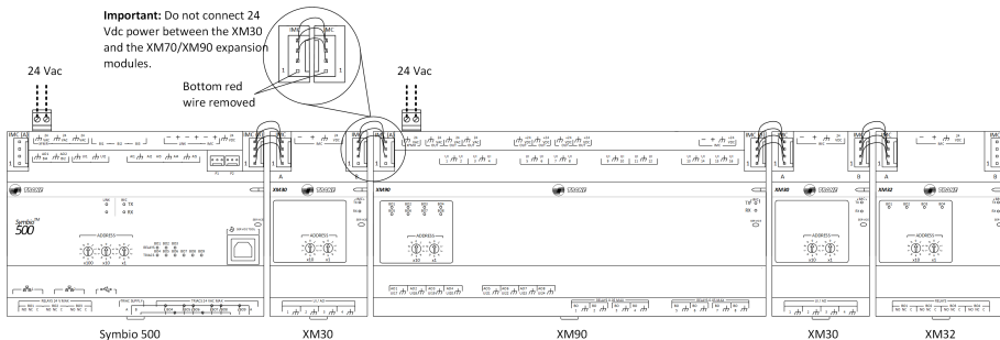
Figure 9. Symbio 500 application with an XM70/XM90 and multiple expansion modules
