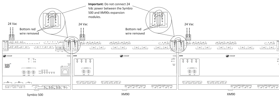
Figure 10. Symbio 500 application with two XM70/XM90 modules
