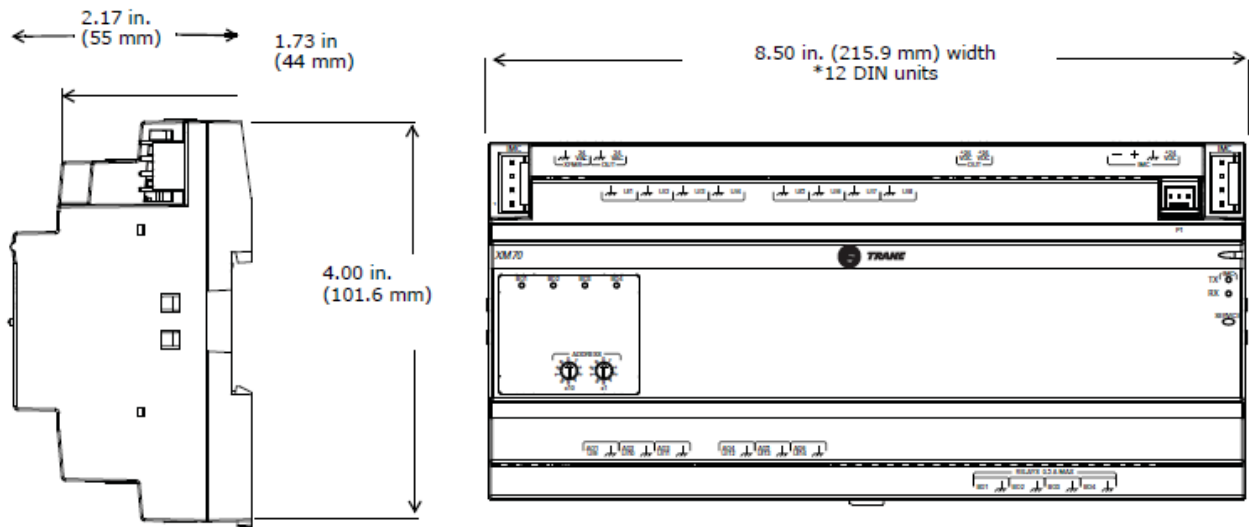
Figure 3. XM70/XM90 dimensions
