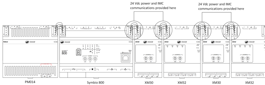
Figure 12. Symbio 800 application example with four expansion modules
