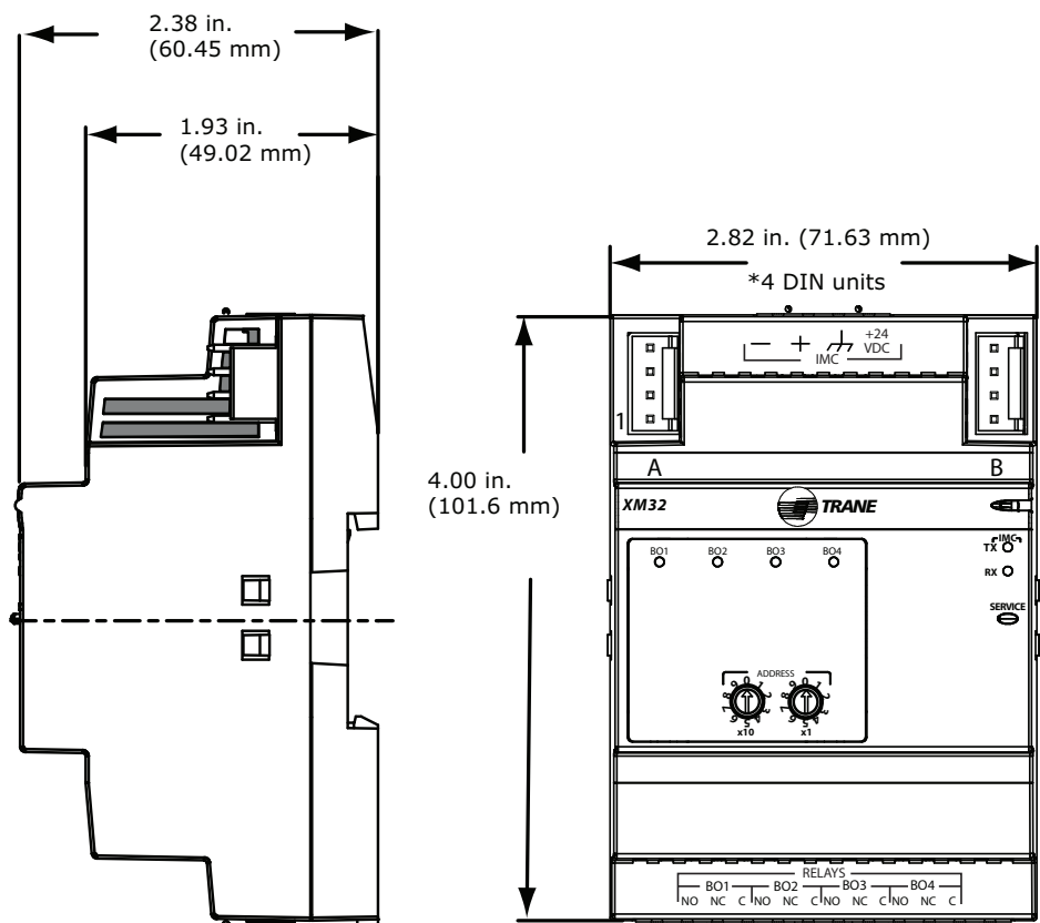
Figure 2. XM32 dimensions
