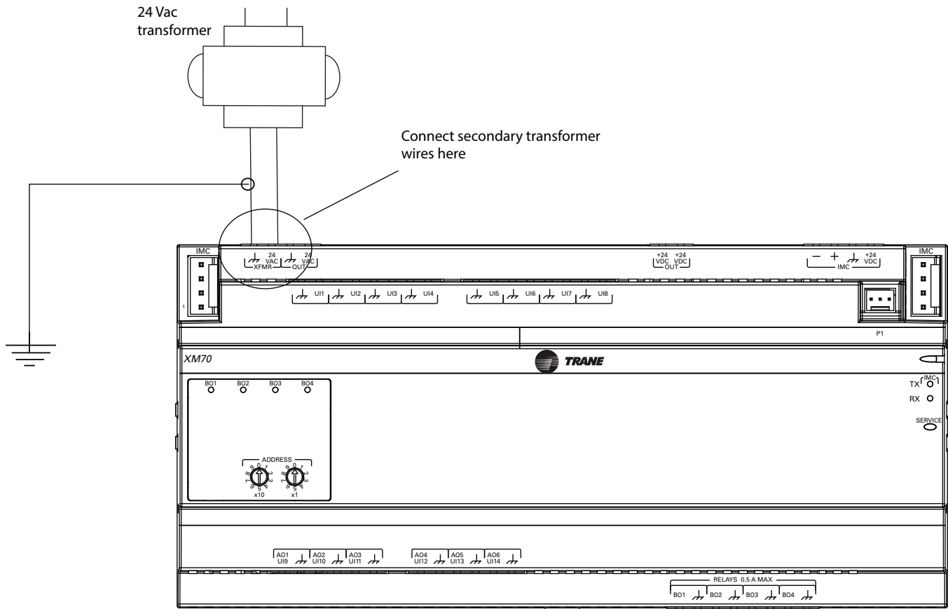
Figure 16. Wiring AC power
