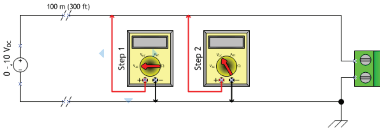
Figure 19. Voltage input
