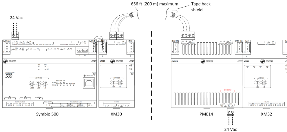
Figure 15. Remote mounting with the use of a PM014 power supply
