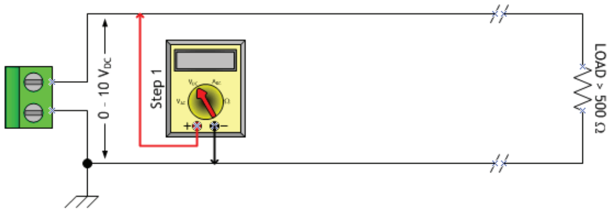
Figure 24. Voltage analog output
