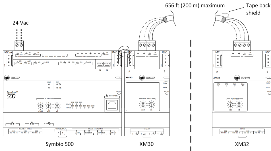
Figure 14. Mounting expansion modules remotely
