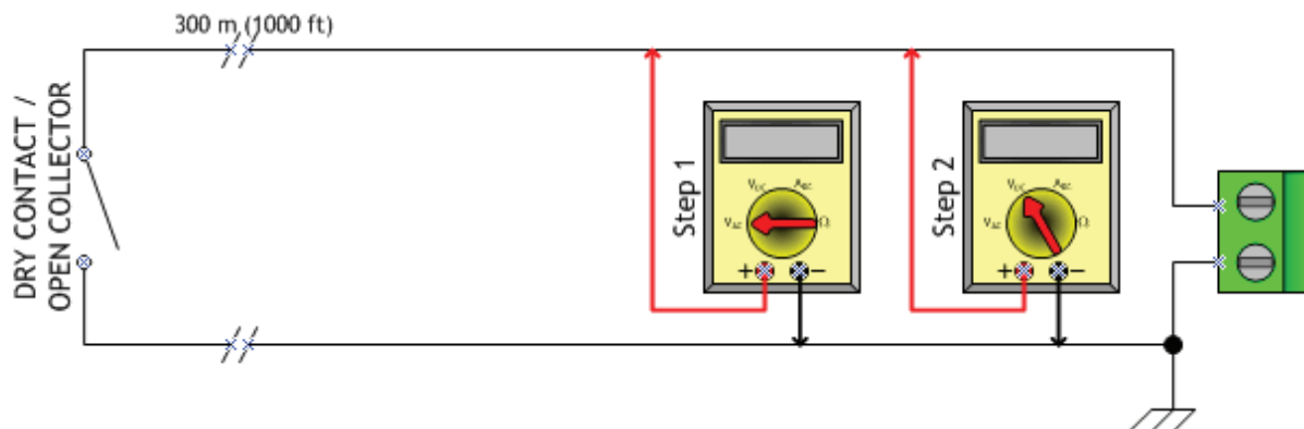
Figure 23. Binary input
