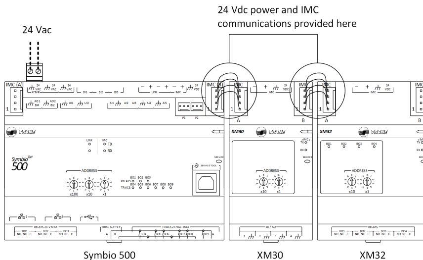
Figure 7. Example of a typical installation: two expansion modules and one Symbio 500 programmable controller
