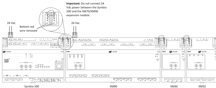
Figure 11. Symbio 500 application with XM70/XM90, XM32, and XM30 modules
