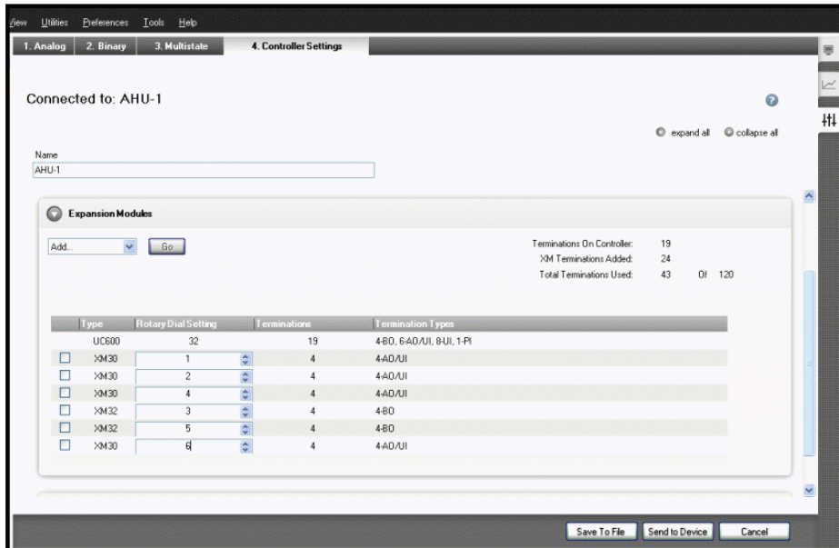
Figure 17. Expansion modules group box (Tracer TU)
