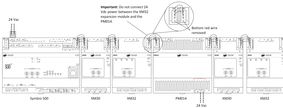
Figure 8. Applications requiring more than two expansion modules
