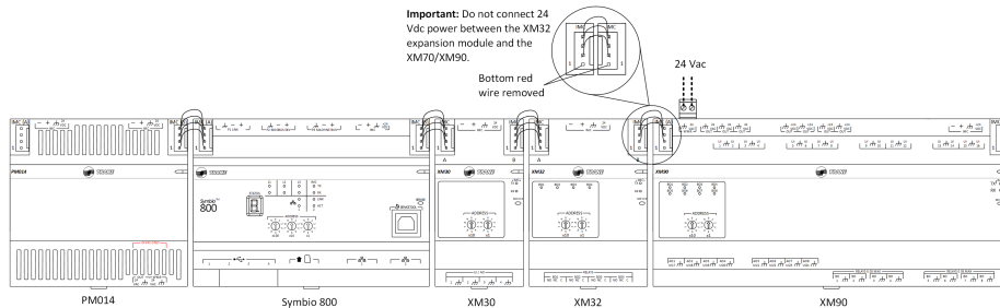
Figure 13. Symbio 800 application with XM70/XM90 expansion modules
