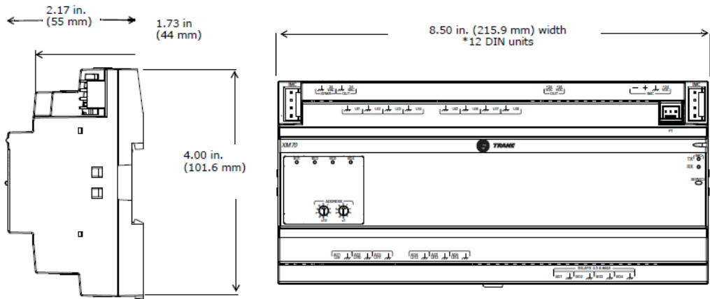
Figure 3. XM70/XM90 dimensions
