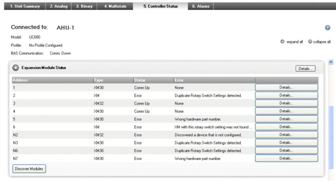
Figure 16. Possible expansion module errors (Tracer TU)
