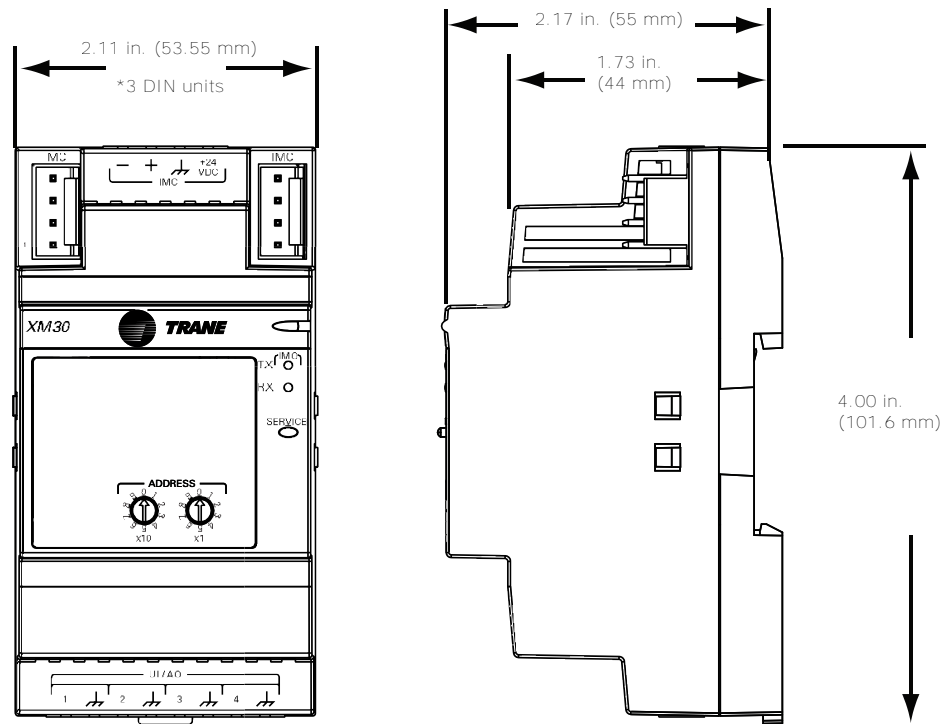
Figure 1. XM30 dimensions
