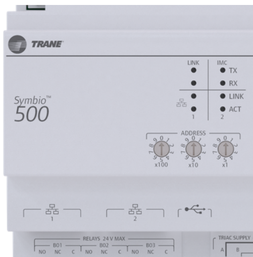
Figure 7. Symbio 500 Ethernet ports
