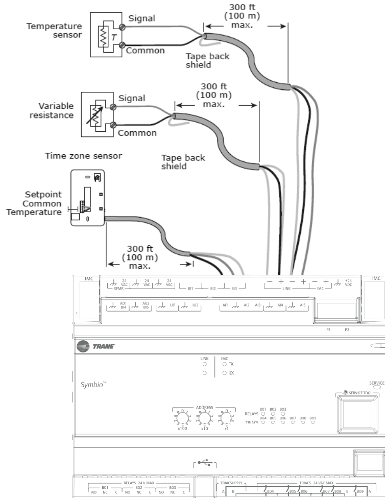
Figure 13. Variable resistance analog inputs
