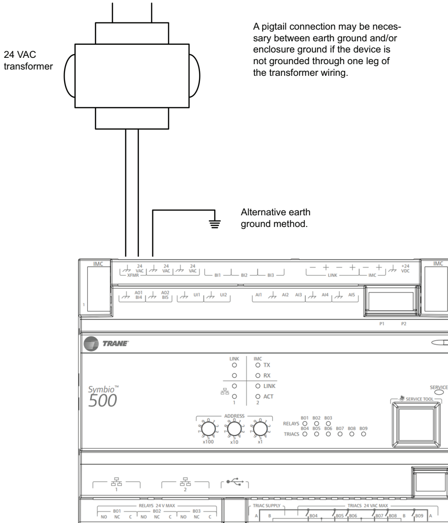
Figure 8. Symbio 500 transformer
