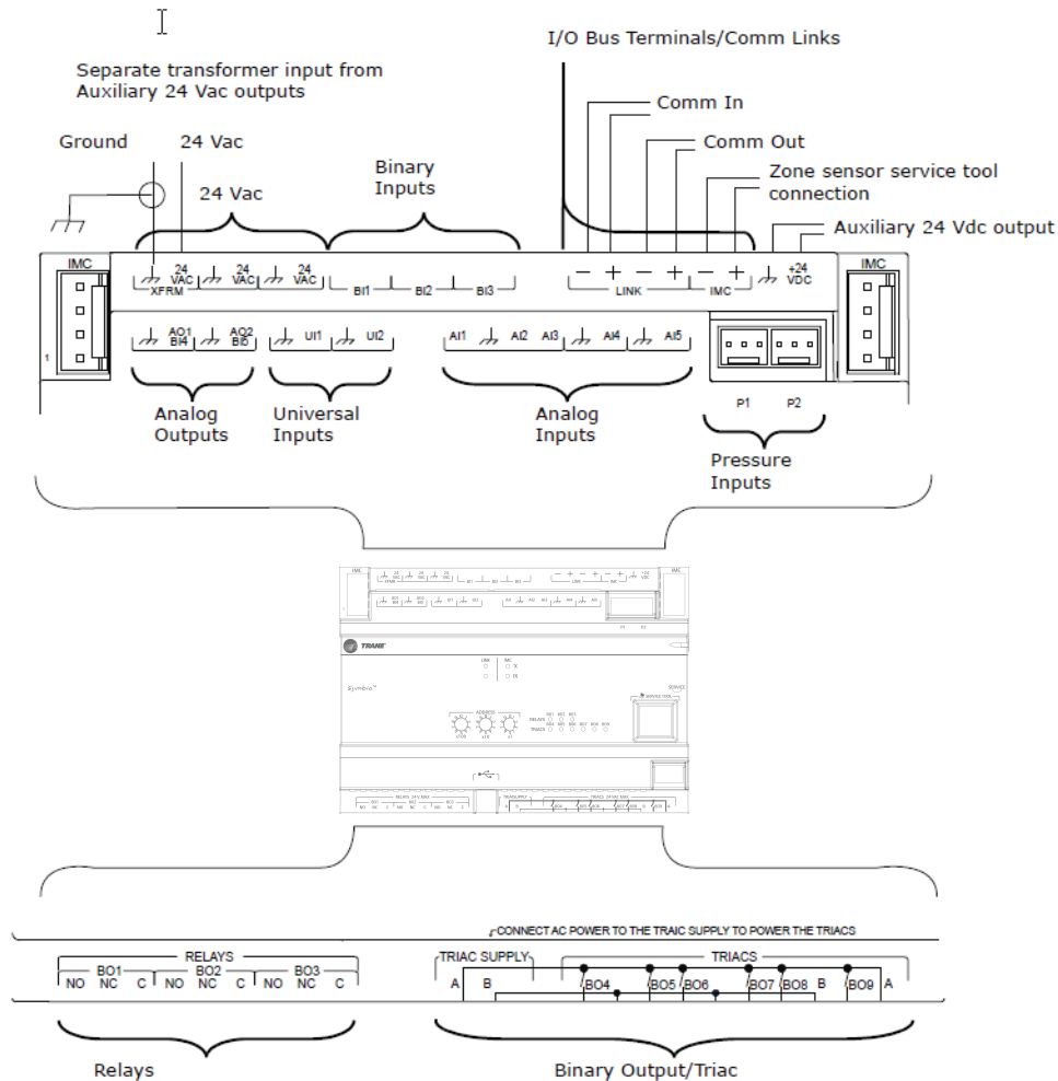
Figure 9. Terminal locations
