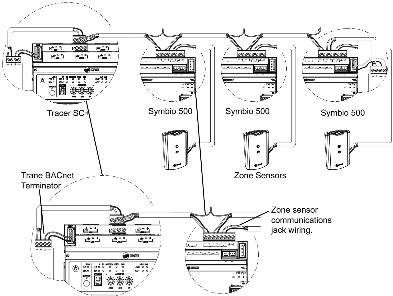
Figure 4. BACnet MS/TP link wiring — zone sensors are not required with this application
