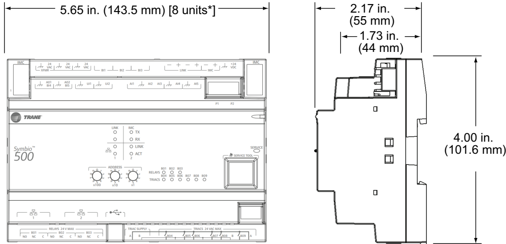
Figure 2. Controller dimensions
