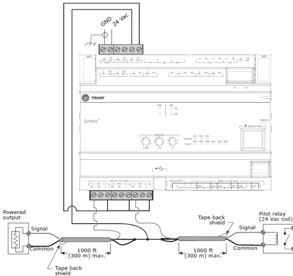
Figure 15. Dry contact/binary outputs
