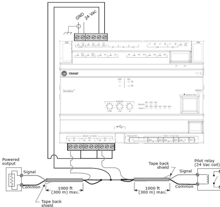
Figure 15. Dry contact/binary outputs
