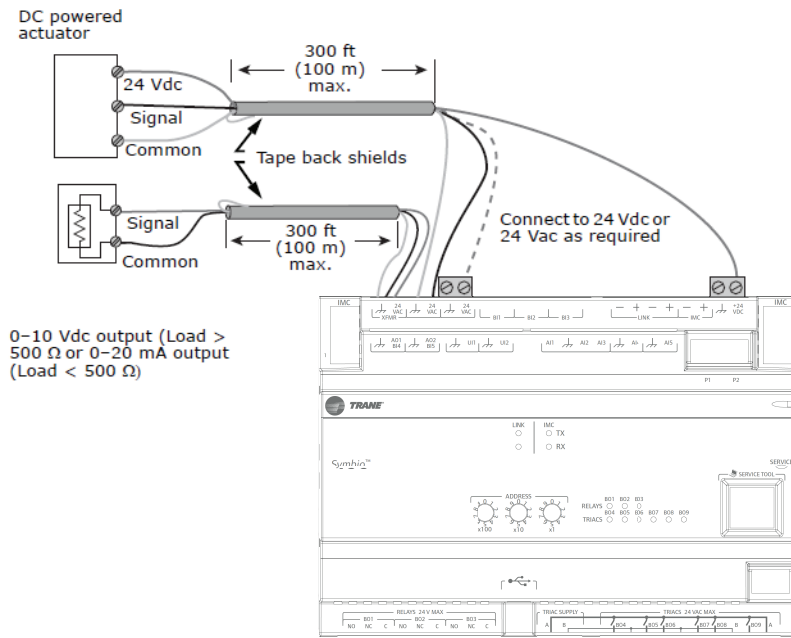
Figure 14. Analog outputs
