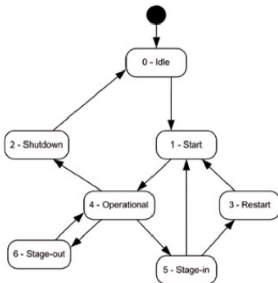
Figure 32. Chiller operational states flow chart
