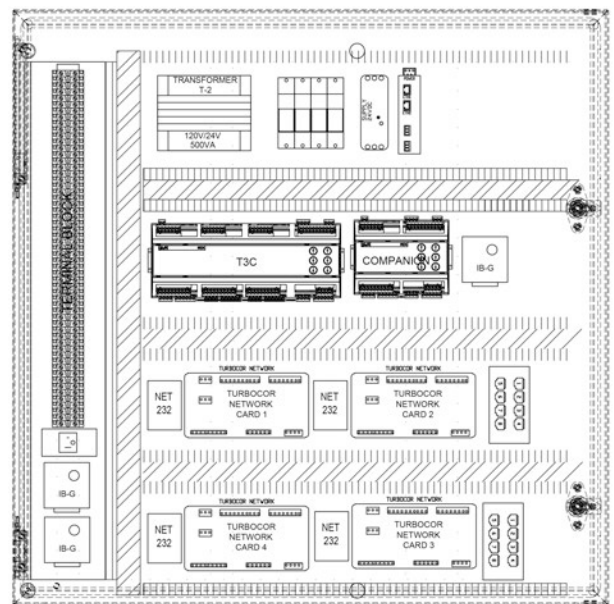
Figure 6. Control panel
