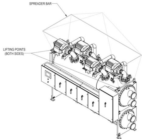
Figure 3. Recommended chiller rigging assembled unit
