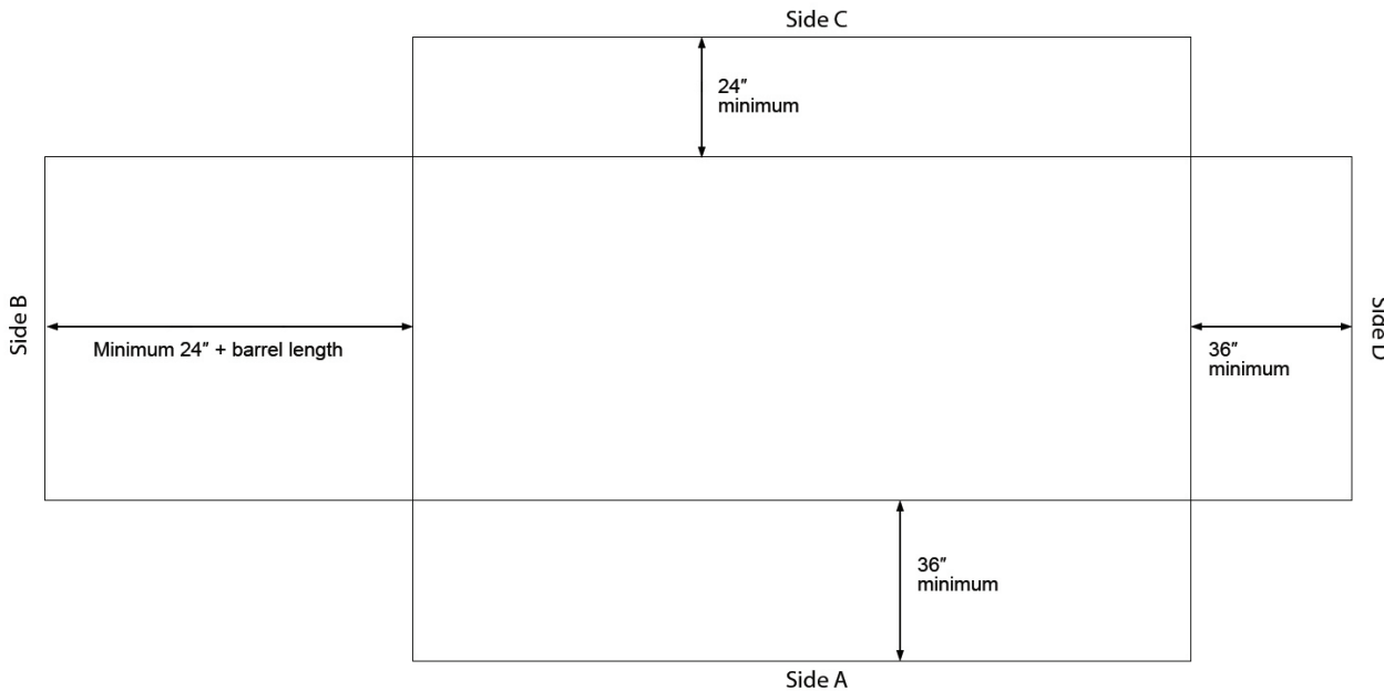
Figure 2. Recommended chiller clearances
