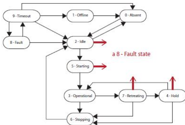
Figure 33. Compressor control states flow chart
