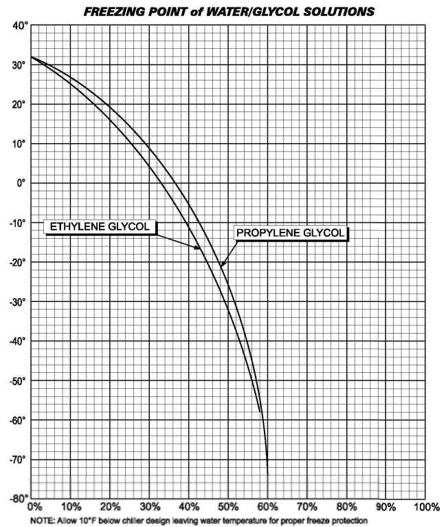
Figure 31. Water/Glycol concentration freezing points (in degrees Fahrenheit)
