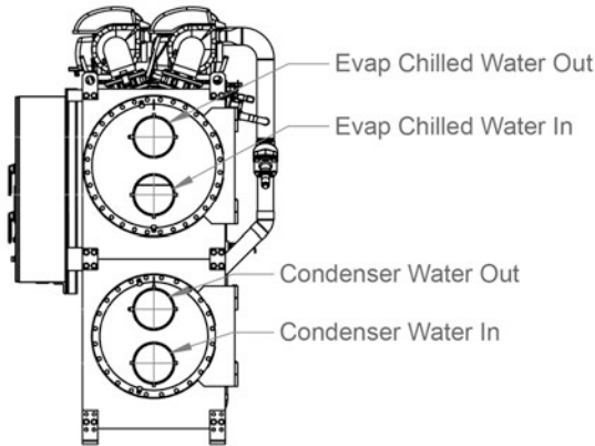
Figure 4. Recommended chiller piping
