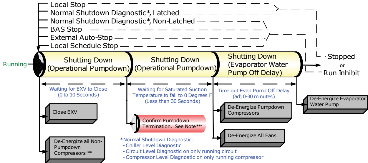
Figure 37. Sequence of operation: normal shutdown to stopped or run inhibit
