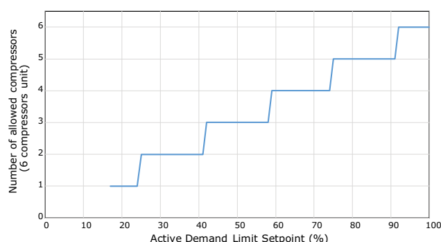
Figure 32. Demand limit setpoint via 4–20 mA signal
