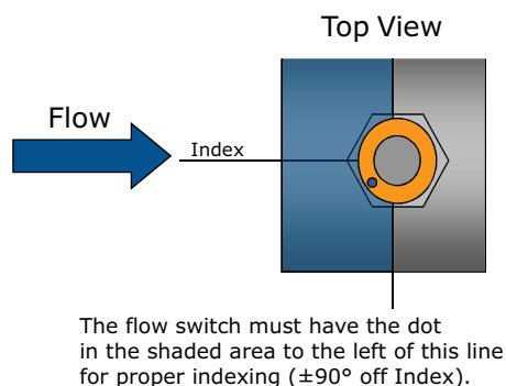
Figure 9. Proper flow switch indexing
