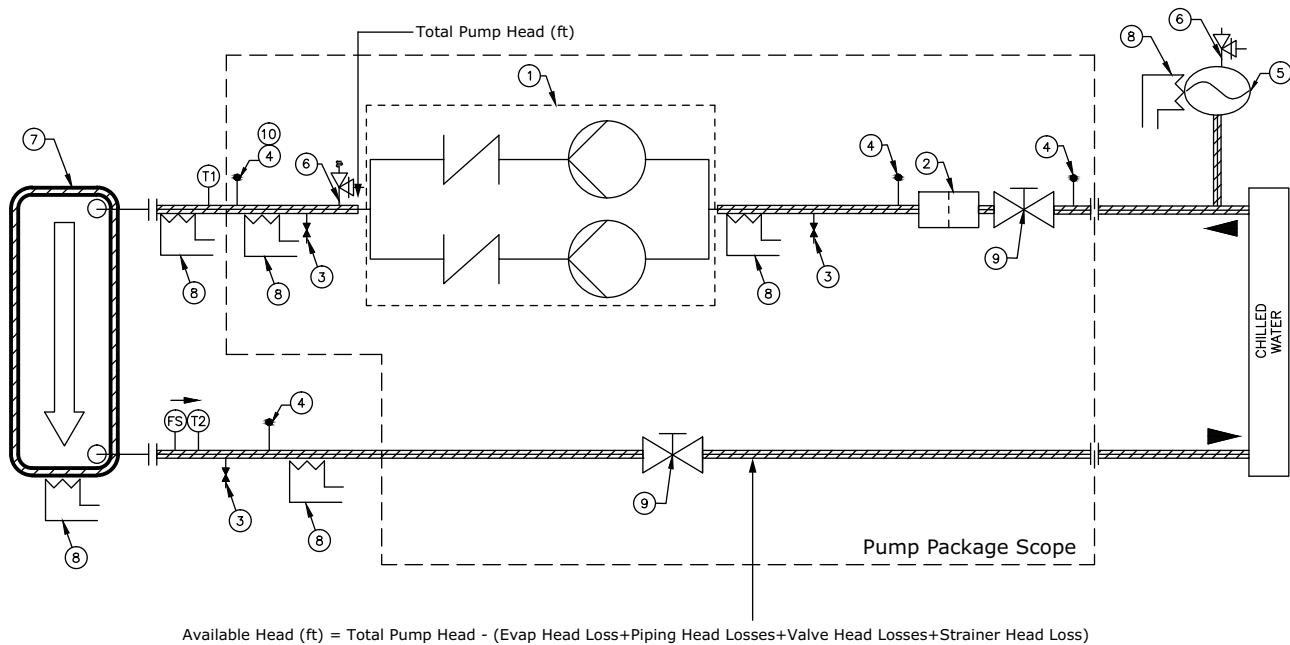
Figure 11. Pump package unit schematic
