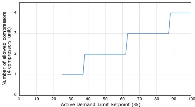
Figure 21. Demand limit setpoint via 4–20 mA signal
