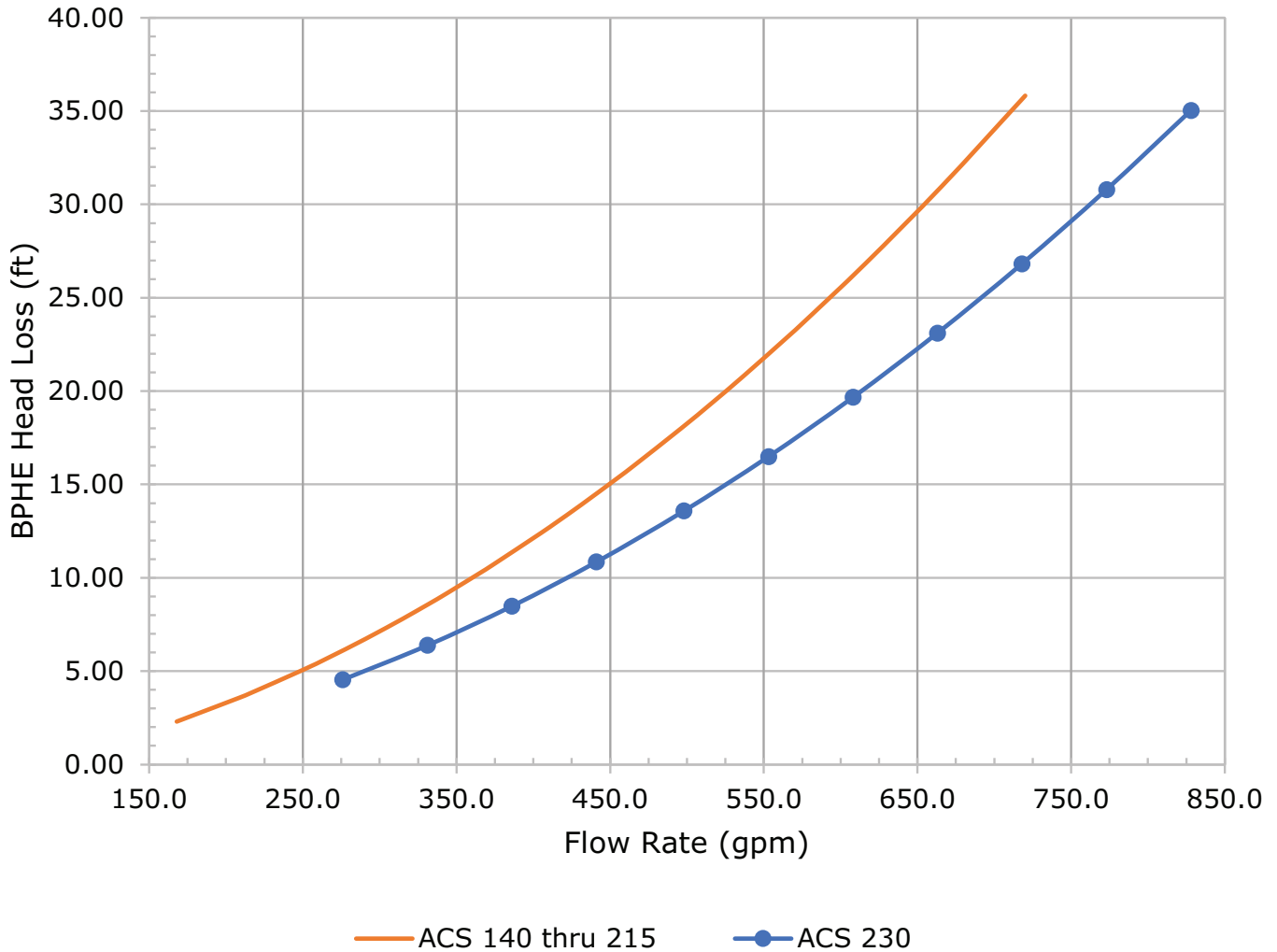
Figure 9. Evaporator head loss
