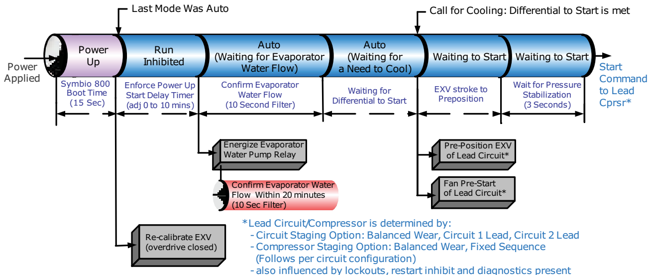
Figure 24. Sequence of operation: power up to starting
