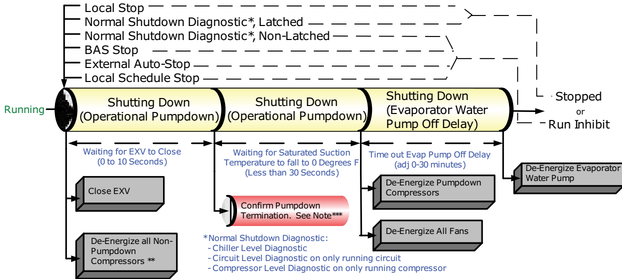
Figure 26. Sequence of operation: normal shutdown to stopped or run inhibit
