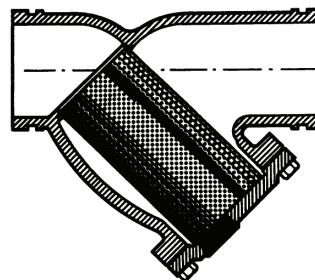
Figure 28. Y-type strainer, units with pump package
