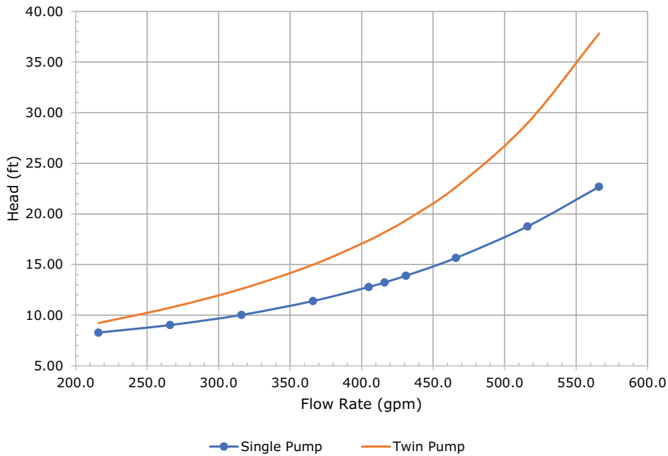
Figure 17. ACS NPSHR water 180-200
