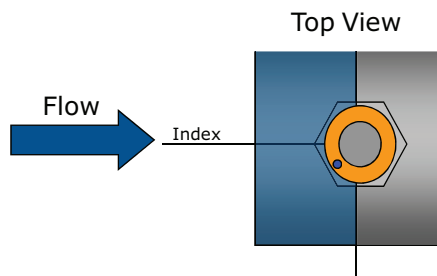
Figure 8. Proper flow switch indexing
