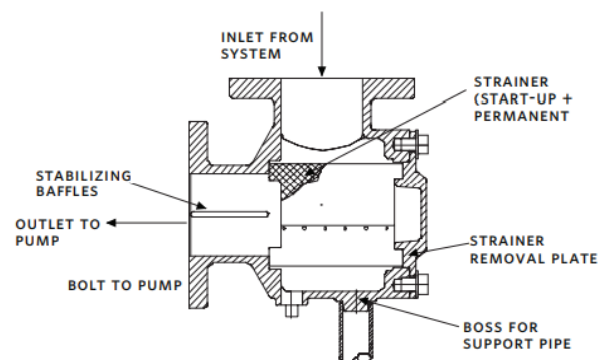
Figure 54. Pump package
