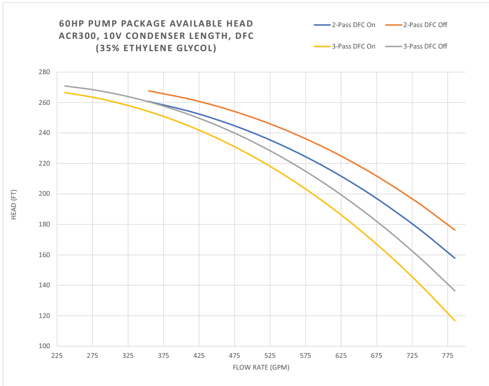
Figure 28. ACR300 – 60hp pump package available head, 10V condenser length
