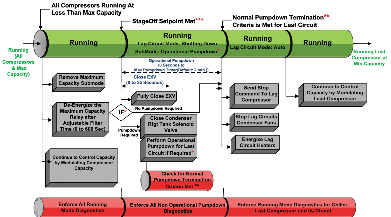
Figure 47. Sequence of events: full load to minimum load
