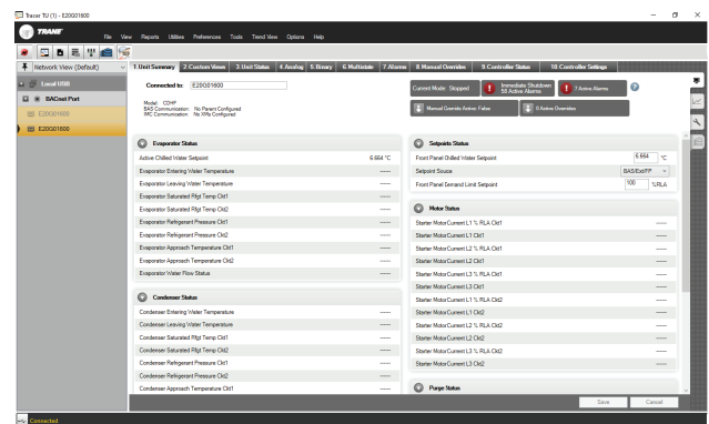
Figure 40. Tracer TU
