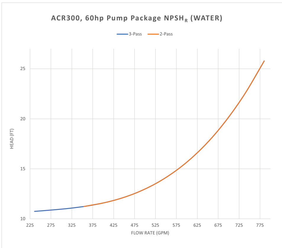
Figure 26. ACR300 –60hp pump package NPSH R (water)
