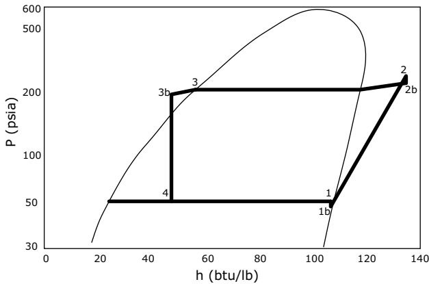
Figure 39. Pressure-enthalpy (P-h) diagram
