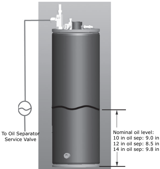
Figure 53. Nominal oil level
