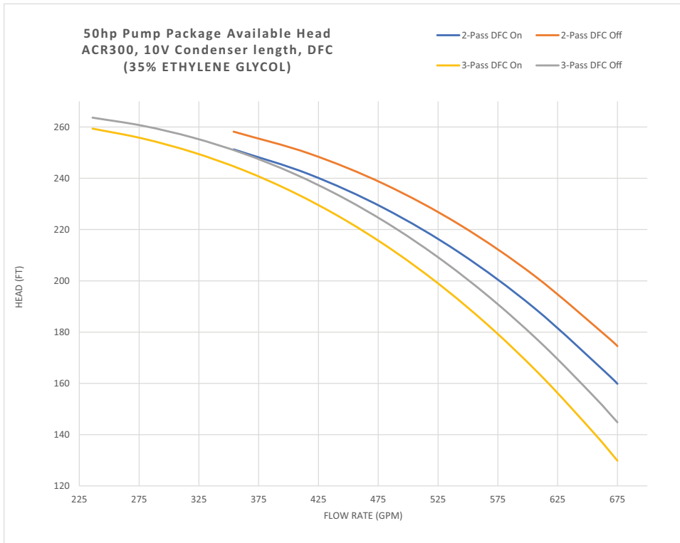
Figure 24. ACR300 – 50hp pump package available head, 10V condenser length
