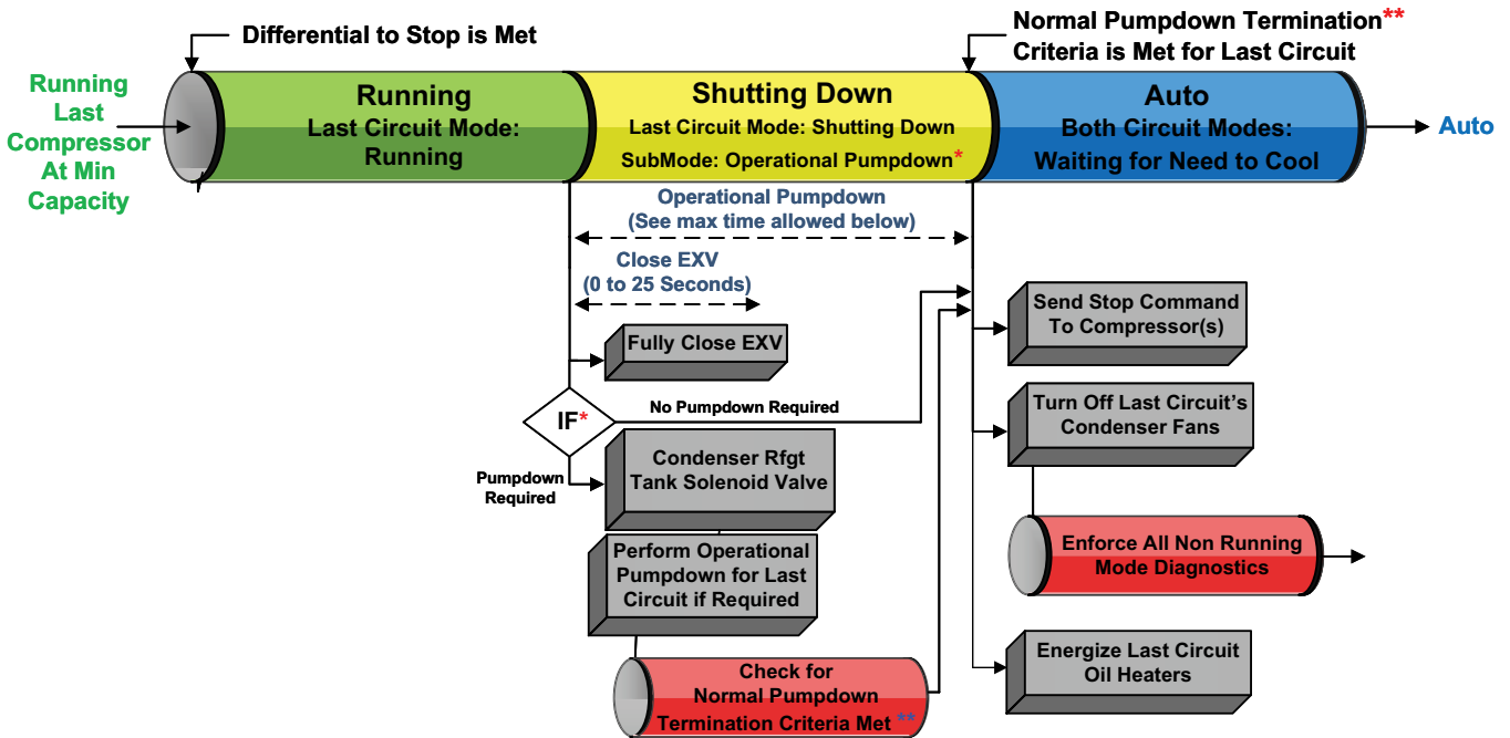
Figure 46. Sequence of events: satisfied setpoint with operational pumpdown
