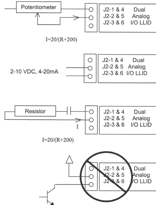
Figure 37. Wiring examples for EDLS and ECWS/EHWS
