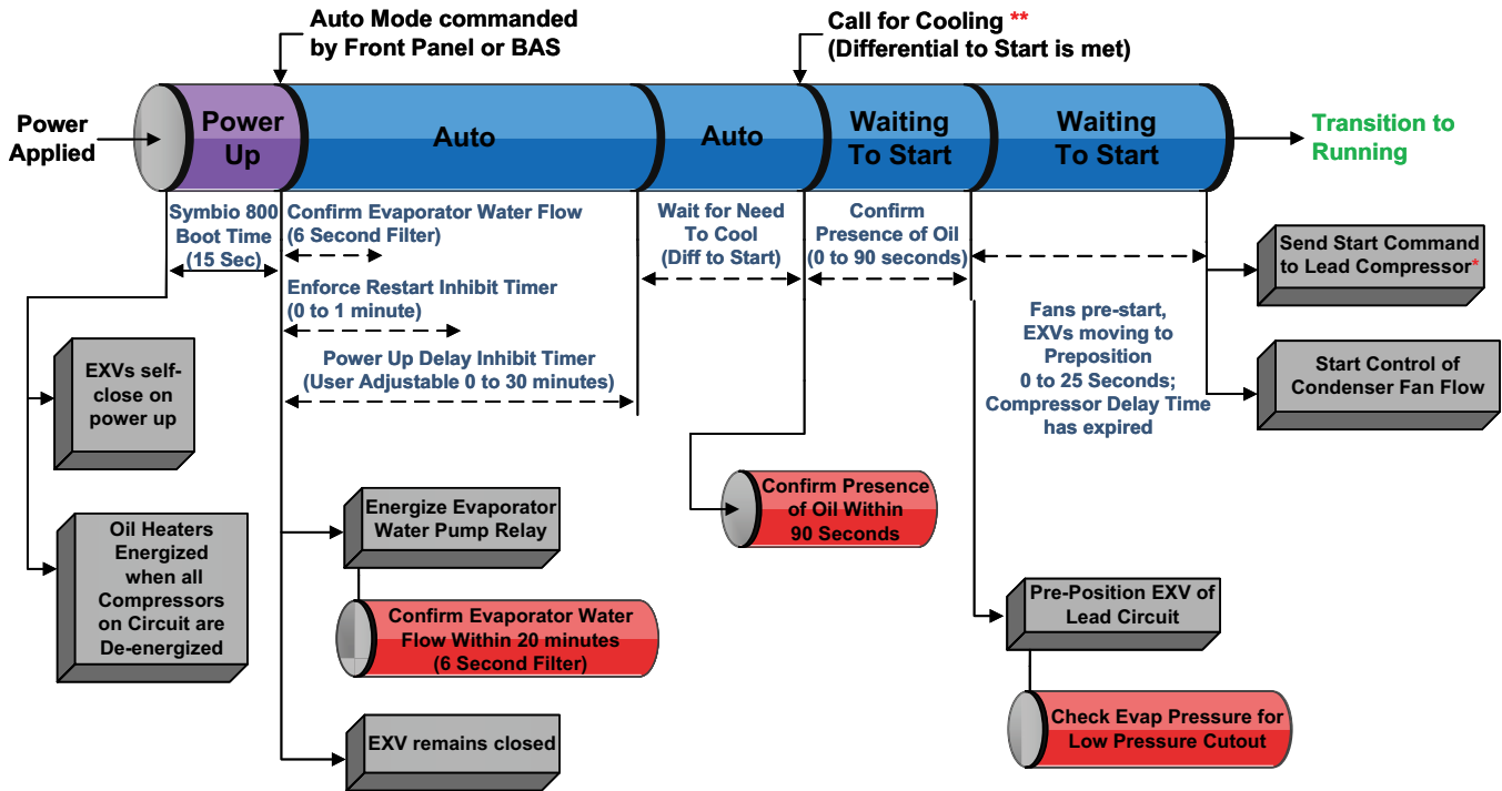
Figure 42. Sequence of events: power up to starting
