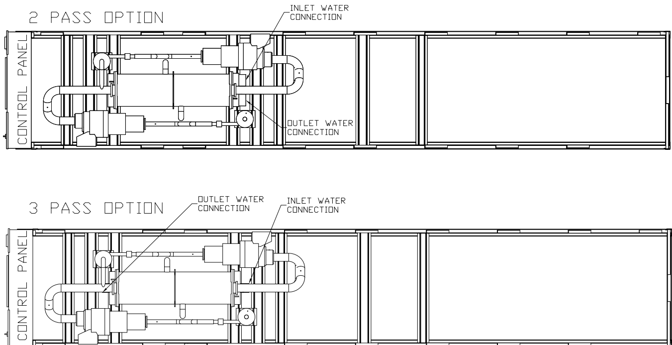
Figure 18. Evaporator pass configurations — two-compressor units
