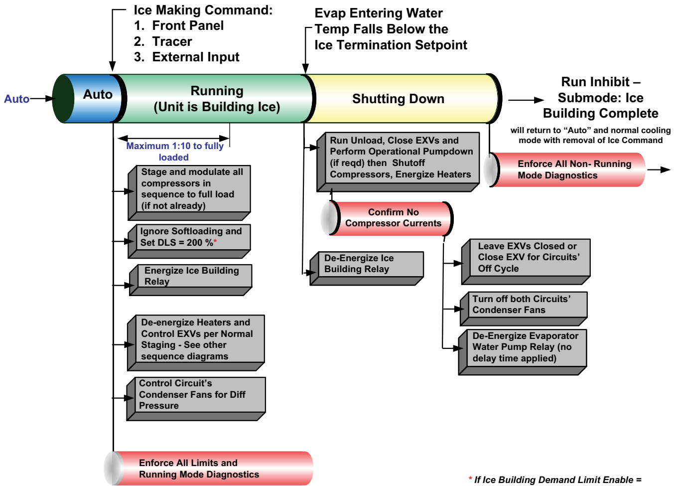
Figure 51. Sequence of events: ice making (stopped to ice to ice making complete)
