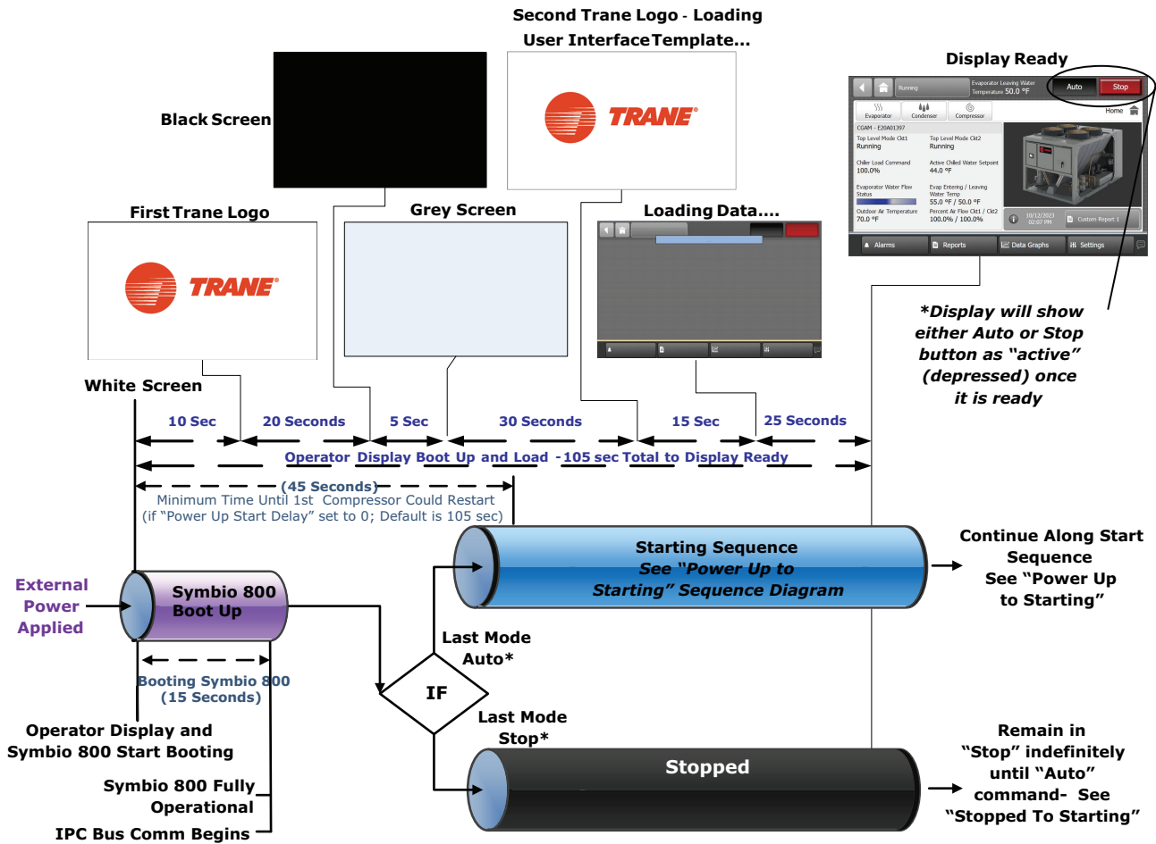
Figure 41. Sequence of operation: power up diagram
