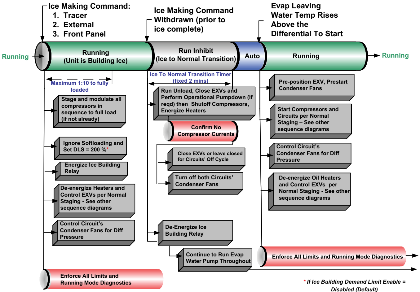
Figure 50. Sequence of events: ice making (running to ice making to running)
