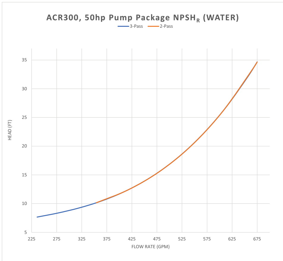
Figure 22. ACR300 – 50hp pump package NPSH R (water)
