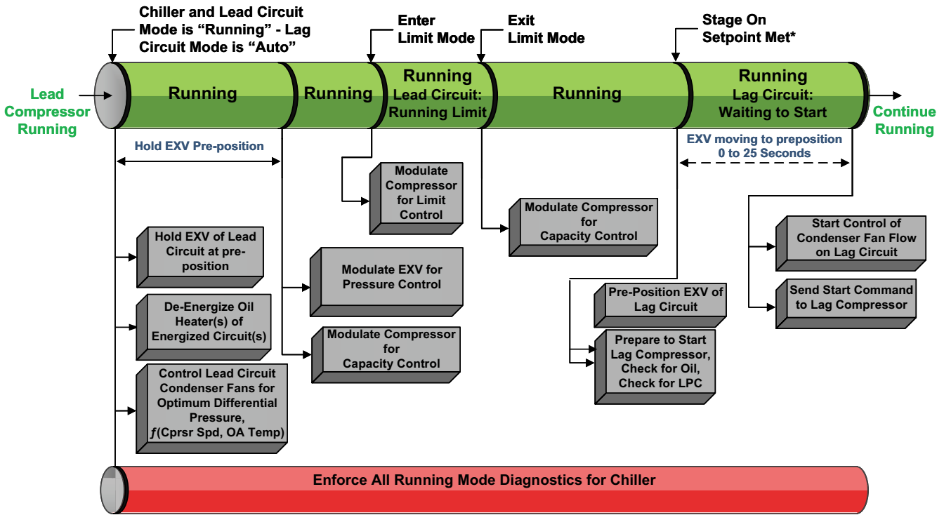
Figure 44. Sequence of events: lead circuit running — increasing load
