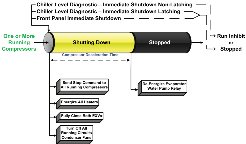
Figure 49. Sequence of events: immediate shutdown to stopped or run inhibit
