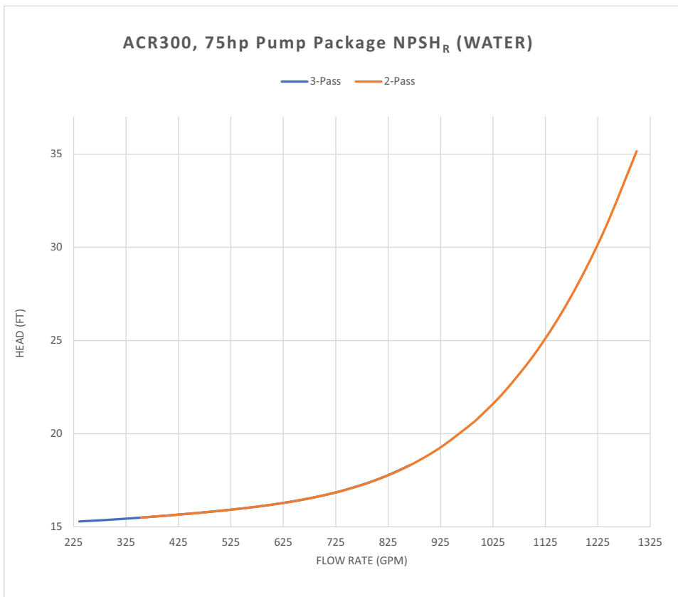
Figure 30. ACR300 – 75hp pump package NPSH R (water)
