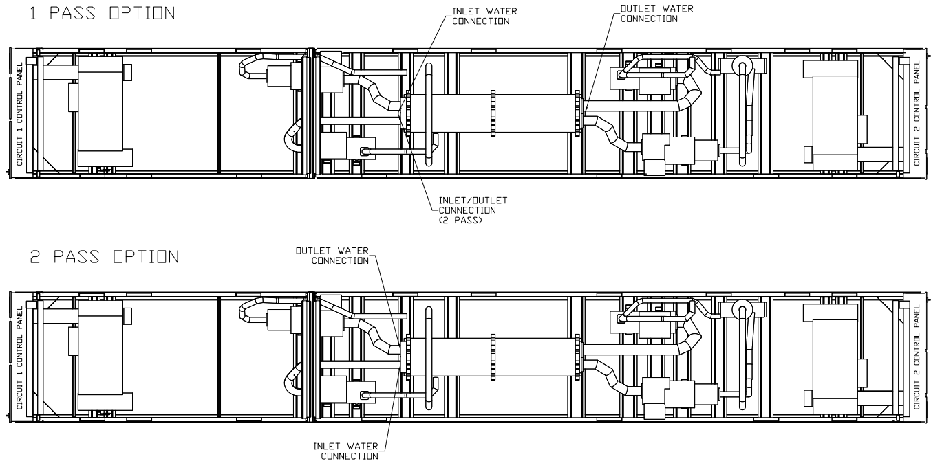
Figure 19. Evaporator pass configurations — three- and four-compressor units
