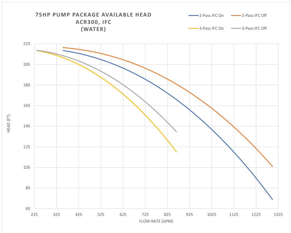
Figure 33. ACR300 – 75hp pump package available head, IFC (water)
