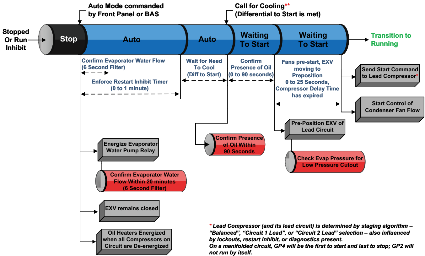
Figure 43. Sequence of events: stopped to starting
