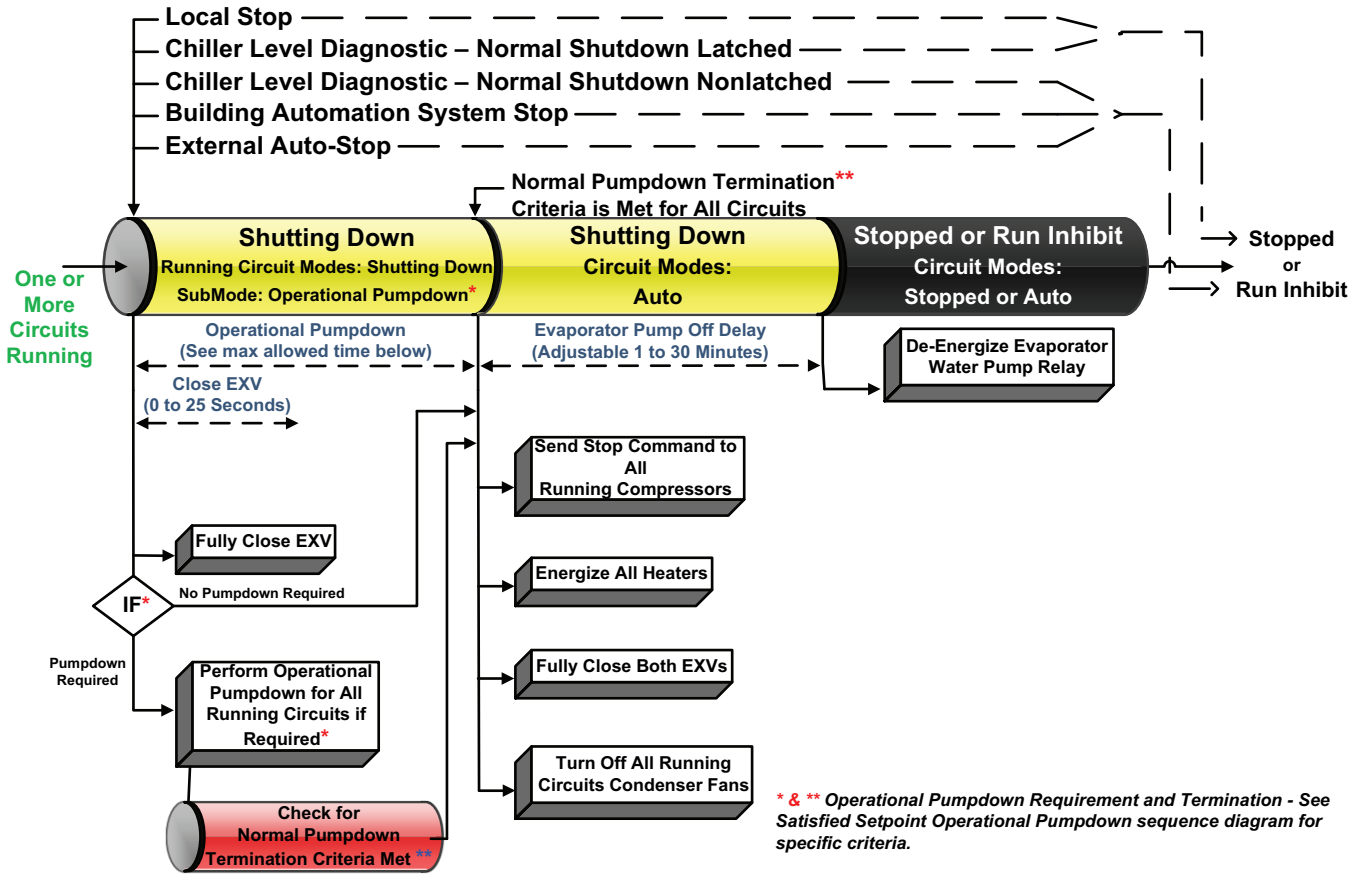
Figure 48. Sequence of events: normal shutdown to stopped or run inhibit
