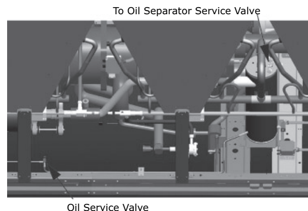
Figure 52. Oil service valves
