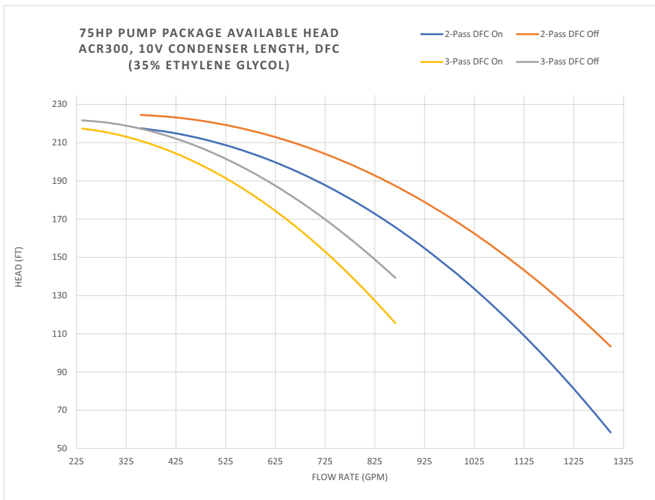
Figure 32. ACR300 – 75hp pump package available head, 10V condenser length
