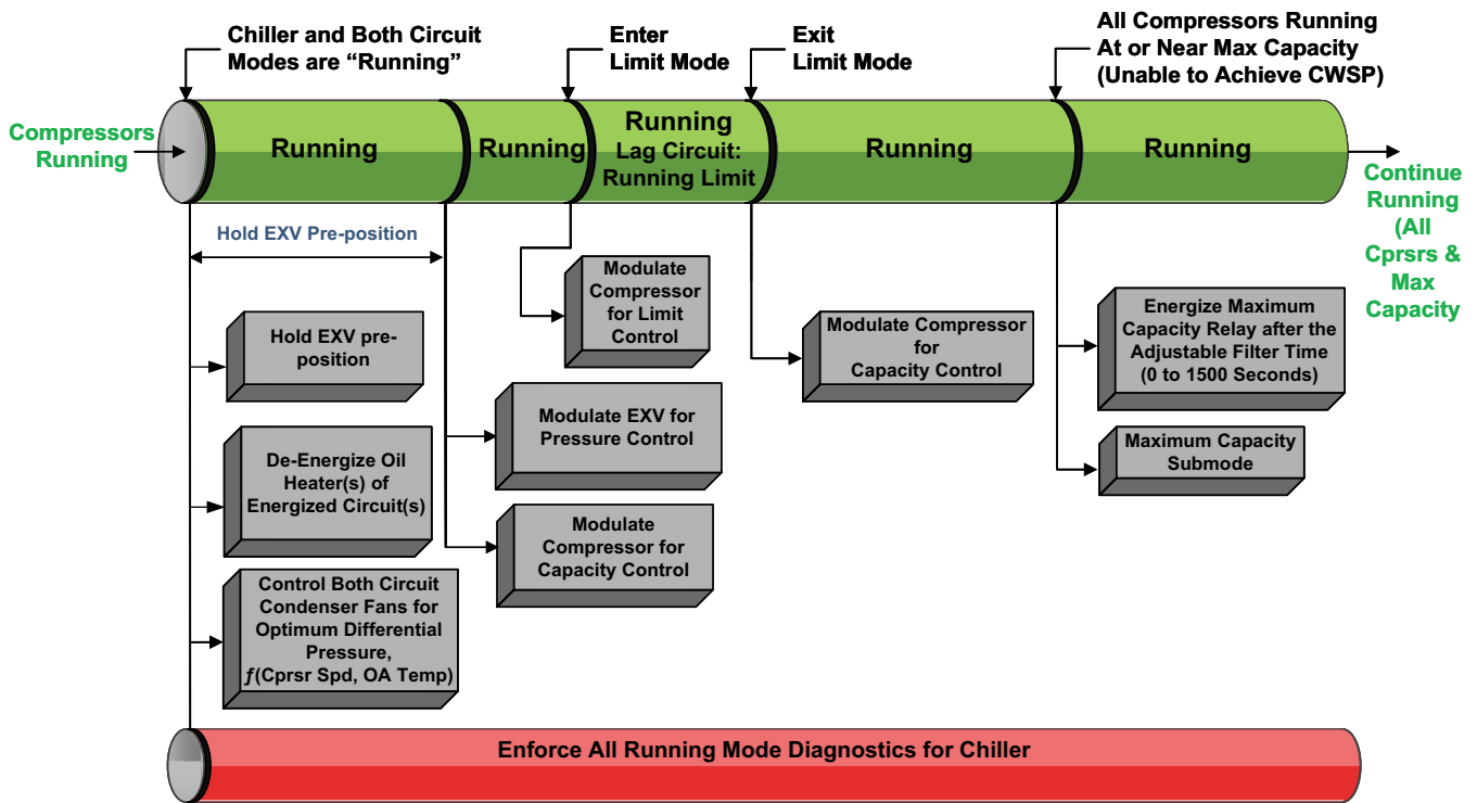
Figure 45. Sequence of operation: lag circuit running — increasing load
