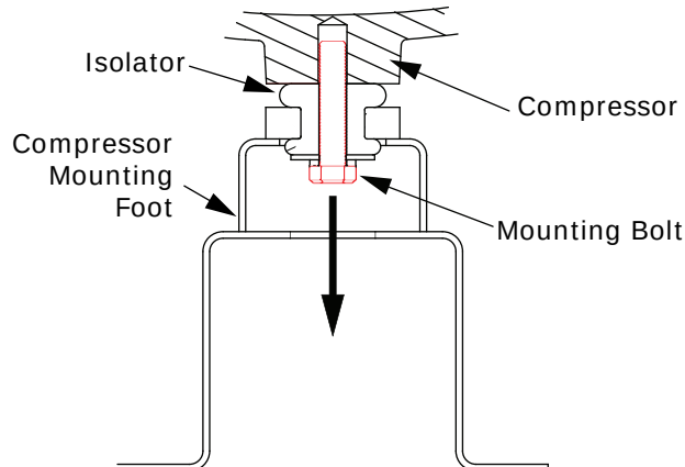
Figure 17. Compressor mounting bolt removal
