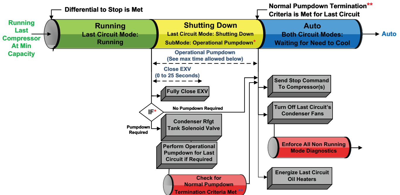
Figure 34. Sequence of events: satisfied setpoint with operational pumpdown
