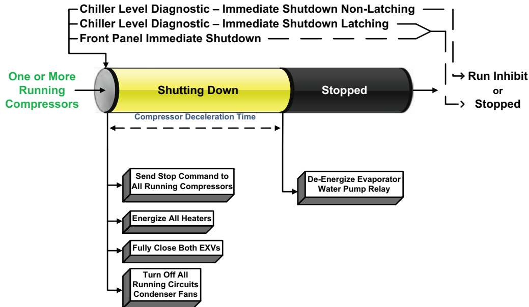
Figure 37. Sequence of events: immediate shutdown to stopped or run inhibit
