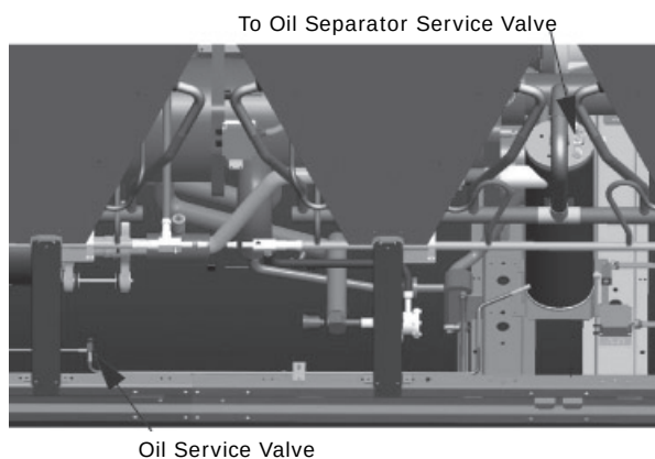
Figure 40. Oil service valves
