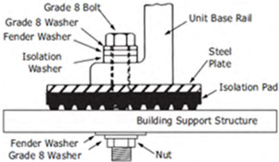
Figure 15. Isolation pad – installed
