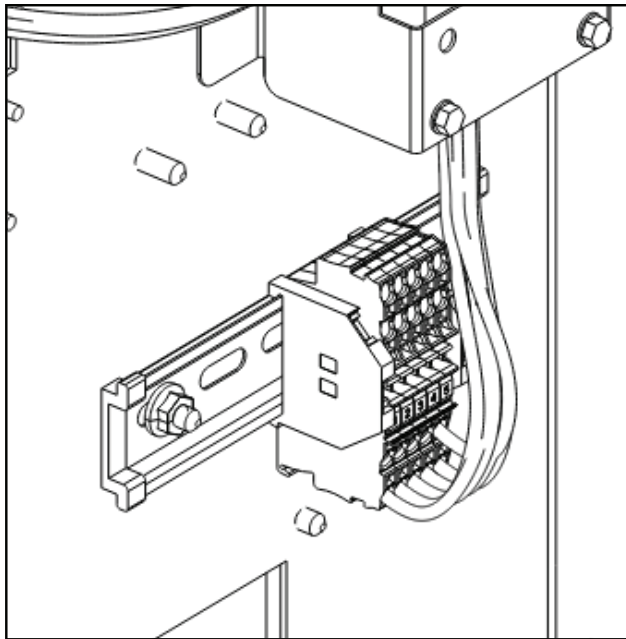
Figure 24. Evaporator heater view
