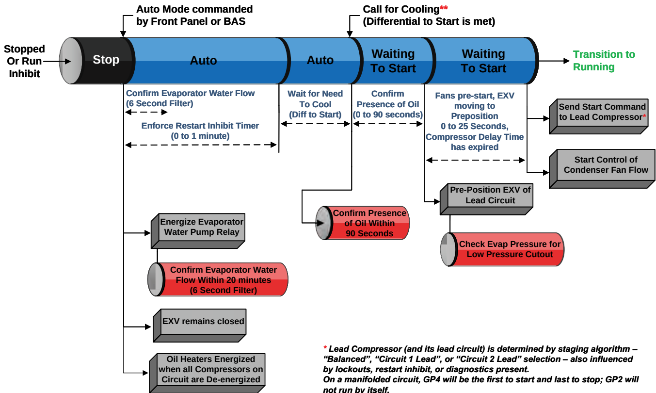
Figure 31. Sequence of events: stopped to starting
