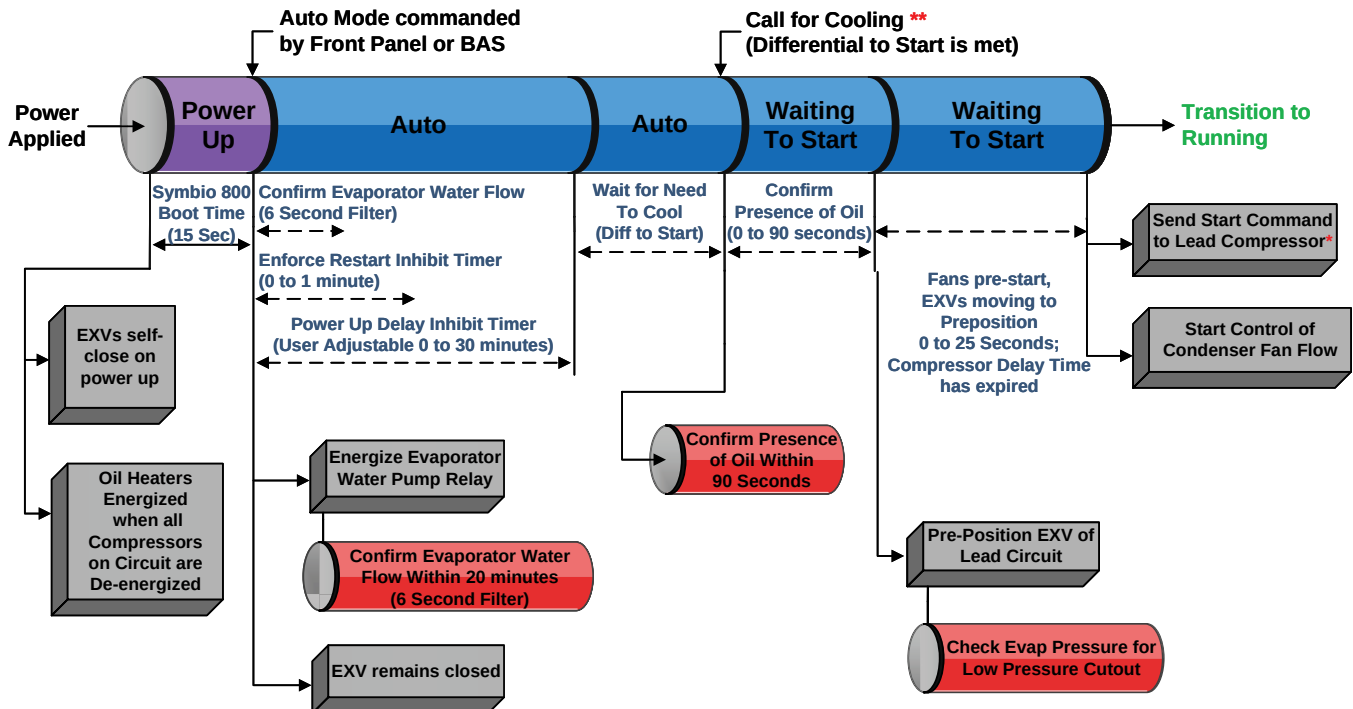
Figure 30. Sequence of events: power up to starting
