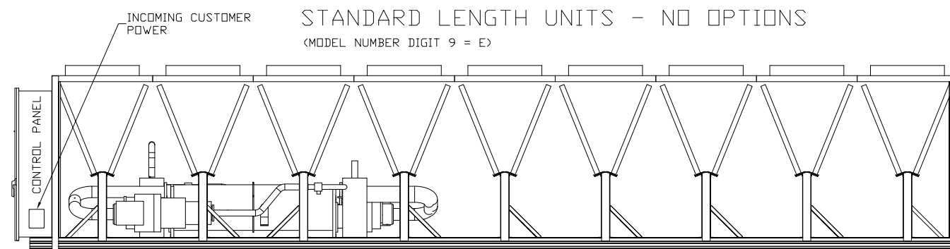
Figure 22. Incoming customer power — control panel (right side view)
