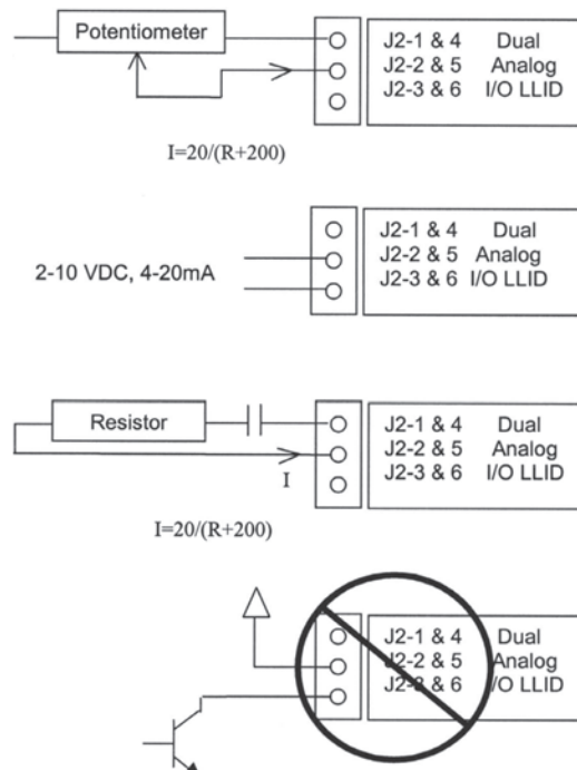
Figure 25. Wiring examples for EDLS and ECWS/EHWS
