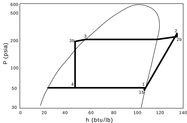
Figure 27. Pressure-enthalpy (P-h) diagram
