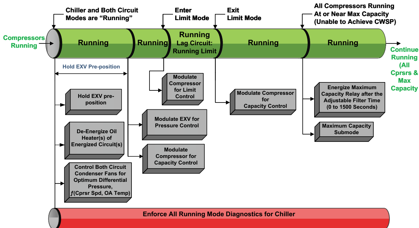
Figure 33. Sequence of operation: lag circuit running — increasing load
