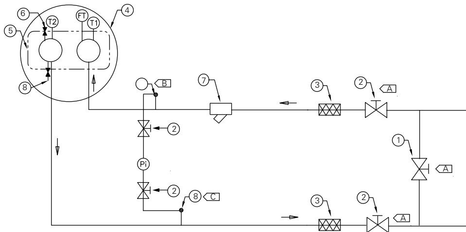
Figure 20. Typical water piping components
