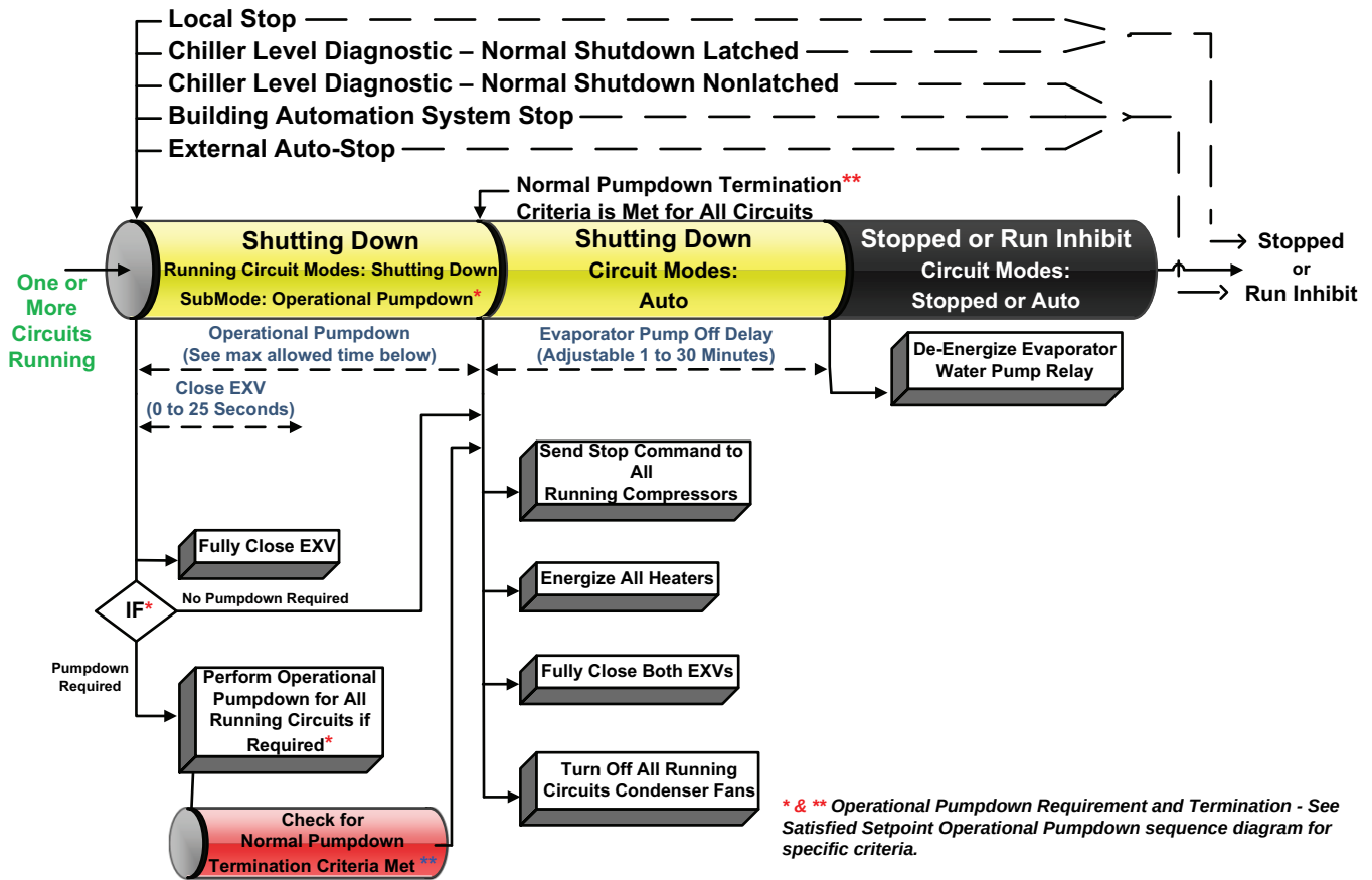
Figure 36. Sequence of events: normal shutdown to stopped or run inhibit
