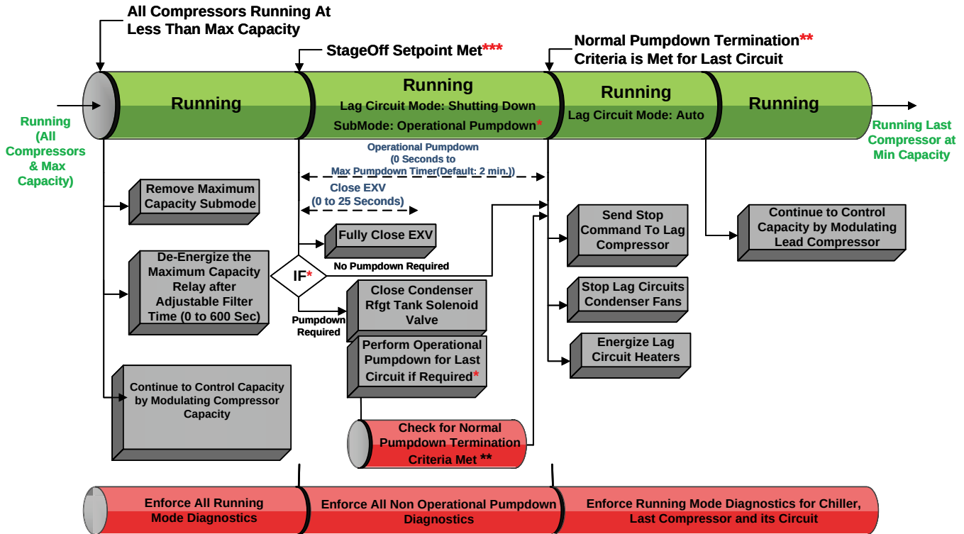
Figure 35. Sequence of events: full load to minimum load
