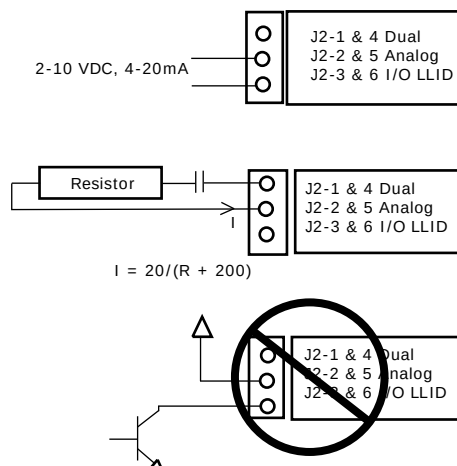
Figure 26. Wiring examples for EDLS and ECWS
