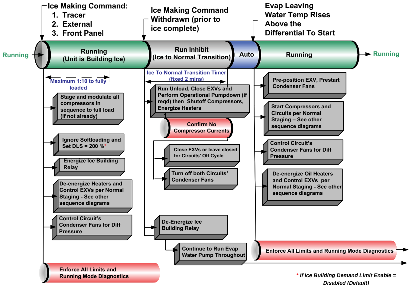
Figure 38. Sequence of events: ice making (running to ice making to running)
