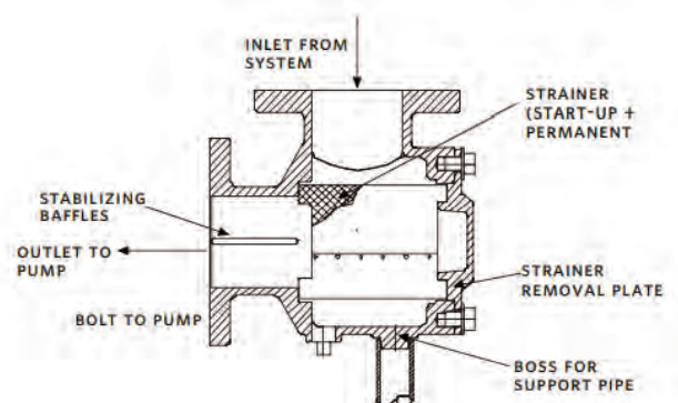
Figure 42. Pump package
