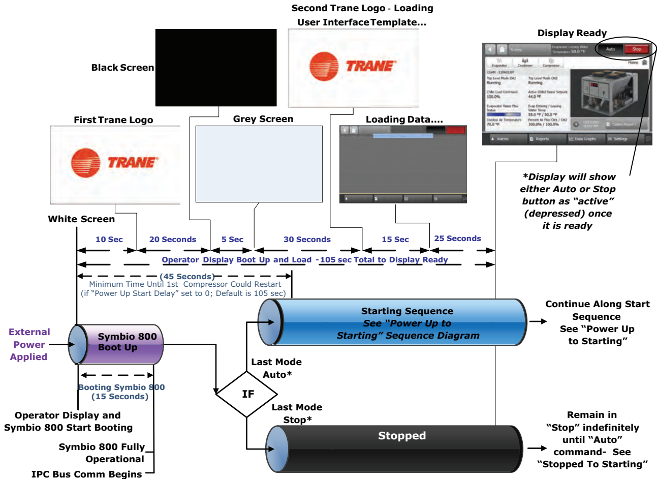
Figure 29. Sequence of operation: power up diagram
