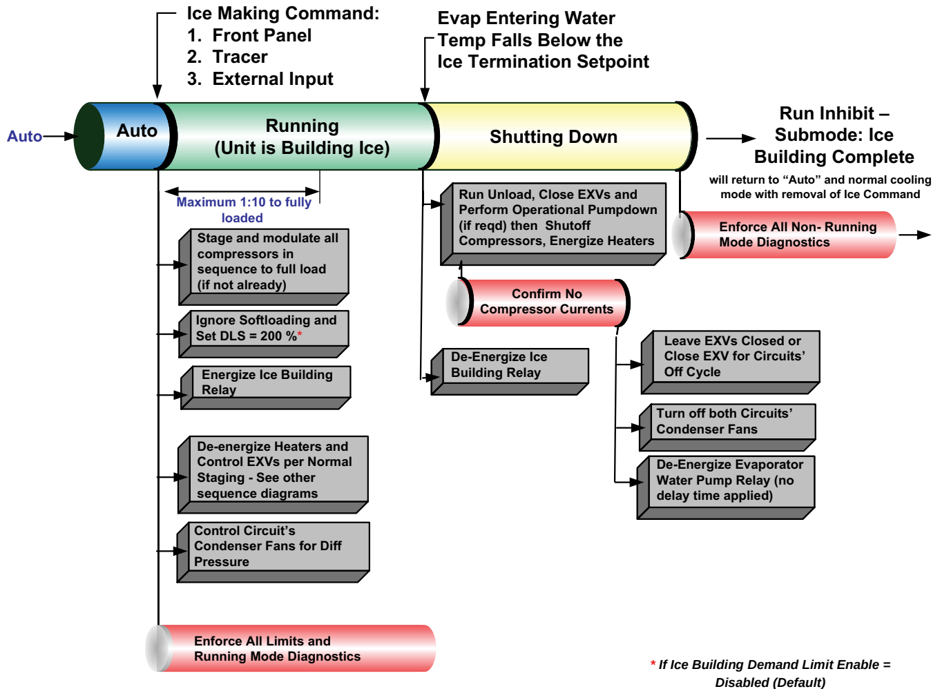
Figure 39. Sequence of events: ice making (stopped to ice to ice making complete)
