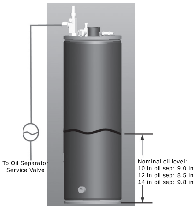
Figure 41. Nominal oil level
