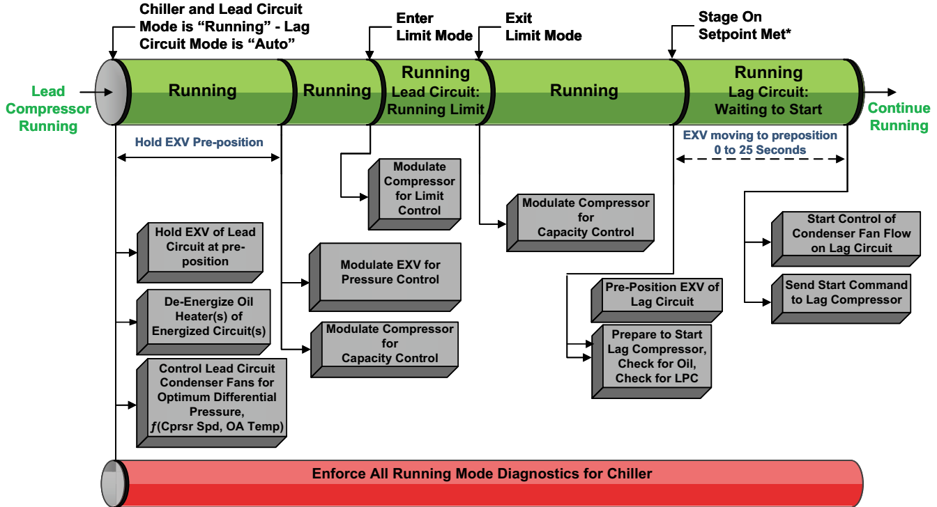
Figure 32. Sequence of events: lead circuit running — increasing load
