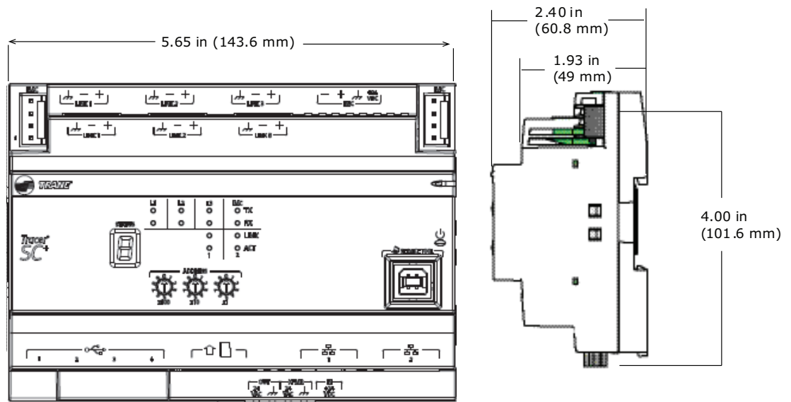
Figure 18. Tracer SC+ system controller dimensions
