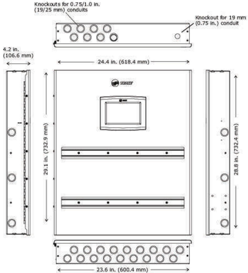
Figure 20. Large enclosure (dimensions)
