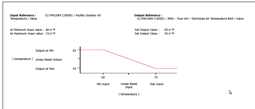
Figure 15. Linear reset example
