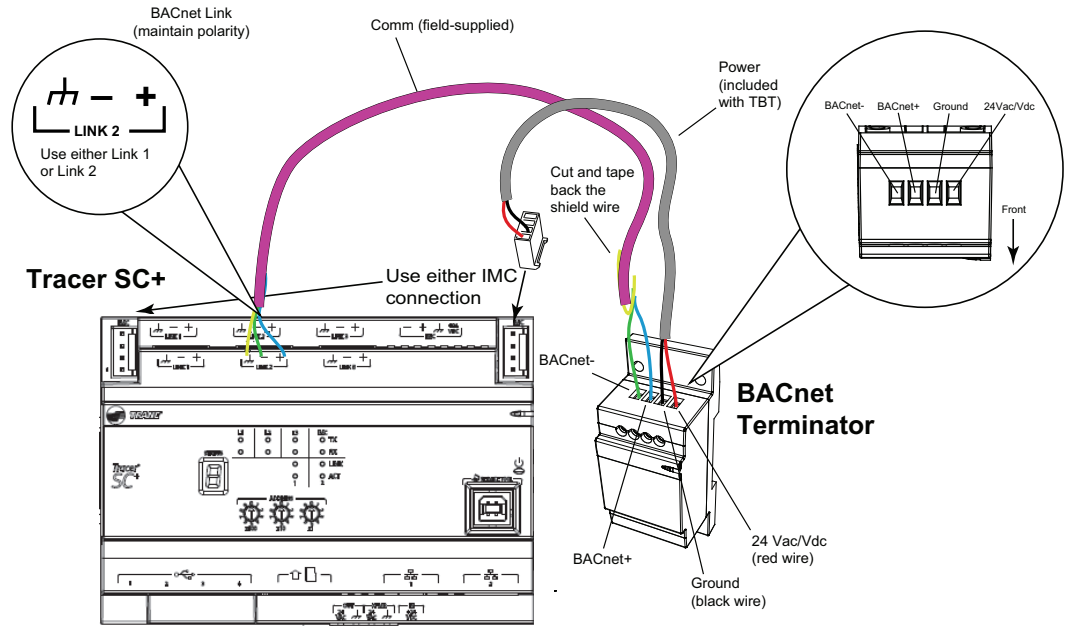
Figure 19. BACnet terminator (wiring)
