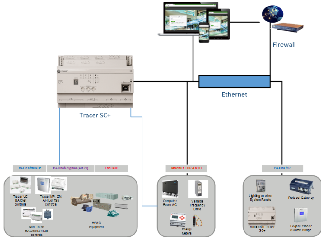
Figure 2. Example of a single SC+ facility configuration
