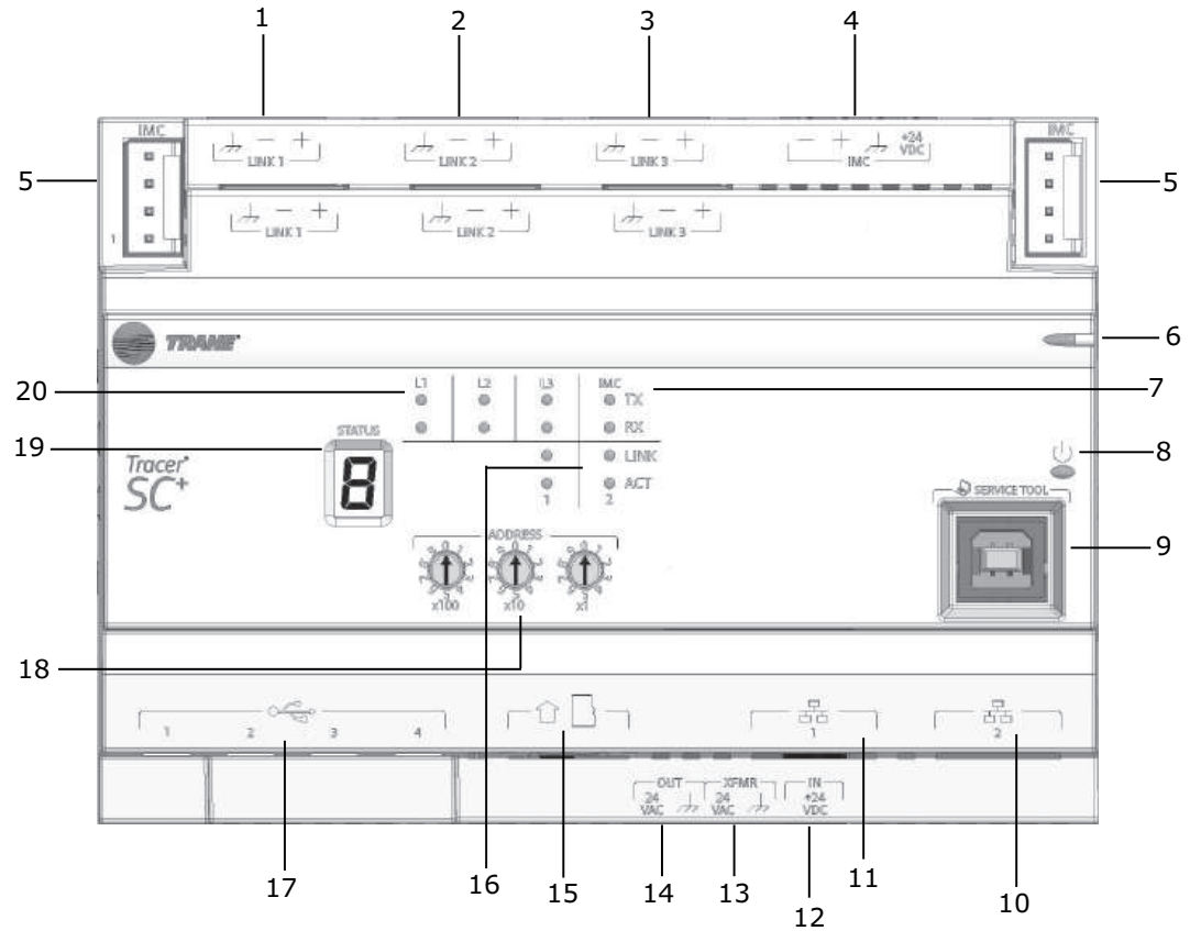
Figure 17. Tracer SC+ components
