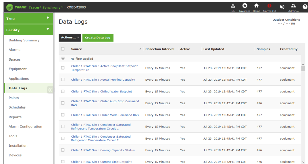
Figure 4. Data logs page
